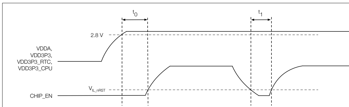
Figure 5: ESP32-C3 Power-up and Reset Timing
