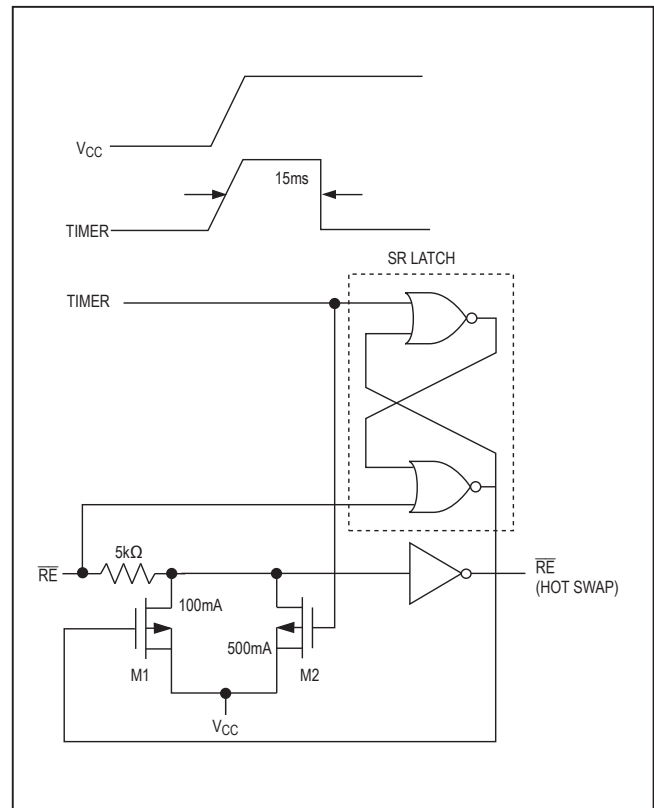
Figure 9. Simplified Structure of the Receiver Enable Pin ( \overline{\text{RE}} )
