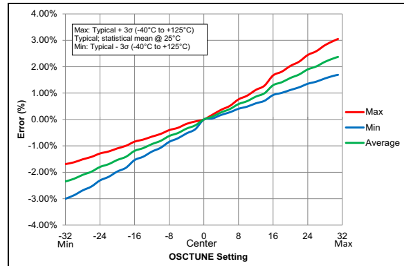
FIGURE 38-105: OSCTUNE Center Frequency, PIC16LF15313/23 Only.
