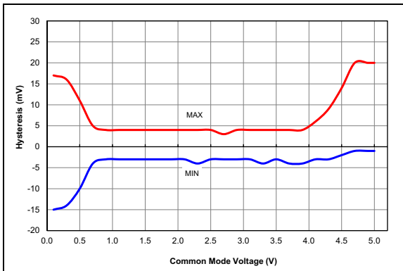
FIGURE 38-81: Comparator Offset, NP Mode (CxSP = 1), VDD = 5.0V, Typical Measured Values at 25°C.
