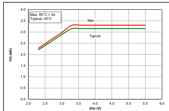
FIGURE 38-6: I_{DD} , HFINTOSC Mode, FOSC = 32 MHz, PIC16F15313/23 Only.
