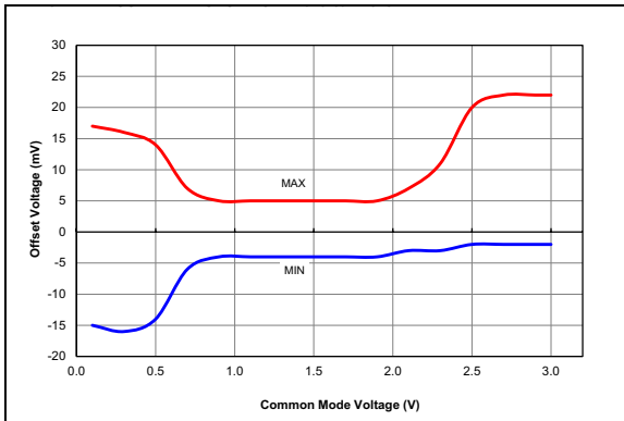
FIGURE 38-79: Comparator Offset, NP Mode (CxSP = 1), VDD = 3.0V, Typical Measured Values from -40°C to 125°C.
