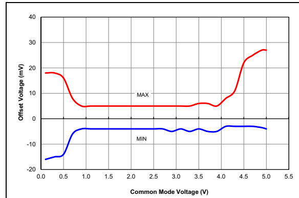
FIGURE 38-82: Comparator Offset, NP Mode (CxSP = 1), VDD = 5.5V, Typical Measured Values from -40°C to 125°C.
