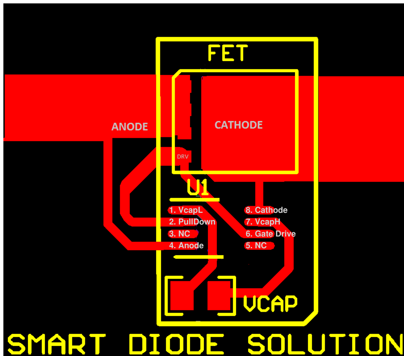
Figure 23. Layout Example
