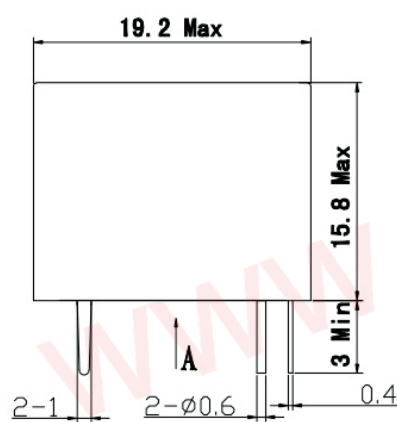
Physical installation diagram
