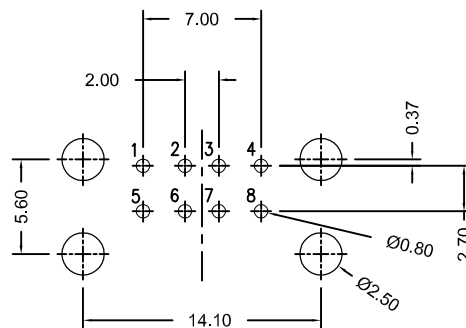
RECOMMENDED P.C.B. LAYOUT TOP VIEW , TOLERANCE ±0.10
