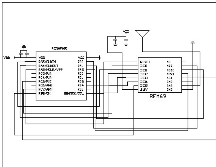
Figure 41. +13dBm Schematic
