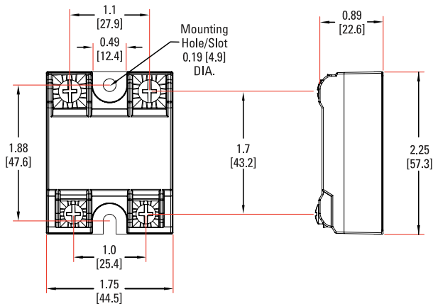
Screw Termination, IP00
