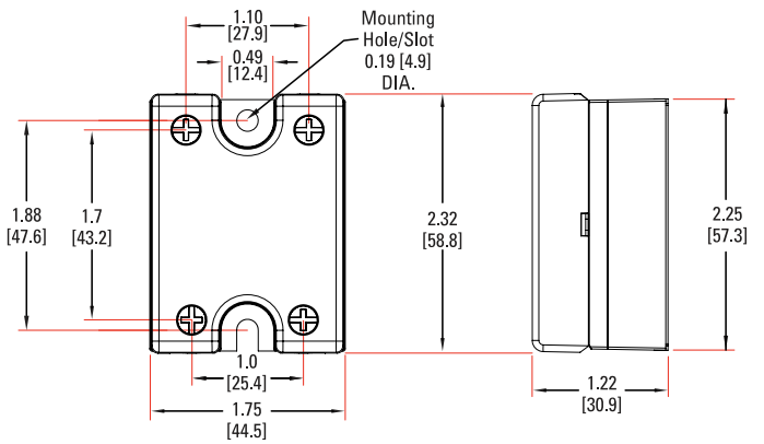
Screw Termination, IP20
