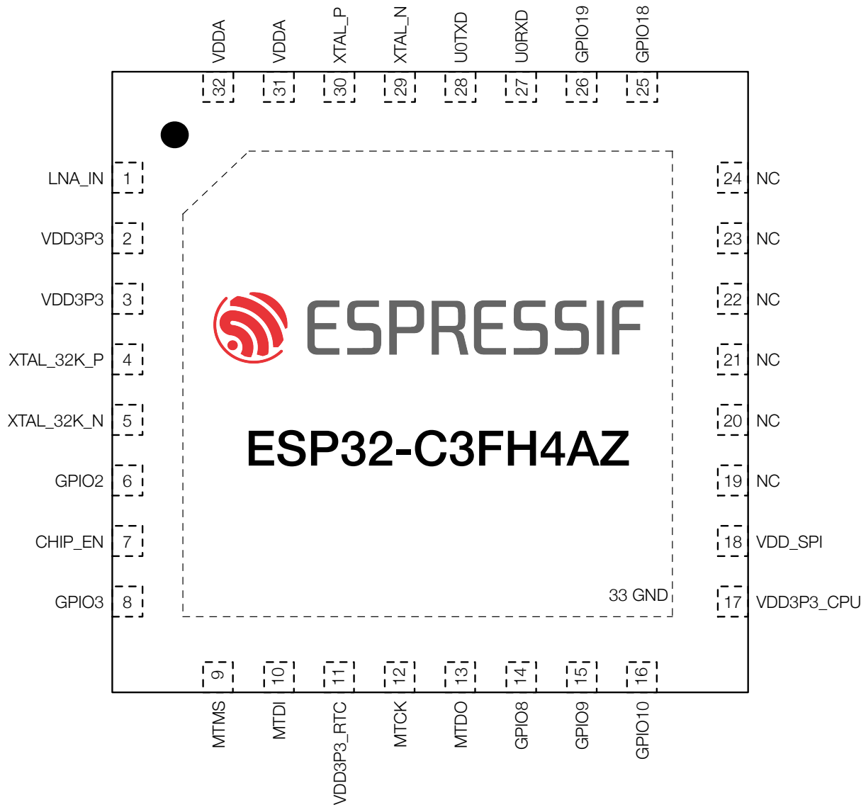
Figure 2-2. ESP32-C3FH4AZ Pin Layout (Top View)
