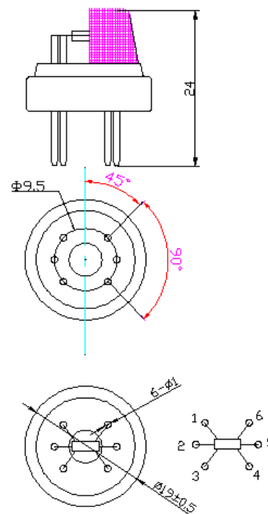
Fig1. Sensor Structure
