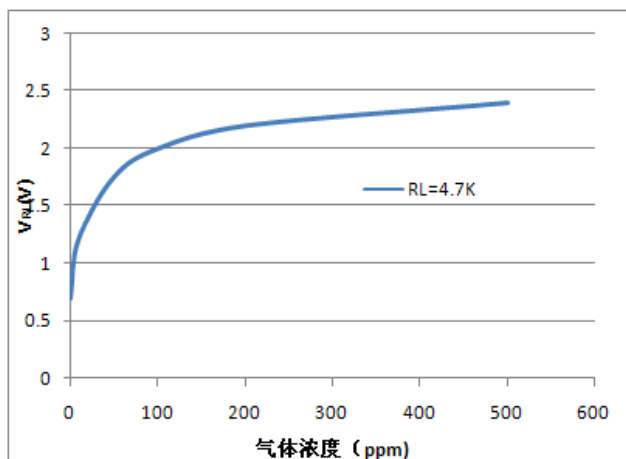
Fig5. Sensitivity Curve
