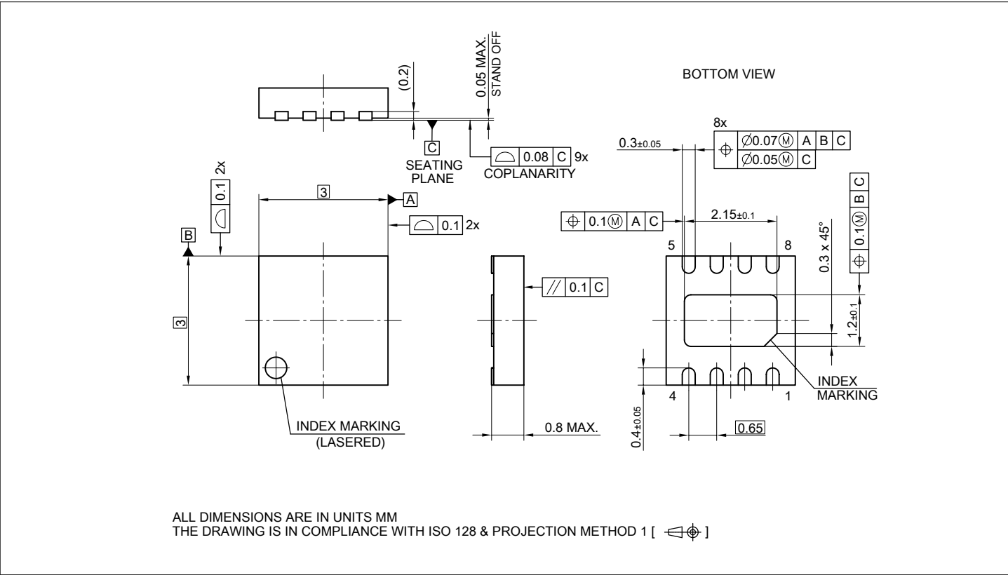
Figure 33 PG-WSO8-8 outline
