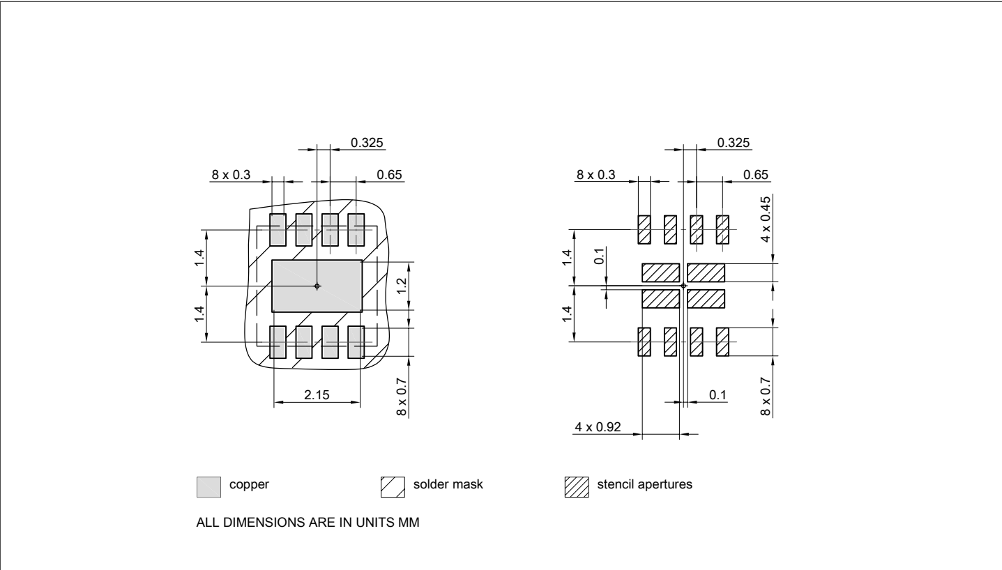
Figure 34 PG-WSO8-8 footprint
