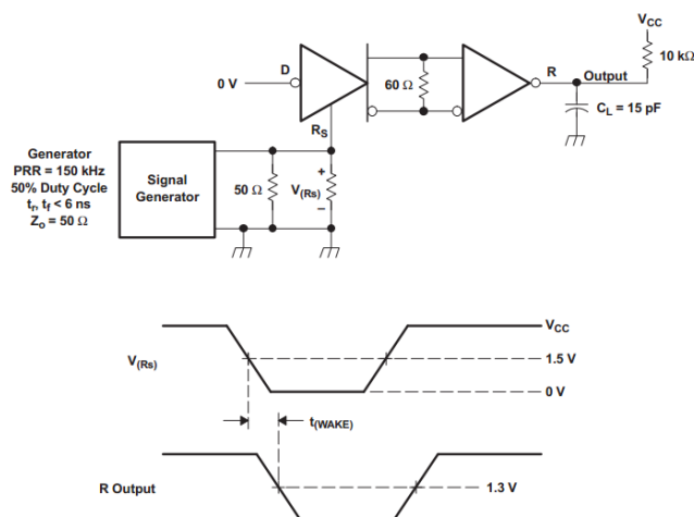
Fig.7 t_{(WAKE)} Test Circuit and Waveform
