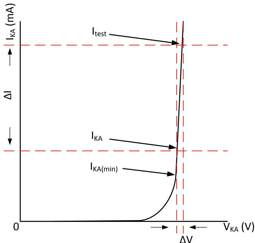
Figure 7-4. Dynamic Impedance
