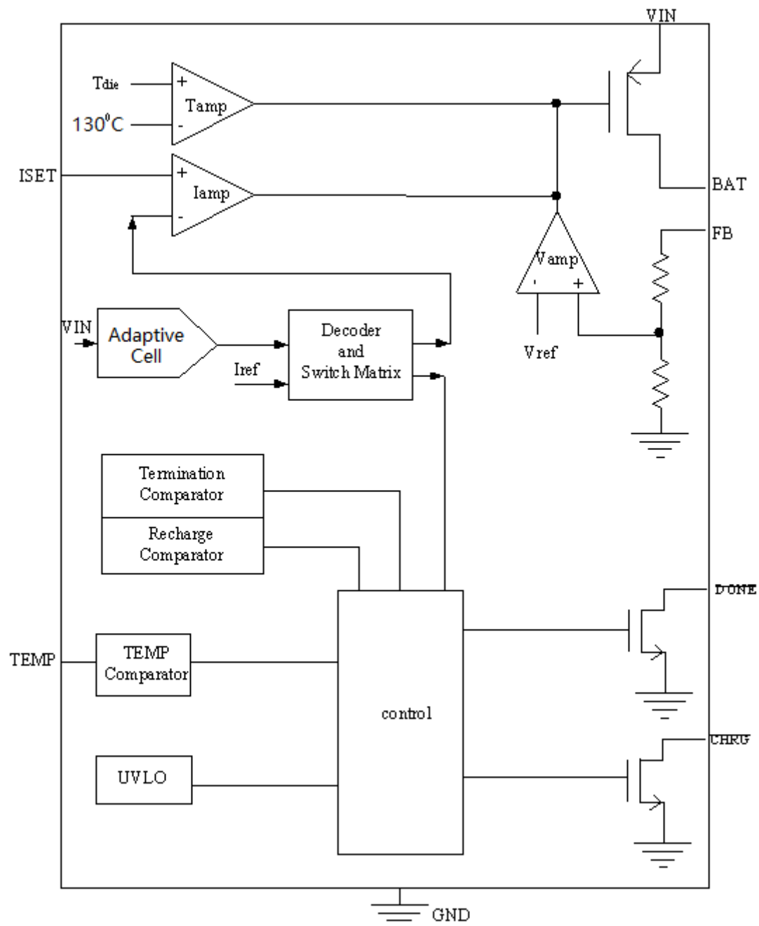
Figure 3 Block Diagram
