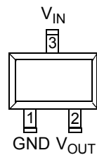
3-Pin SOT-23
