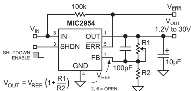
MIC2954 ADJUSTABLE REGULATOR
