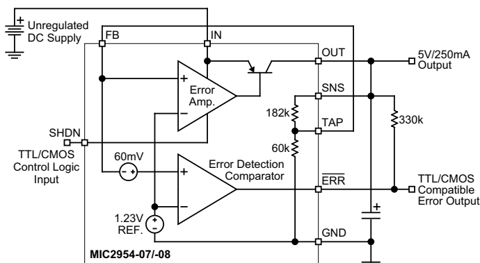
MIC2954-07 and MIC2954-08
