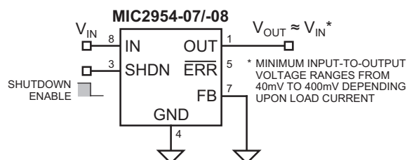
MIC2954 WIDE INPUT VOLTAGE RANGE CURRENT LIMITER
