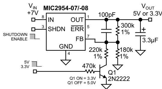
MIC2954 5V OR 3V SELECTABLE REGULATOR WITH SHUTDOWN
