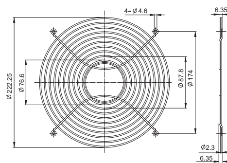
FG-25 For 254mm Fan
