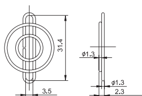
FG-02 For 25mm Fan
