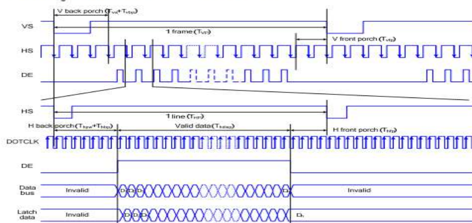
Figure 28 Timing Chart of Signals in RGB Interface DE Mode
