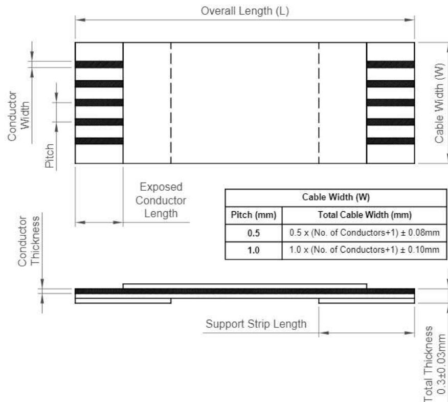
Cable Type A - Conductor Same Side
