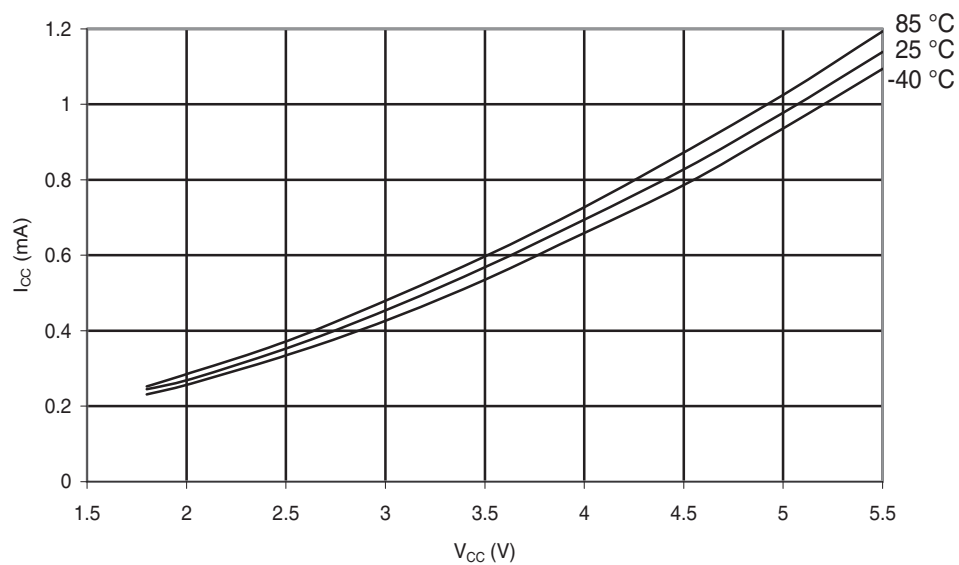
Figure 30-57. ATmega48PA: Idle Supply Current vs. V_{CC} (Internal RC Oscillator, 8MHz)
