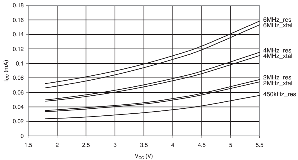
Figure 30-155. ATmega88PA: Standby Supply Current vs. V_{CC} (Watchdog Timer Disabled)
