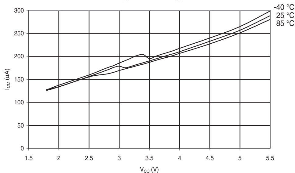
Figure 30-181. ATmega88PA: ADC Current vs. V_{CC} (AREF = AV_{CC} )
