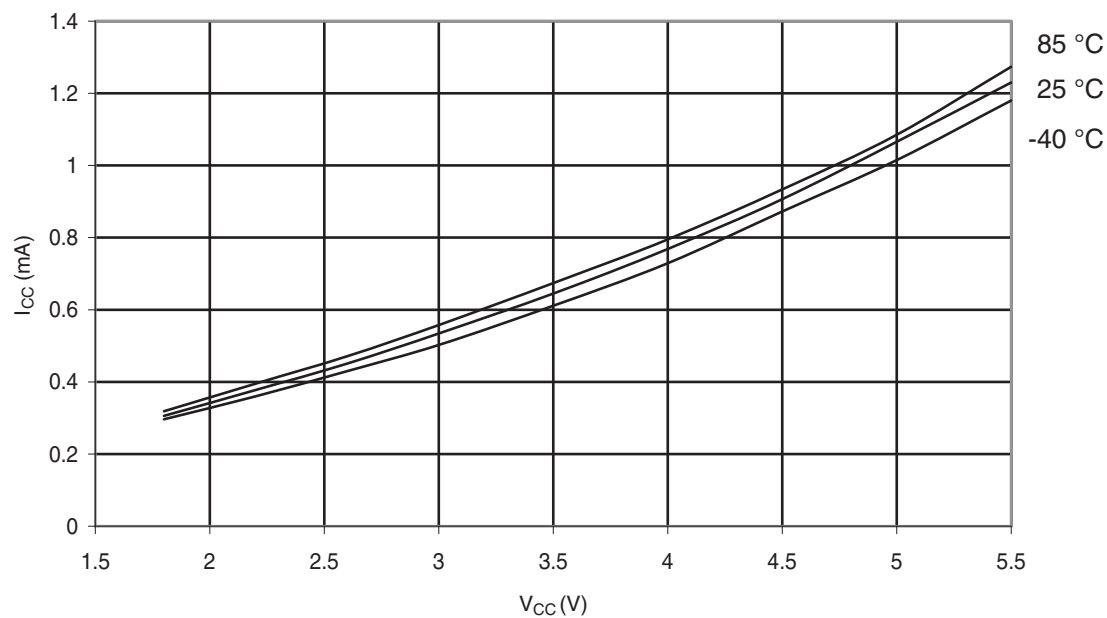
Figure 30-286. ATmega328: Active Supply Current vs. V_{CC} (Internal RC Oscillator, 1MHz)
