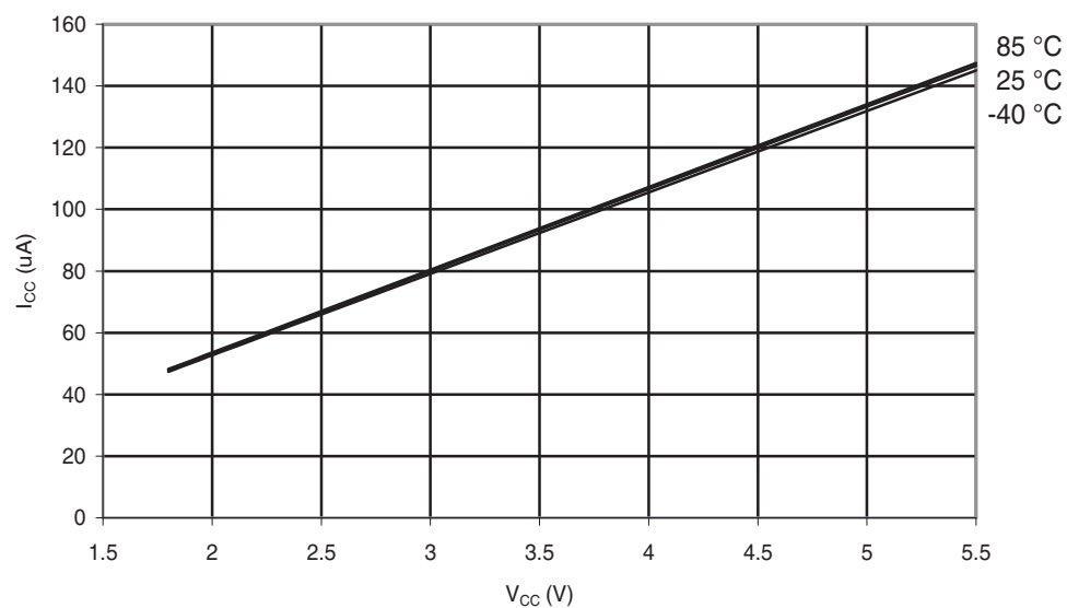
Figure 30-89. ATmega48PA: AREF External Reference Current vs. V_{CC}
