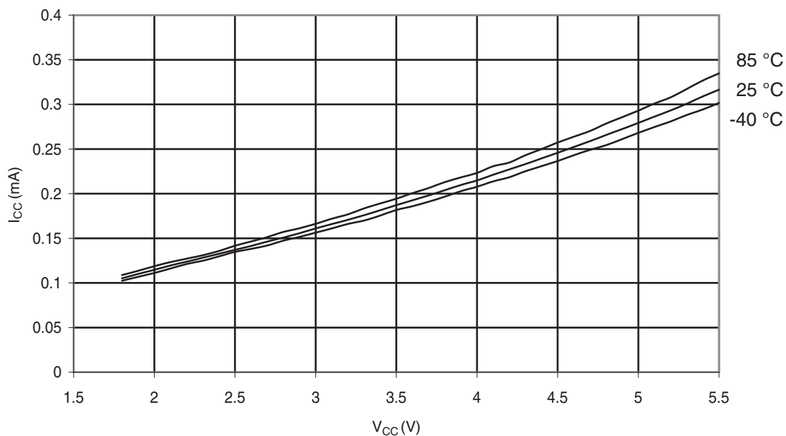
Figure 30-338. ATmega328P: Idle Supply Current vs. V_{CC} (Internal RC Oscillator, 1MHz)
