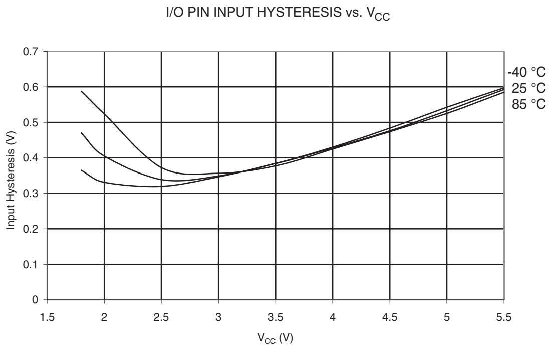
Figure 30-309. ATmega328: I/O Pin Input Hysteresis vs. V_{CC}
