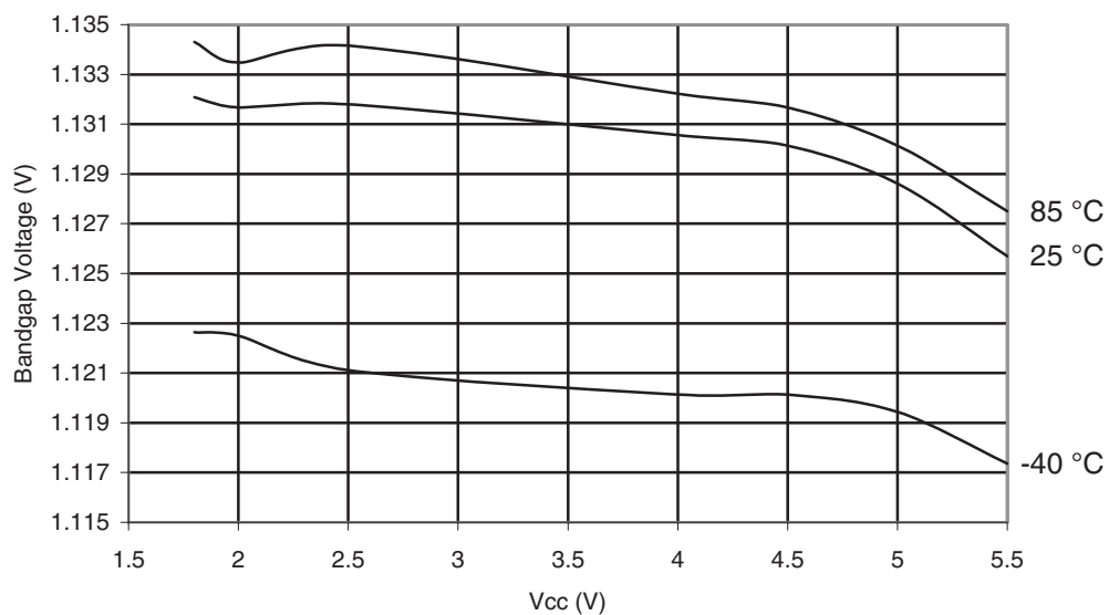
Figure 30-269. ATmega168PA: Bandgap Voltage vs. V_{CC}
