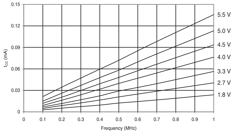
Figure 30-241. ATmega168PA: Idle Supply Current vs. Low Frequency (0.1-1.0MHz)
