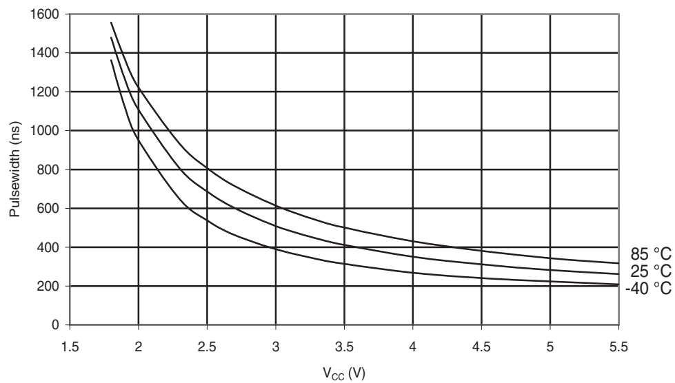
Figure 30-47. ATmega48A: Minimum Reset Pulse width vs. V_{CC}
