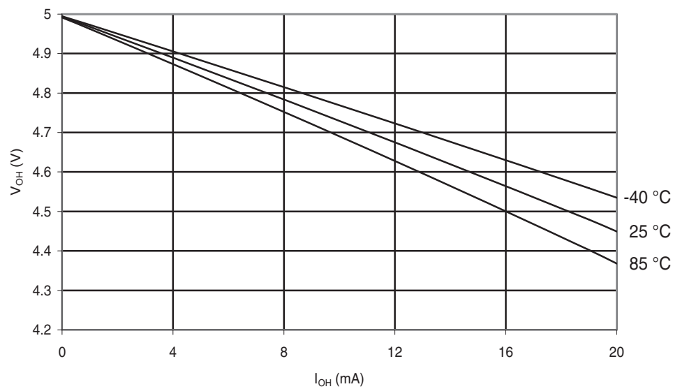
Figure 30-71. ATmega48PA: I/O Pin Output Voltage vs. Source Current ( V_{CC} = 5\text{ V} )
