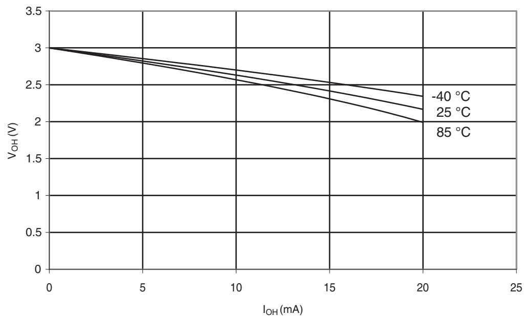
Figure 30-305. ATmega328: I/O Pin Output Voltage vs. Source Current ( V_{CC} = 3\text{ V} )
