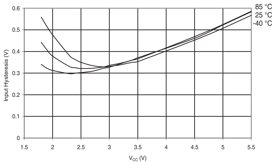
Figure 30-262. ATmega168PA: I/O Pin Input Hysteresis vs. V_{CC}
