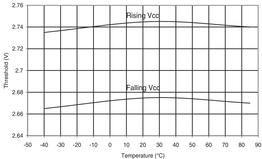
Figure 30-126.ATmega88A: BOD Thresholds vs. Temperature (BODLEVEL is 2.7 V)
