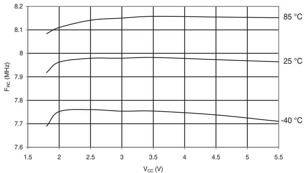
Figure 30-84. ATmega48PA: Calibrated 8MHz RC Oscillator Frequency vs. V_{CC}
