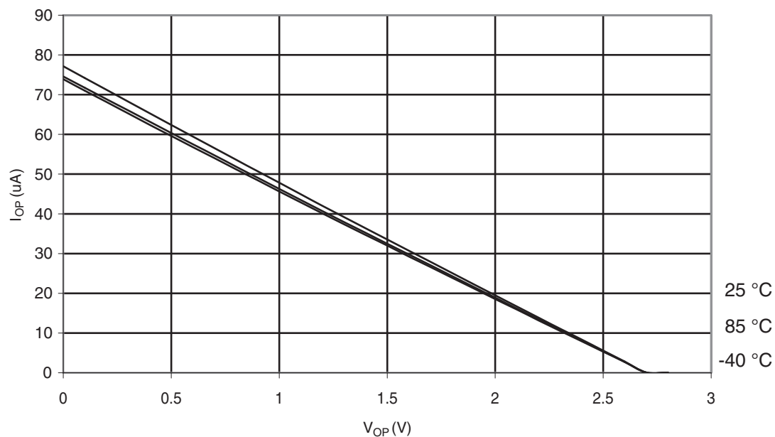
Figure 30-298. ATmega328: I/O Pin Pull-up Resistor Current vs. Input Voltage ( V_{CC} = 2.7\text{ V} )
