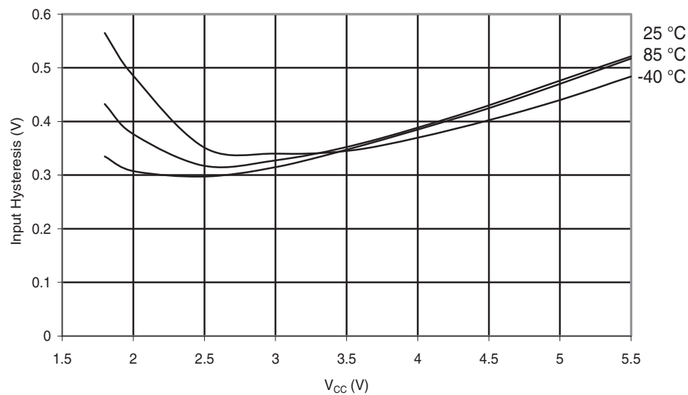
Figure 30-121. ATmega88A: I/O Pin Input Hysteresis vs. V_{CC}
