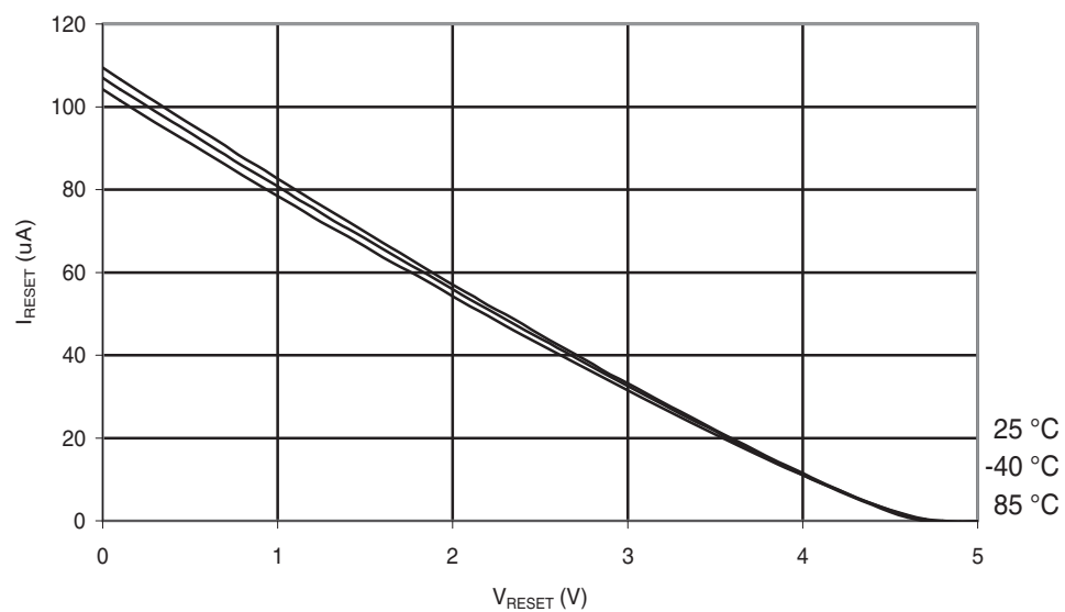
Figure 30-208. ATmega168A: Reset Pull-up Resistor Current vs. Reset Pin Voltage ( V_{CC} = 5\text{ V} )
