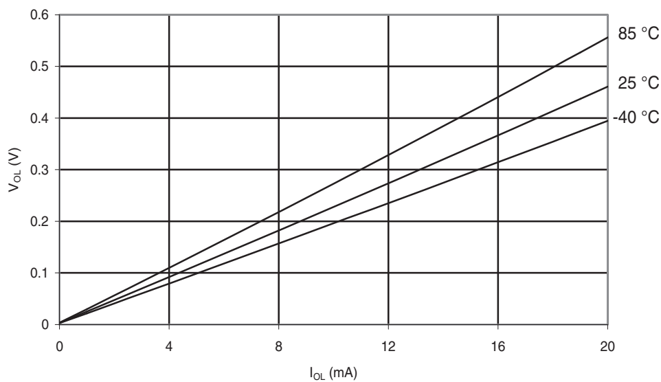
Figure 30-210. ATmega168A: I/O Pin Output Voltage vs. Sink Current ( V_{CC} = 5\text{ V} )
