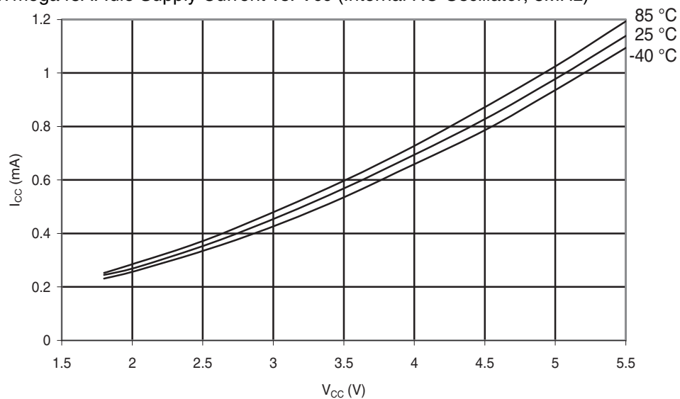
Figure 30-10. ATmega48A: Idle Supply Current vs. V_{CC} (Internal RC Oscillator, 8MHz)
