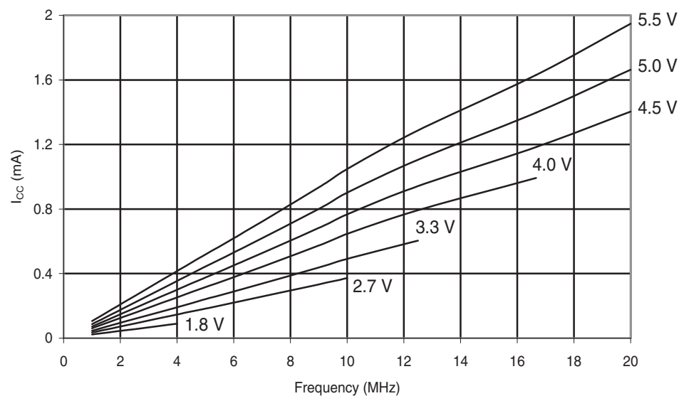
Figure 30-140. ATmega88A: Reset Supply Current vs. Frequency (1 - 20MHz)
