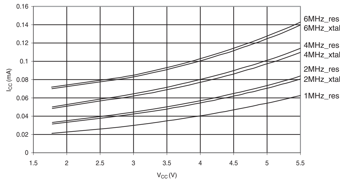
Figure 30-343. ATmega328P: Standby Supply Current vs. V CC (Watchdog Timer Disabled)
