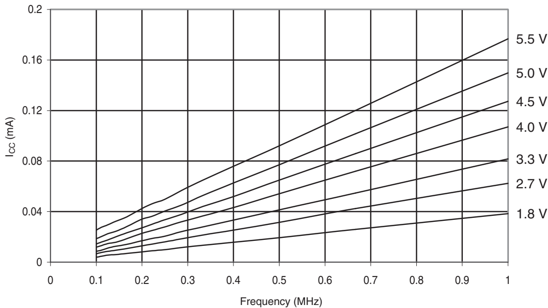
Figure 30-288.ATmega328: Idle Supply Current vs. Low Frequency (0.1-1.0MHz)
