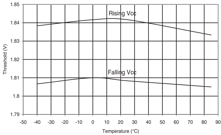
Figure 30-78. ATmega48PA: BOD Thresholds vs. Temperature (BODLEVEL is 1.8 V)
