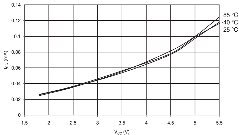
Figure 30-3. ATmega48A: Active Supply Current vs. V_{CC} (Internal RC Oscillator, 128kHz)
