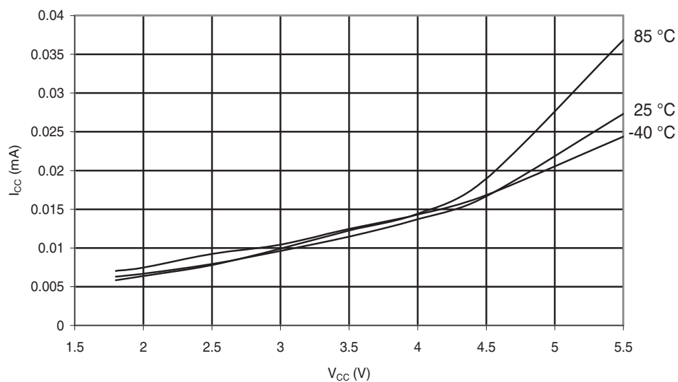
Figure 30-243. ATmega168PA: Idle Supply Current vs. V_{CC} (Internal RC Oscillator, 128kHz)
