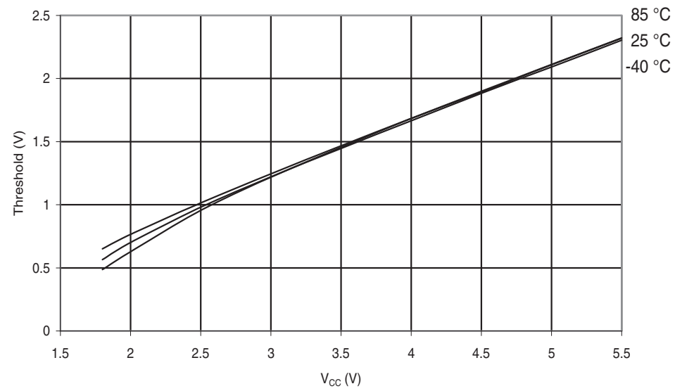
Figure 30-214. ATmega168A: I/O Pin Input Threshold Voltage vs. V_{CC} ( V_{IL} , I/O Pin read as '0')
