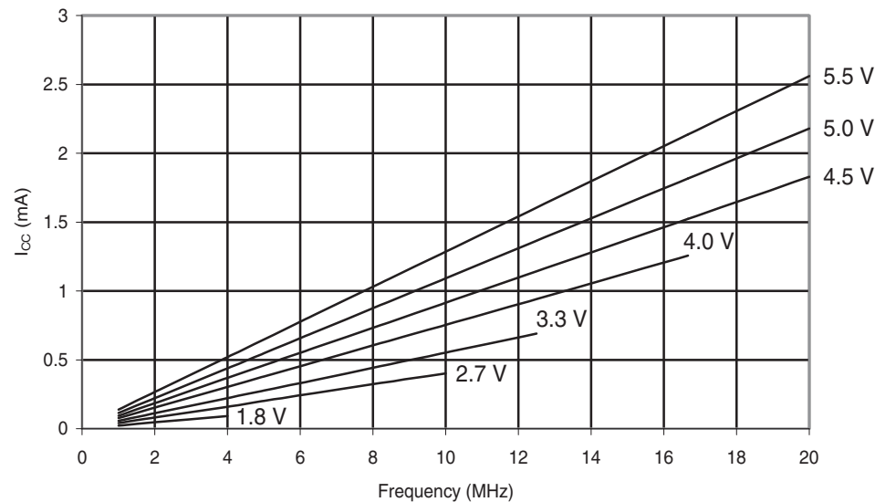
Figure 30-242. ATmega168PA: Idle Supply Current vs. Frequency (1-20MHz)
