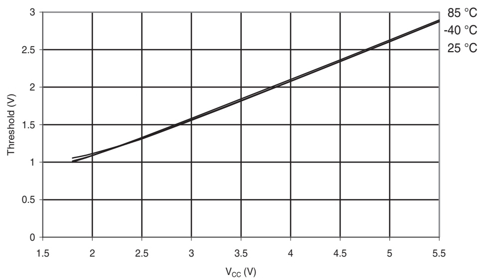
Figure 30-119. ATmega88A: I/O Pin Input Threshold Voltage vs. V_{CC} ( V_{IH} , I/O Pin read as '1')
