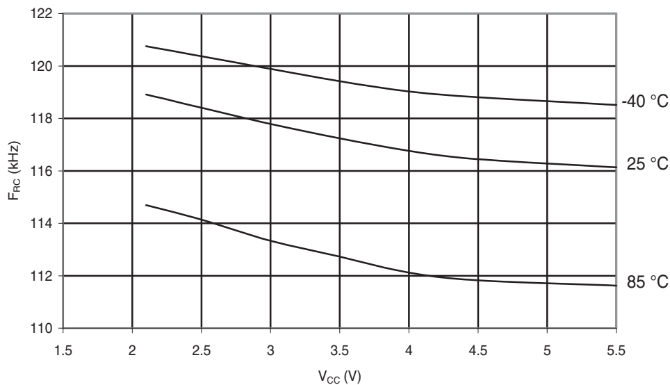
Figure 30-271.ATmega168PA: Watchdog Oscillator Frequency vs. V_{CC}
