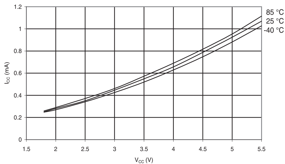
Figure 30-4. ATmega48A: Active Supply Current vs. V_{CC} (Internal RC Oscillator, 1MHz)
