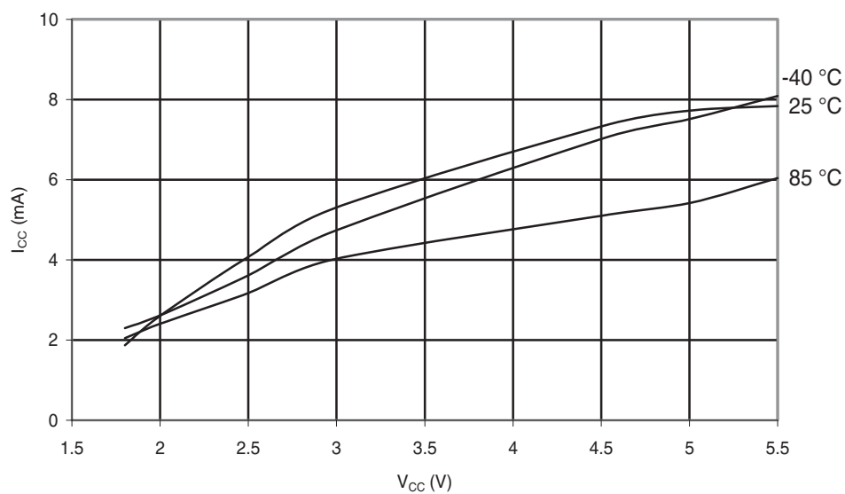
Figure 30-279. ATmega168PA: Programming Current vs. V_{CC}
