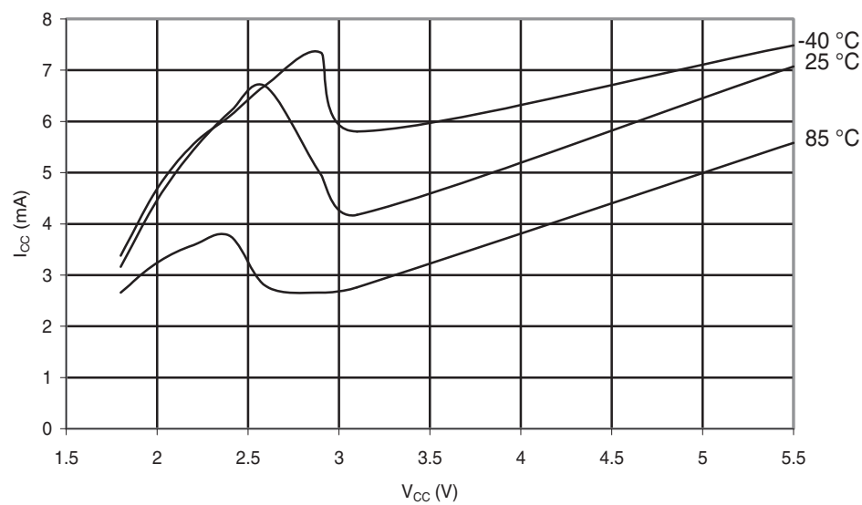
Figure 30-185. ATmega88PA: Programming Current vs. V_{CC}
