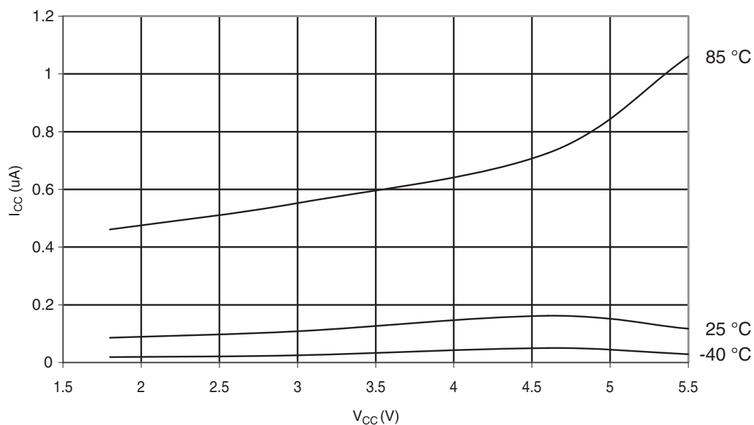
Figure 30-340. ATmega328P: Power-Down Supply Current vs. V_{CC} (Watchdog Timer Disabled)
