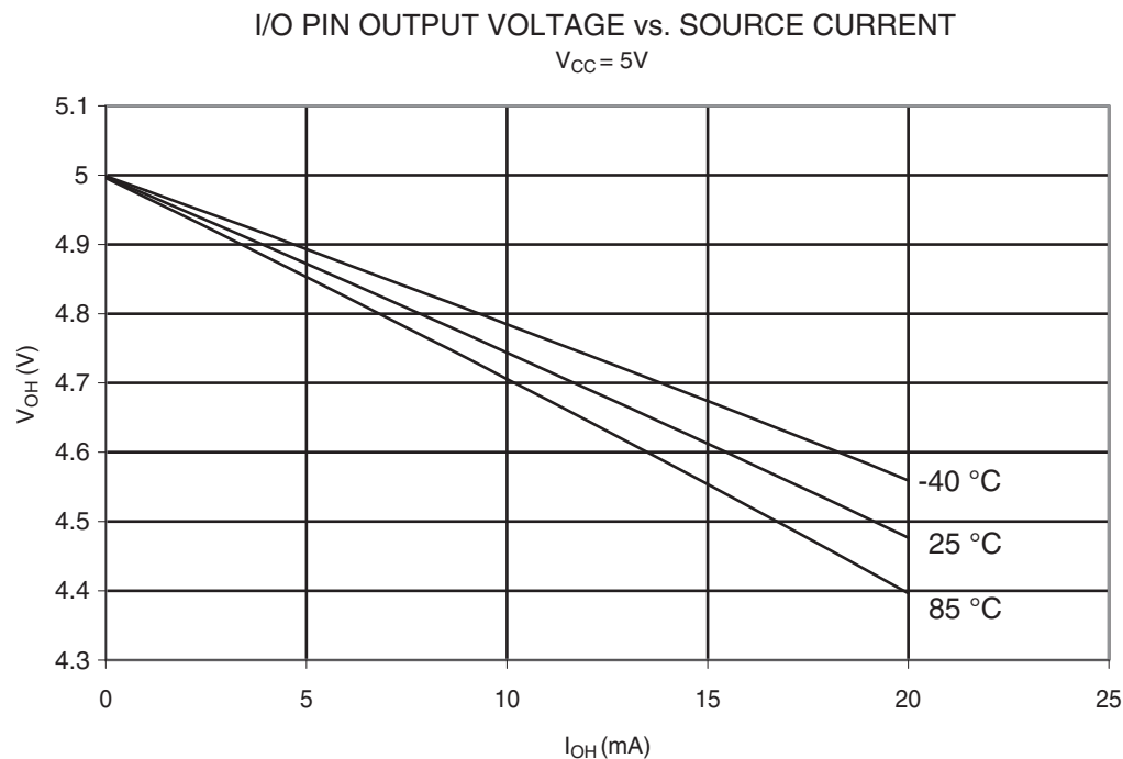
Figure 30-306. ATmega328: I/O Pin Output Voltage vs. Source Current ( V_{CC} = 5\text{ V} )
