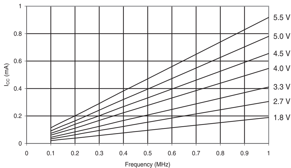
Figure 30-1. ATmega48A: Active Supply Current vs. Low Frequency (0.1-1.0MHz)
