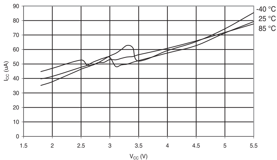
Figure 30-182. ATmega88PA: Analog Comparator Current vs. V_{CC}
