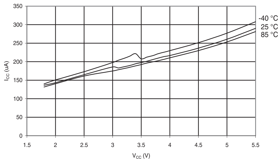
Figure 30-40. ATmega48A: ADC Current vs. V_{CC} (AREF = AV_{CC} )
