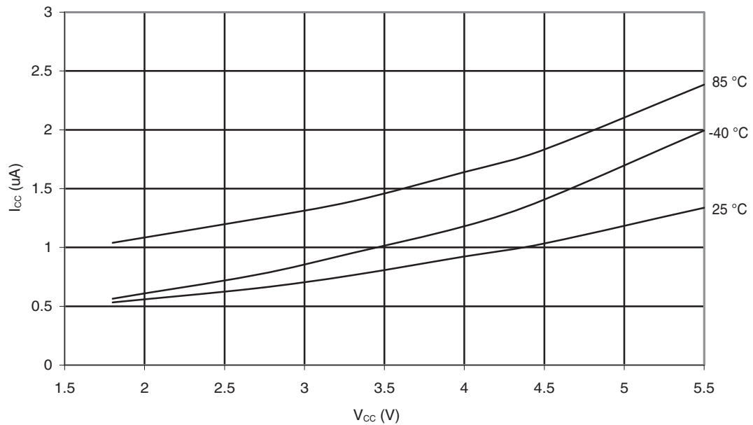
Figure 30-154. ATmega88PA: Power-Save Supply Current vs. V_{CC} (Watchdog Timer Disabled and 32kHz Crystal Oscillator Running)
