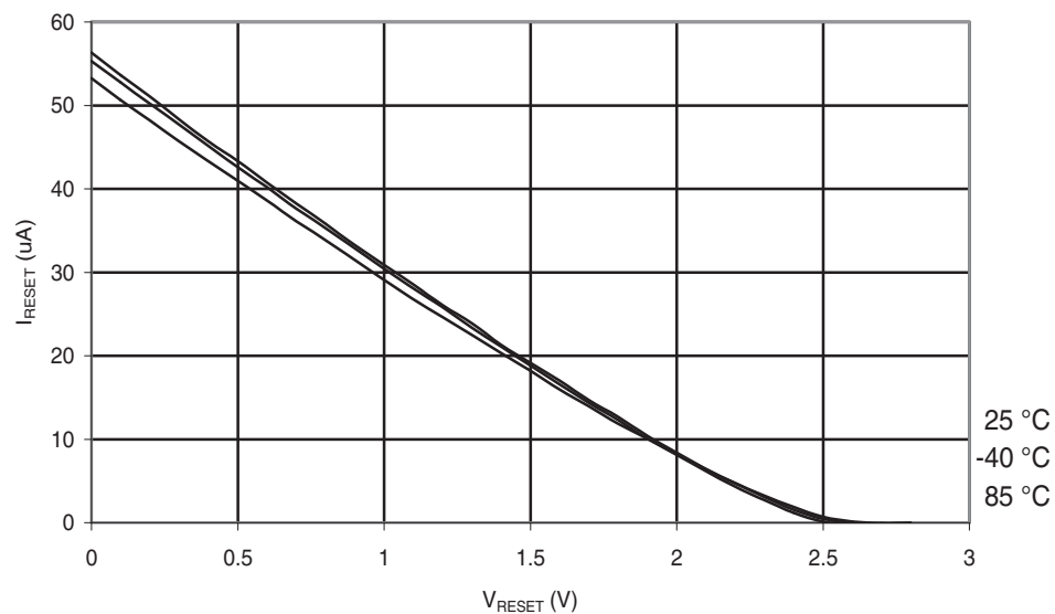
Figure 30-207. ATmega168A: Reset Pull-up Resistor Current vs. Reset Pin Voltage ( V_{CC} = 2.7\text{ V} )
