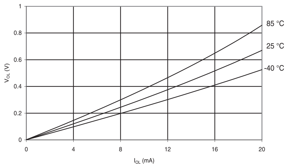
Figure 30-162. ATmega88PA: I/O Pin Output Voltage vs. Sink Current ( V_{CC} = 3\text{ V} )
