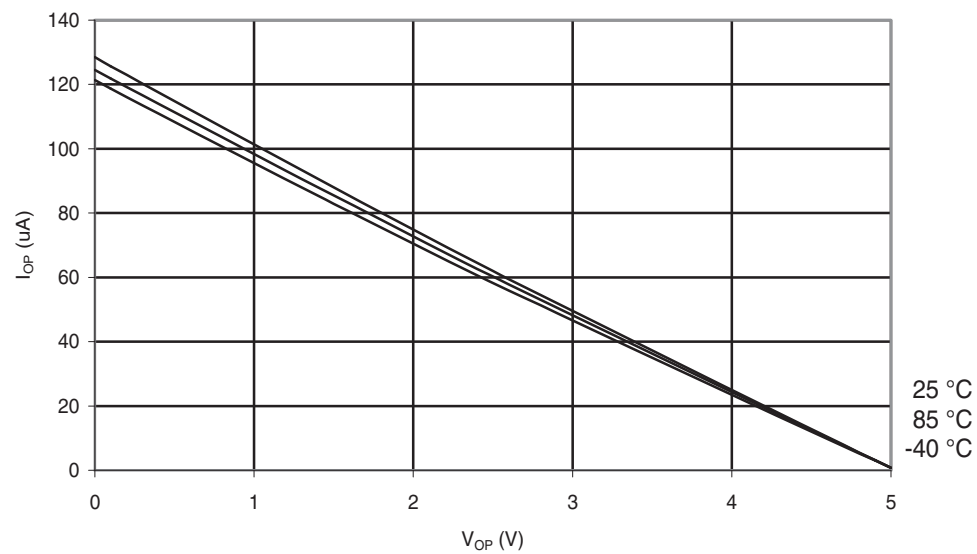
Figure 30-64. ATmega48PA: I/O Pin Pull-up Resistor Current vs. Input Voltage ( V_{CC} = 5\text{ V} )
