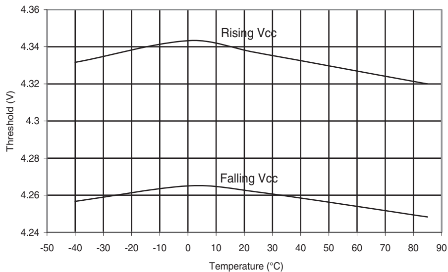
Figure 30-80. ATmega48PA: BOD Thresholds vs. Temperature (BODLEVEL is 4.3 V)
