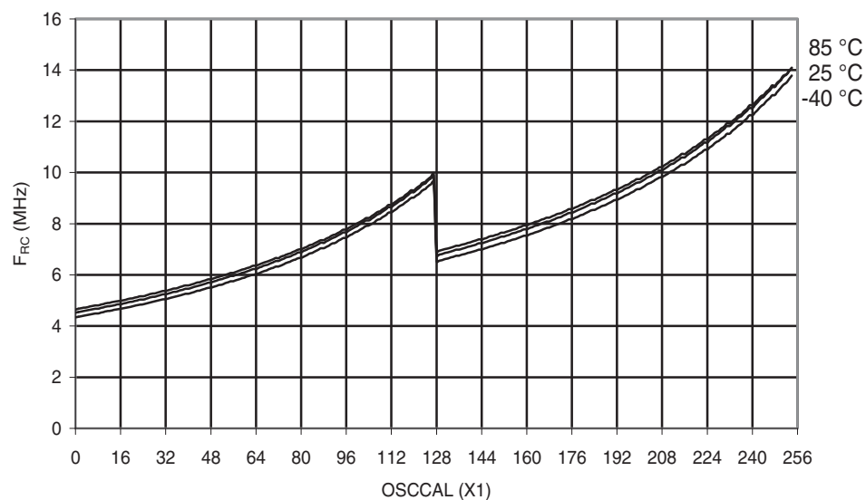
Figure 30-39. ATmega48A: Calibrated 8MHz RC Oscillator Frequency vs. OSCCAL Value
