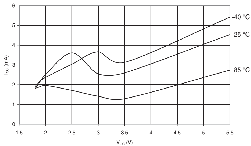
Figure 30-91. ATmega48PA: Programming Current vs. V_{CC}
