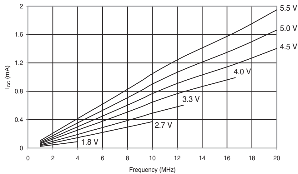
Figure 30-187.ATmega88PA: Reset Supply Current vs. Frequency (1 - 20MHz)
