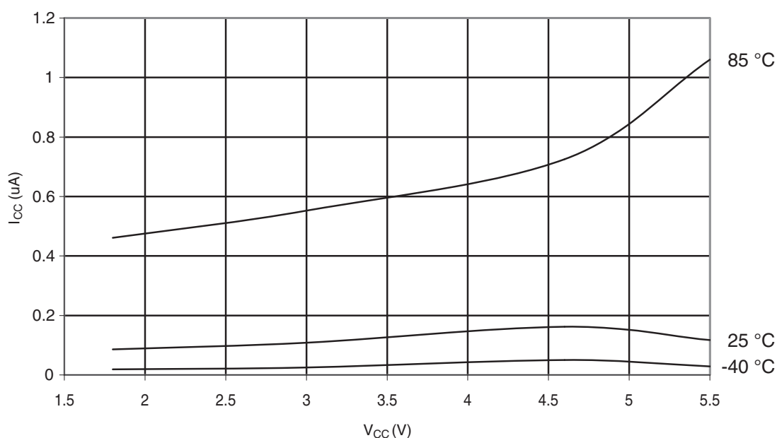
Figure 30-293. ATmega328: Power-Down Supply Current vs. V_{CC} (Watchdog Timer Disabled)
