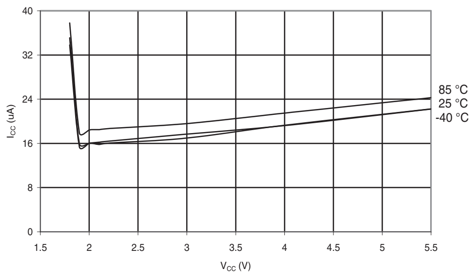
Figure 30-43. ATmega48A Brownout Detector Current vs. V_{CC}
