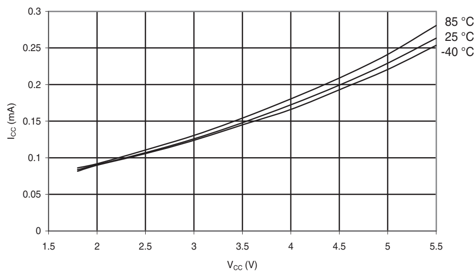
Figure 30-197. ATmega168A: Idle Supply Current vs. V_{CC} (Internal RC Oscillator, 1MHz)
