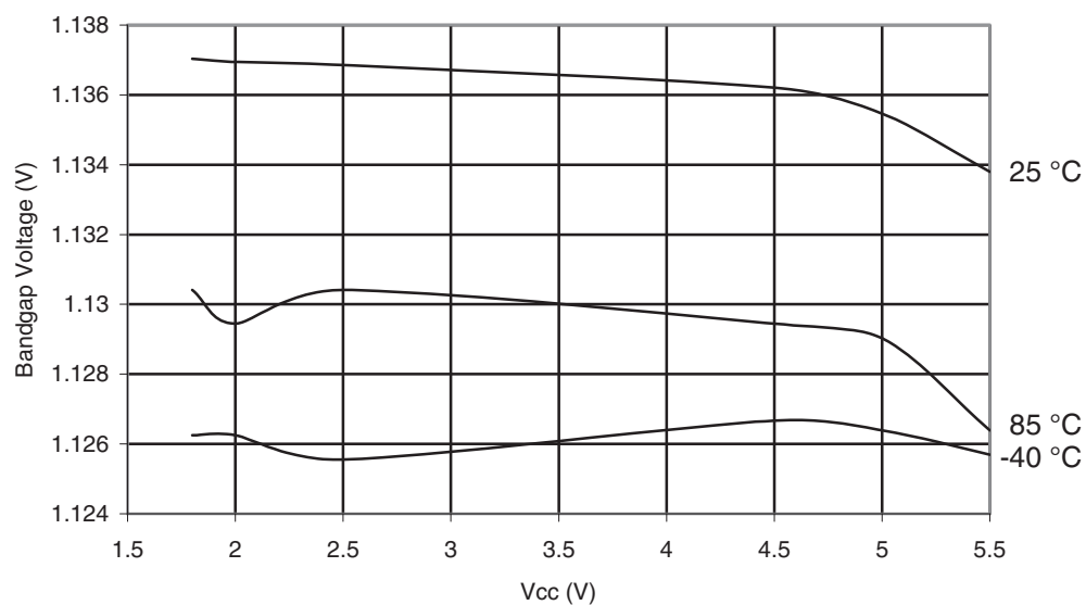
Figure 30-363. ATmega328P: Bandgap Voltage vs. V_{CC}
