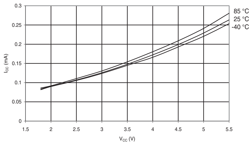
Figure 30-244. ATmega168PA: Idle Supply Current vs. V_{CC} (Internal RC Oscillator, 1MHz)
