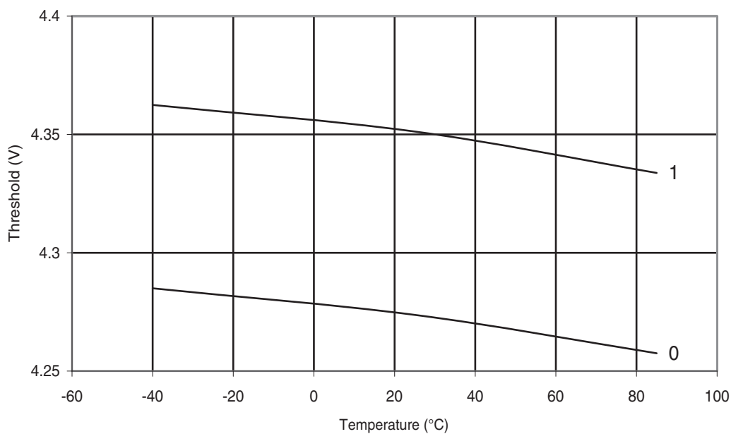
Figure 30-315. ATmega328: BOD Thresholds vs. Temperature (BODLEVEL is 4.3 V)
