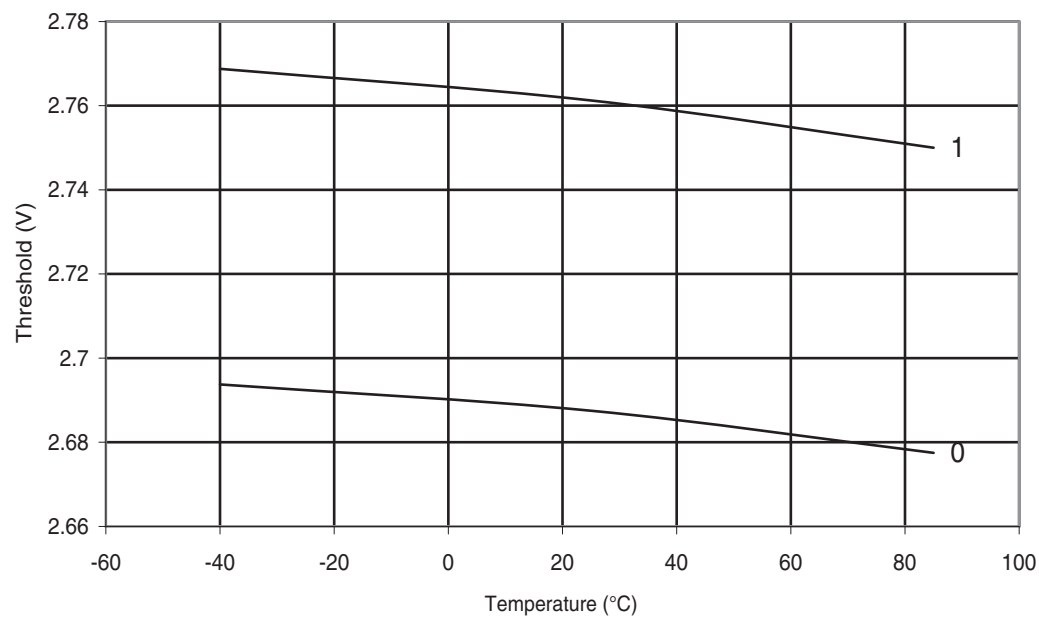
Figure 30-361.ATmega328P: BOD Thresholds vs. Temperature (BODLEVEL is 2.7 V)
