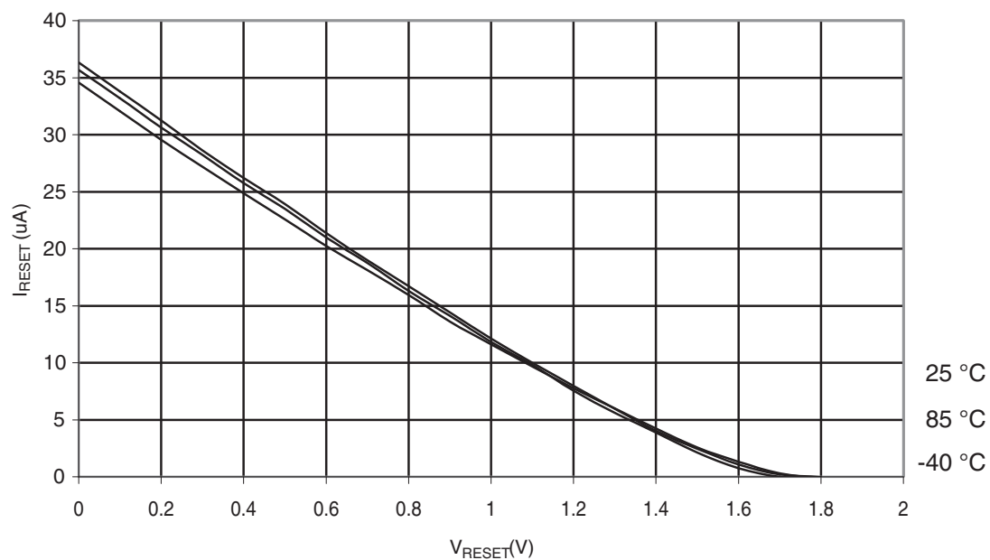
Figure 30-300. ATmega328: Reset Pull-up Resistor Current vs. Reset Pin Voltage ( V_{CC} = 1.8\text{ V} )
