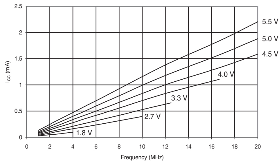
Figure 30-148.ATmega88PA: Idle Supply Current vs. Frequency (1 - 20MHz)
