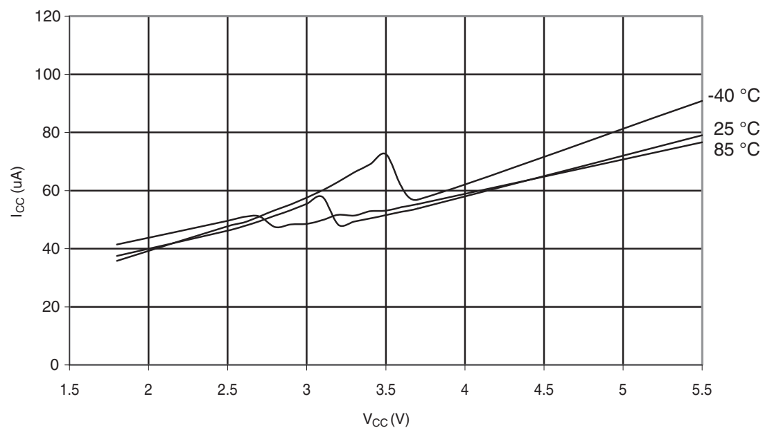
Figure 30-323. ATmega328: Analog Comparator Current vs. V_{CC}
