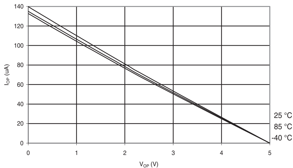
Figure 30-158. ATmega88PA: I/O Pin Pull-up Resistor Current vs. Input Voltage ( V_{CC} = 5\text{ V} )
