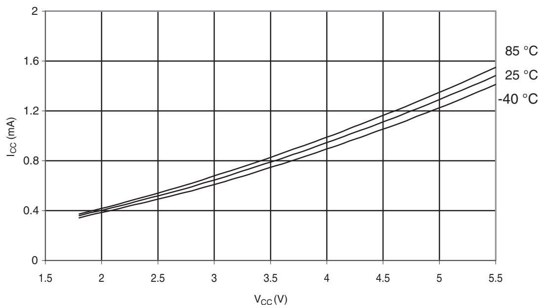
Figure 30-292. ATmega328: Idle Supply Current vs. V_{CC} (Internal RC Oscillator, 8MHz)
