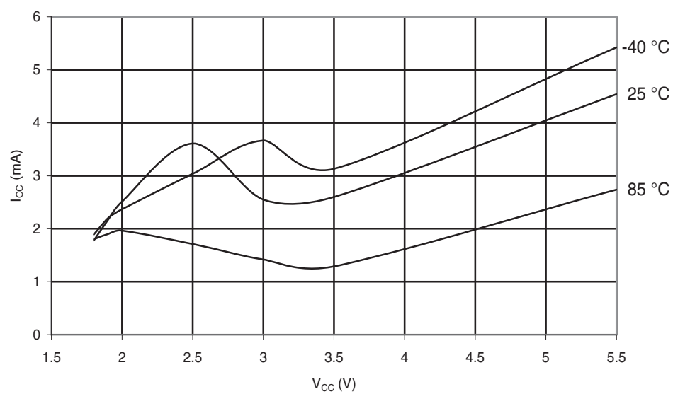
Figure 30-44. ATmega48A: Programming Current vs. V_{CC}
