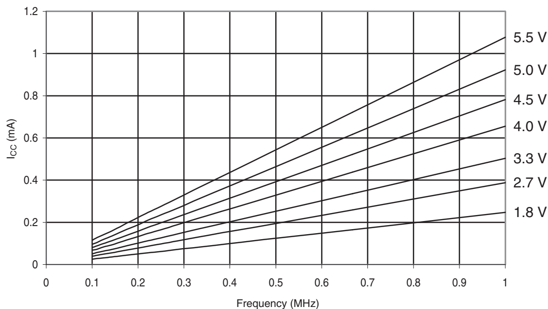
Figure 30-283. ATmega328: Active Supply Current vs. Low Frequency (0.1-1.0MHz)
