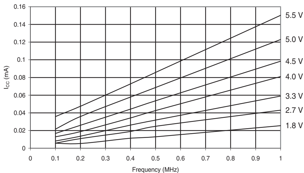
Figure 30-6. ATmega48A: Idle Supply Current vs. Low Frequency (0.1-1.0MHz)
