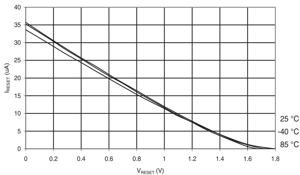
Figure 30-253. ATmega168PA: Reset Pull-up Resistor Current vs. Reset Pin Voltage ( V_{CC} = 1.8\text{ V} )
