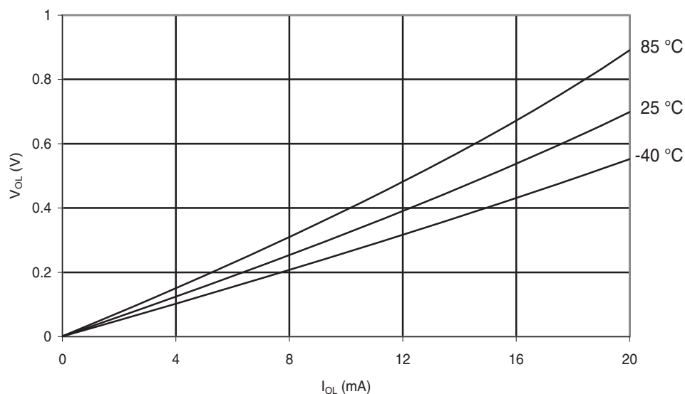
Figure 30-21. ATmega48A: I/O Pin Output Voltage vs. Sink Current ( V_{CC} = 3\text{ V} )
