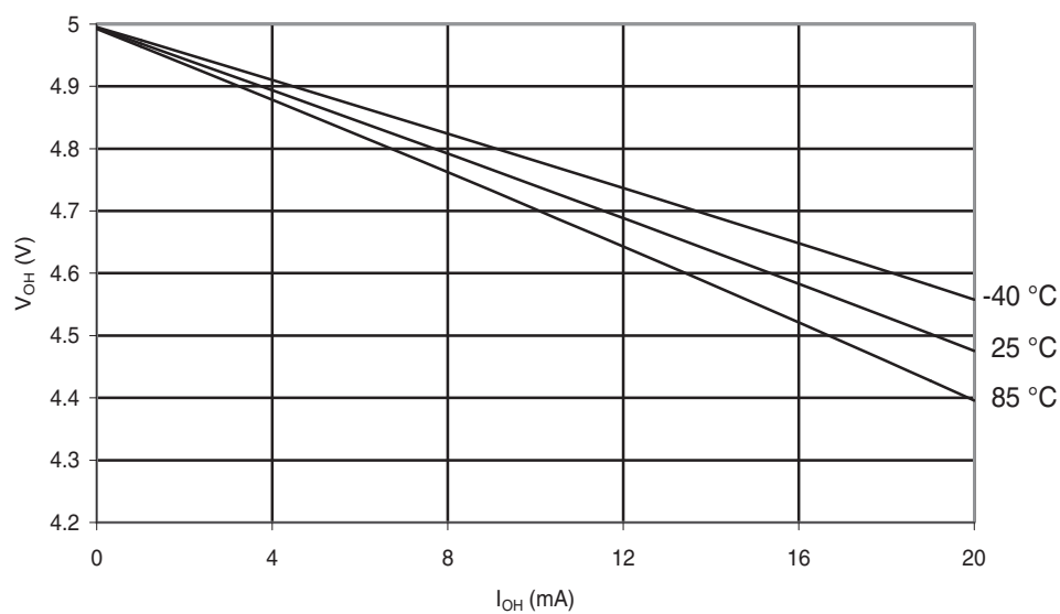
Figure 30-165. ATmega88PA: I/O Pin Output Voltage vs. Source Current ( V_{CC} = 5\text{ V} )
