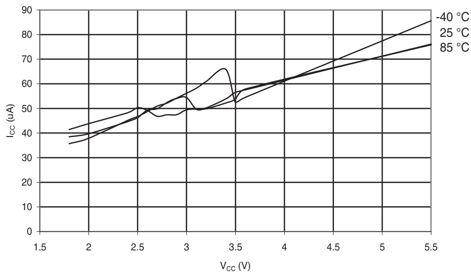
Figure 30-88. ATmega48PA: Analog Comparator Current vs. V_{CC}
