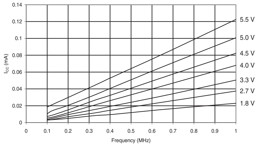
Figure 30-92. ATmega48PA: Reset Supply Current vs. Low Frequency (0.1 - 1.0MHz)
