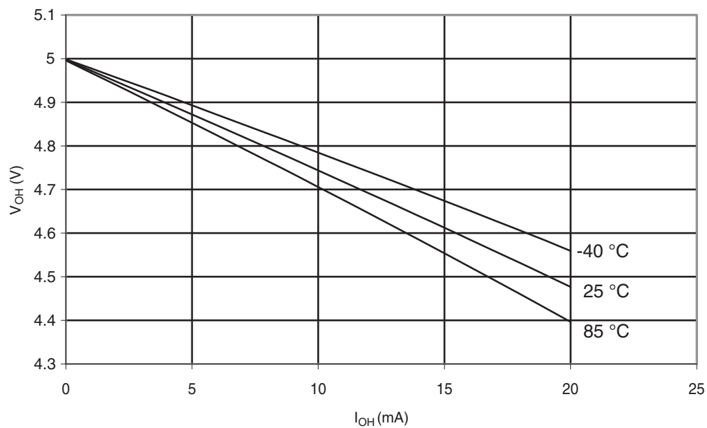
Figure 30-353. ATmega328P: I/O Pin Output Voltage vs. Source Current ( V_{CC} = 5\text{ V} )
