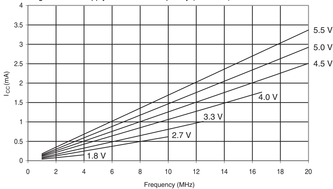
Figure 30-289.ATmega328: Idle Supply Current vs. Frequency (1-20MHz)
