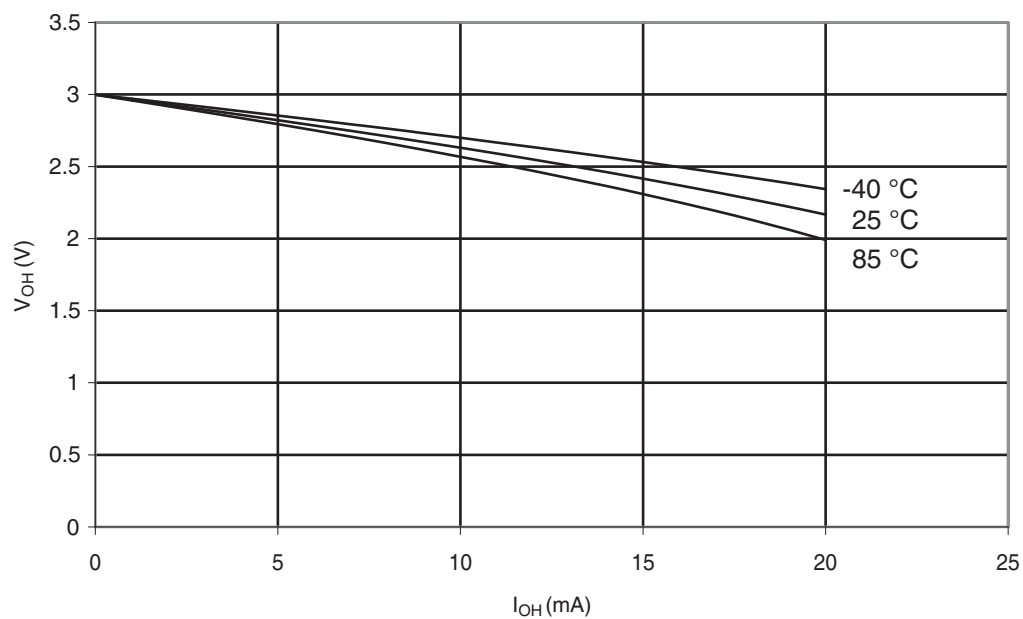
Figure 30-352. ATmega328P: I/O Pin Output Voltage vs. Source Current ( V_{CC} = 3\text{ V} )
