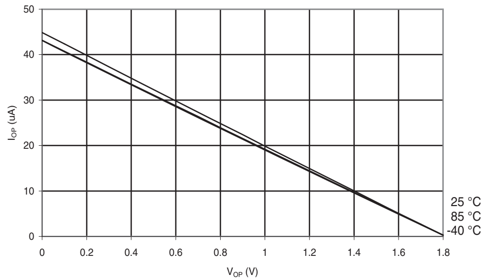
Figure 30-15. ATmega48A: I/O Pin Pull-up Resistor Current vs. Input Voltage ( V_{CC} = 1.8\text{ V} )
