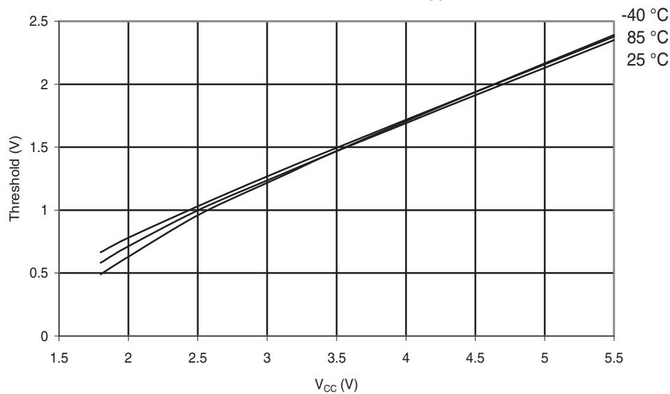
Figure 30-167. ATmega88PA: I/O Pin Input Threshold Voltage vs. V_{CC} ( V_{IL} , I/O Pin read as '0')
