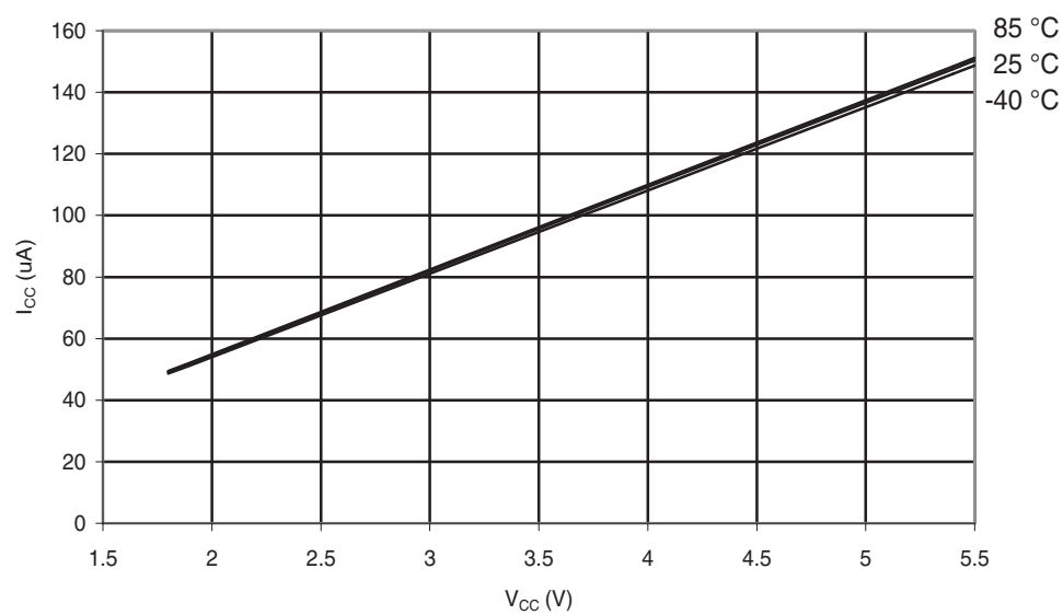
Figure 30-183. ATmega88PA: AREF External Reference Current vs. V_{CC}
