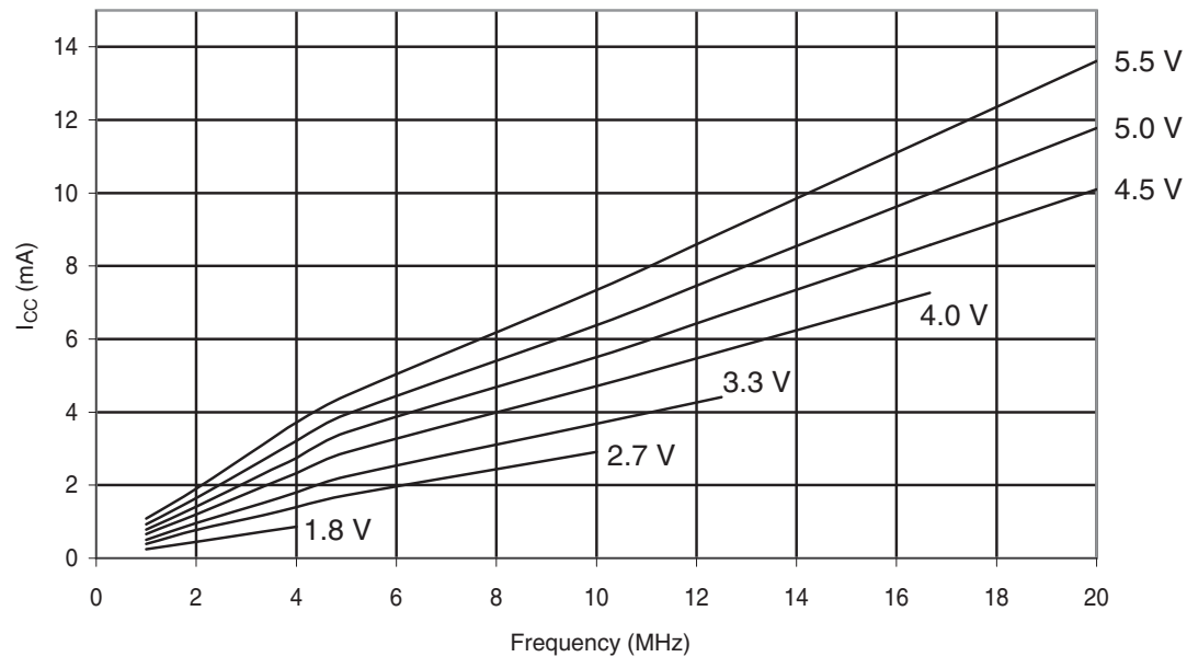
Figure 30-331. ATmega328P: Active Supply Current vs. Frequency (1-20MHz)
