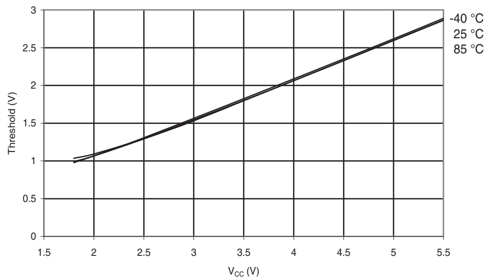
Figure 30-25. ATmega48A: I/O Pin Input Threshold Voltage vs. V_{CC} ( V_{IH} , I/O Pin read as '1')
