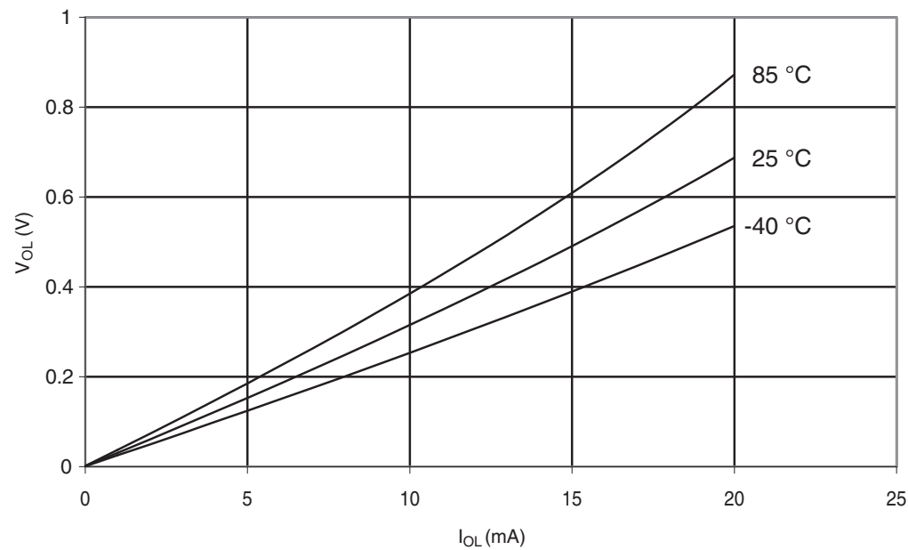
Figure 30-350. ATmega328P: I/O Pin Output Voltage vs. Sink Current ( V_{CC} = 3\text{ V} )
