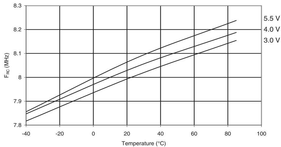
Figure 30-132. ATmega88A: Calibrated 8MHz RC Oscillator Frequency vs. Temperature
