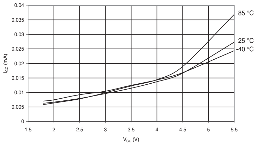
Figure 30-197. ATmega168A: Idle Supply Current vs. V_{CC} (Internal RC Oscillator, 1MHz)
