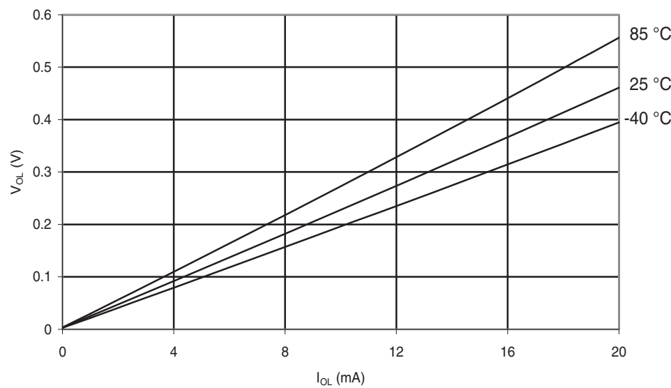
Figure 30-257. ATmega168PA: I/O Pin Output Voltage vs. Sink Current ( V_{CC} = 5\text{ V} )
