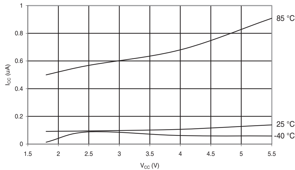
Figure 30-246. ATmega168PA: Power-Down Supply Current vs. V_{CC} (Watchdog Timer Disabled)
