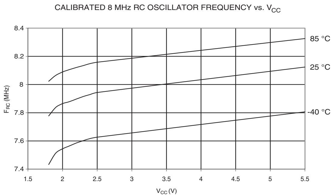
Figure 30-319. ATmega328: Calibrated 8MHz RC Oscillator Frequency vs. V_{CC}
