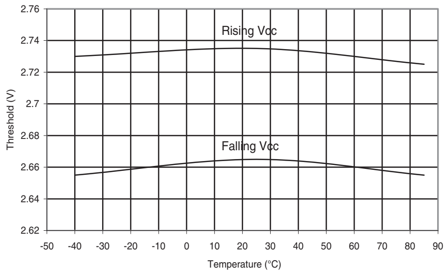
Figure 30-220.ATmega168A: BOD Thresholds vs. Temperature (BODLEVEL is 2.7 V)
