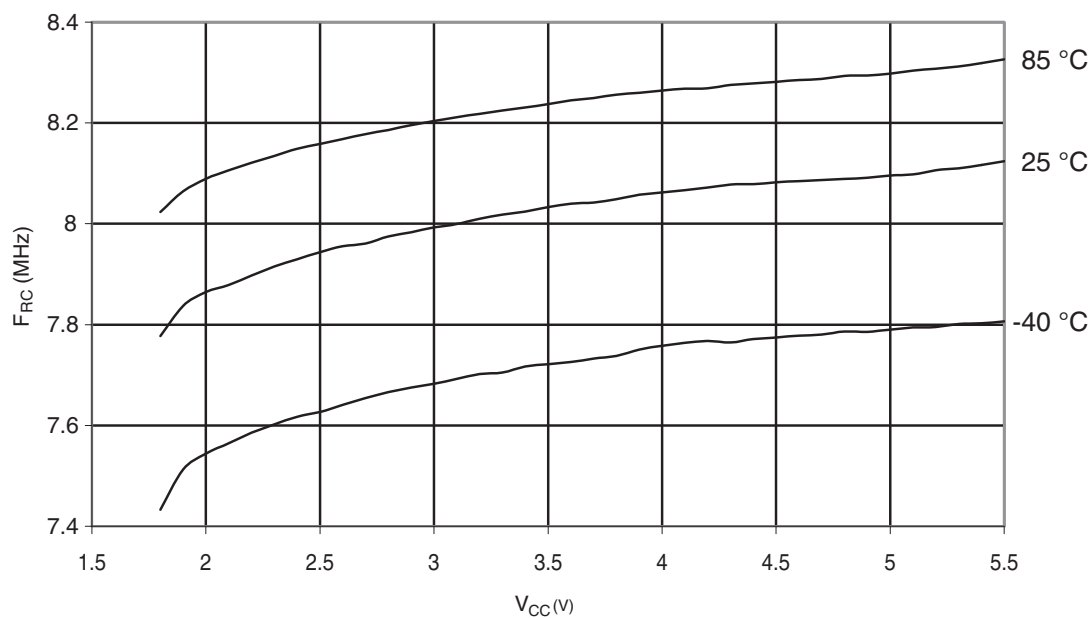
Figure 30-366. ATmega328P: Calibrated 8MHz RC Oscillator Frequency vs. V_{CC}
