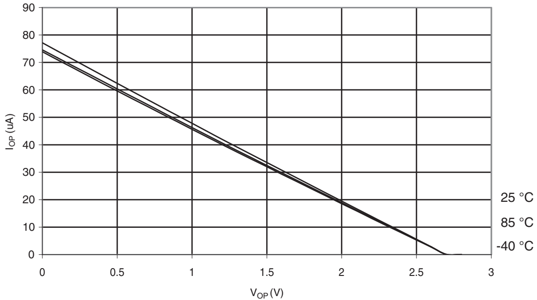
Figure 30-345. ATmega328P: I/O Pin Pull-up Resistor Current vs. Input Voltage ( V_{CC} = 2.7\text{ V} )
