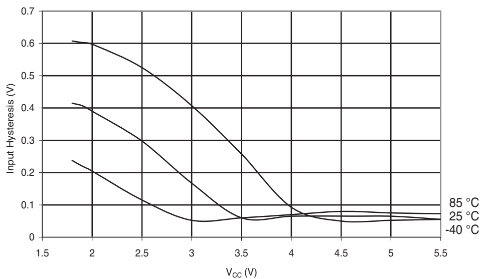
Figure 30-77. ATmega48PA: Reset Pin Input Hysteresis vs. V_{CC}
