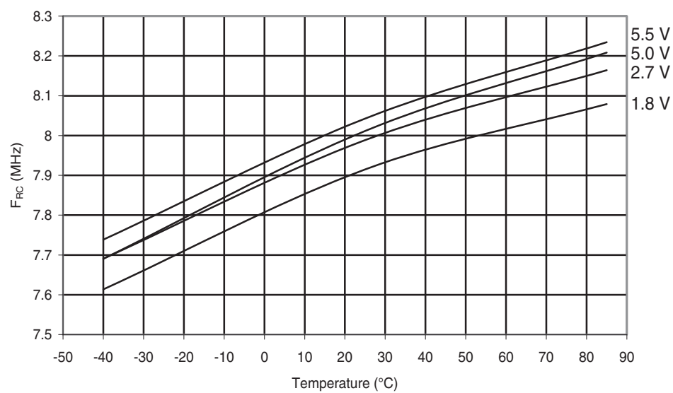
Figure 30-226. ATmega168A: Calibrated 8MHz RC Oscillator Frequency vs. Temperature
