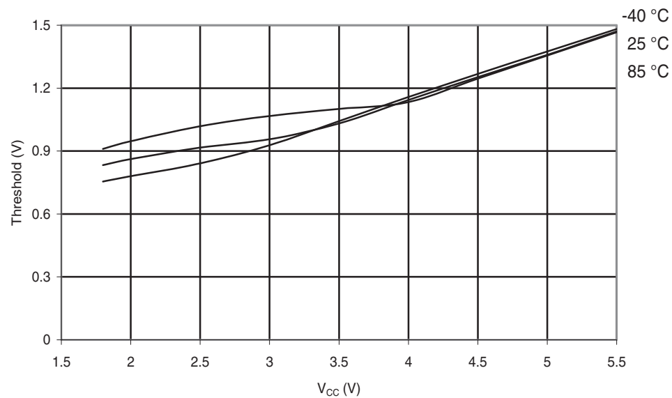
Figure 30-169. ATmega88PA: Reset Input Threshold Voltage vs. V_{CC} ( V_{IH} , I/O Pin read as '1')
