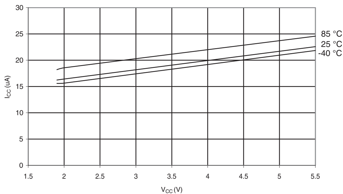
Figure 30-325. ATmega328: Brownout Detector Current vs. V_{CC}
