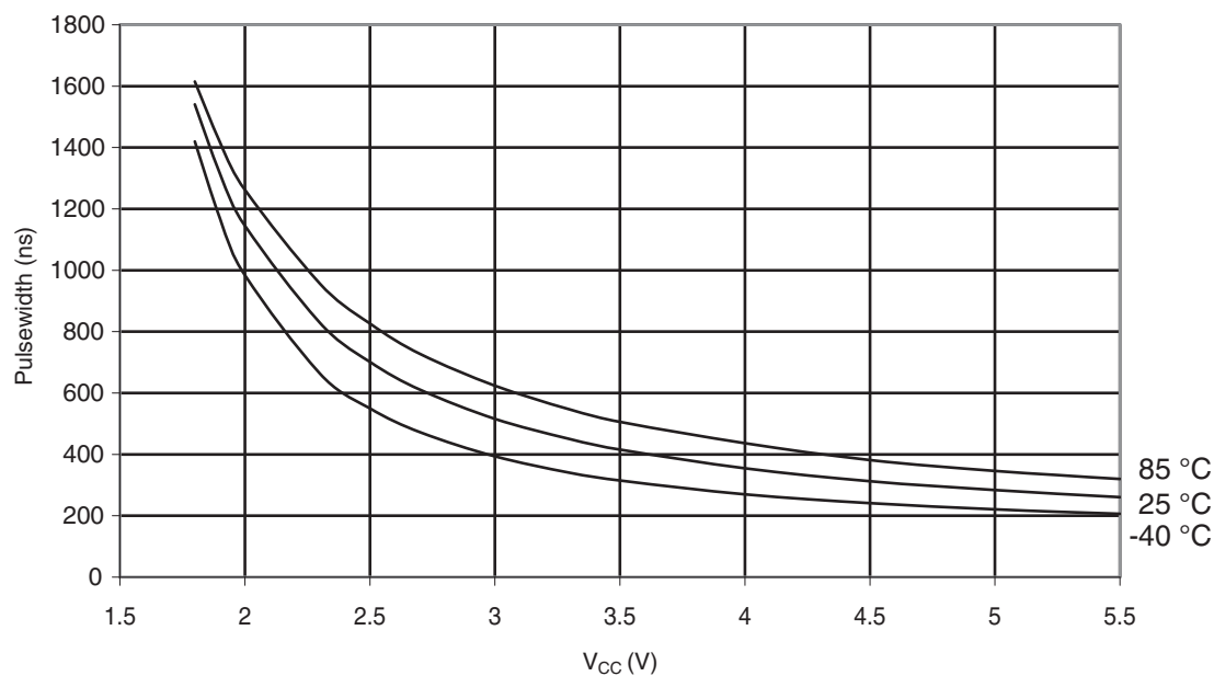
Figure 30-376. ATmega328P: Minimum Reset Pulse width vs. V_{CC}
