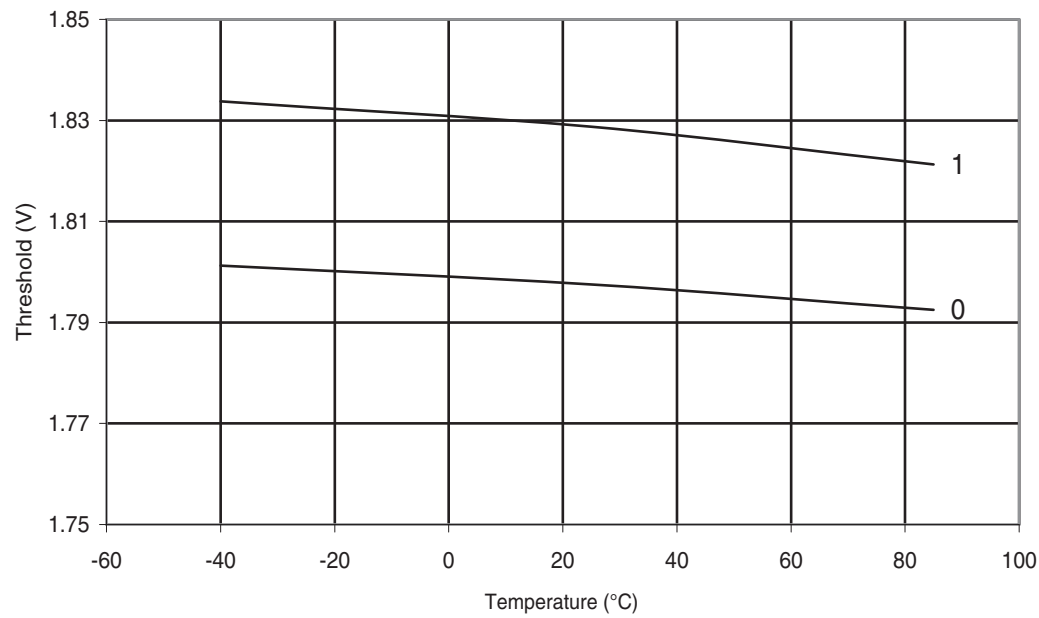
Figure 30-360.ATmega328P: BOD Thresholds vs. Temperature (BODLEVEL is 1.8 V)
