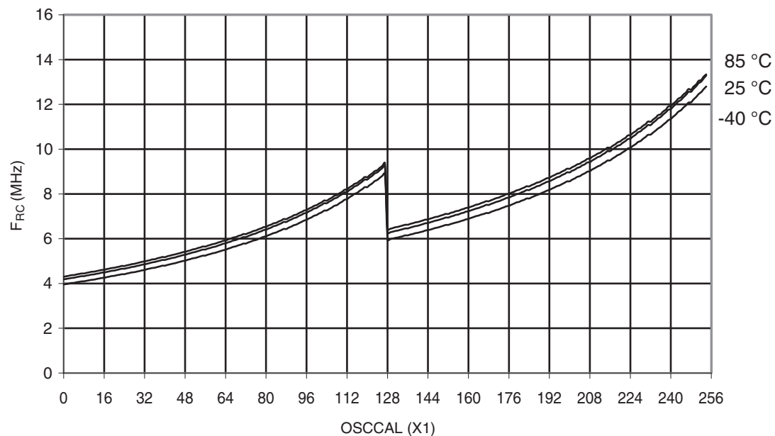
Figure 30-368. ATmega328P: Calibrated 8MHz RC Oscillator Frequency vs. OSCCAL Value
