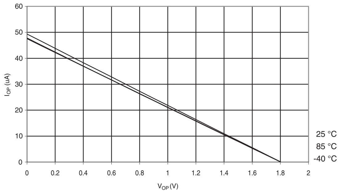
Figure 30-297. ATmega328: I/O Pin Pull-up Resistor Current vs. Input Voltage ( V_{CC} = 1.8 V)
