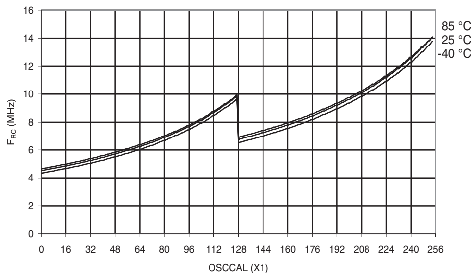
Figure 30-86. ATmega48PA: Calibrated 8MHz RC Oscillator Frequency vs. OSCCAL Value
