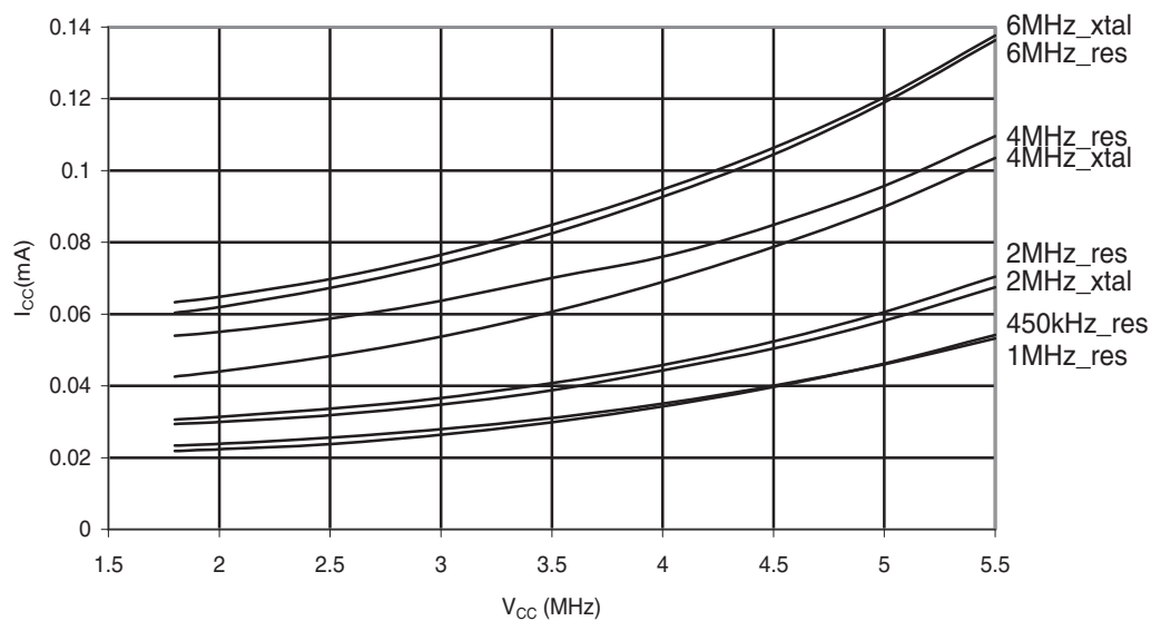
Figure 30-202. ATmega168A: Standby Supply Current vs. V_{CC} (Watchdog Timer Disabled)
