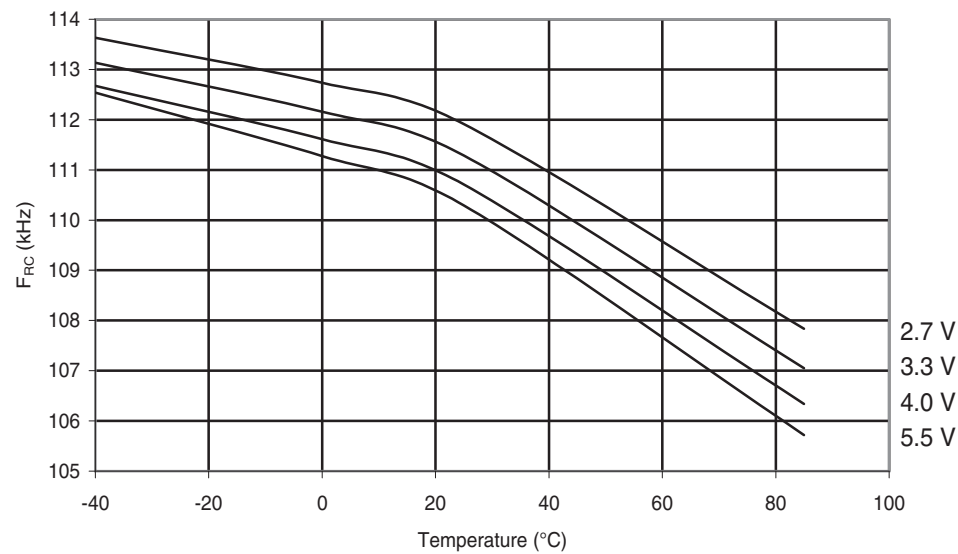
Figure 30-176.ATmega88PA: Watchdog Oscillator Frequency vs. Temperature
