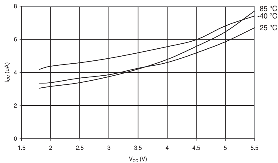
Figure 30-153. ATmega88PA: Power-Down Supply Current vs. V_{CC} (Watchdog Timer Enabled)
