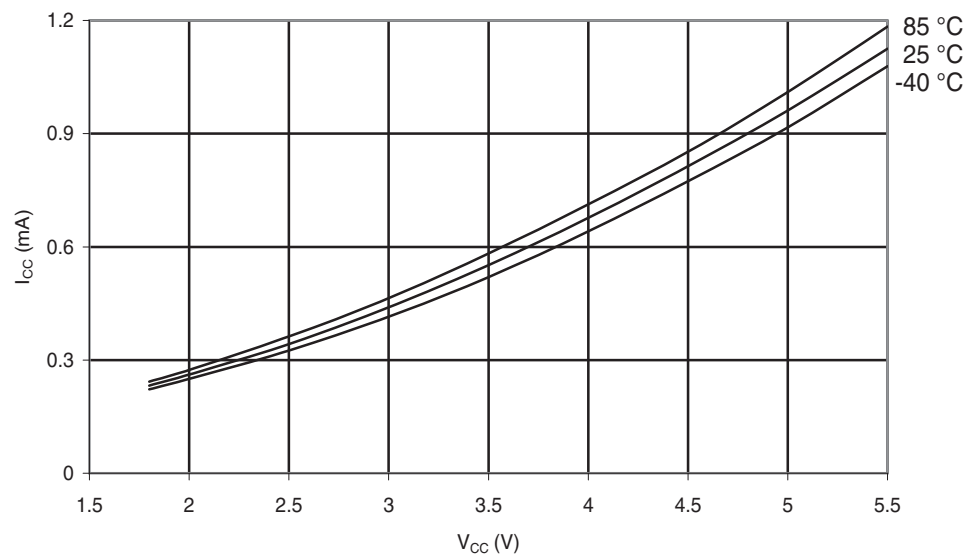
Figure 30-198. ATmega168A: Idle Supply Current vs. V CC (Internal RC Oscillator, 8MHz)
