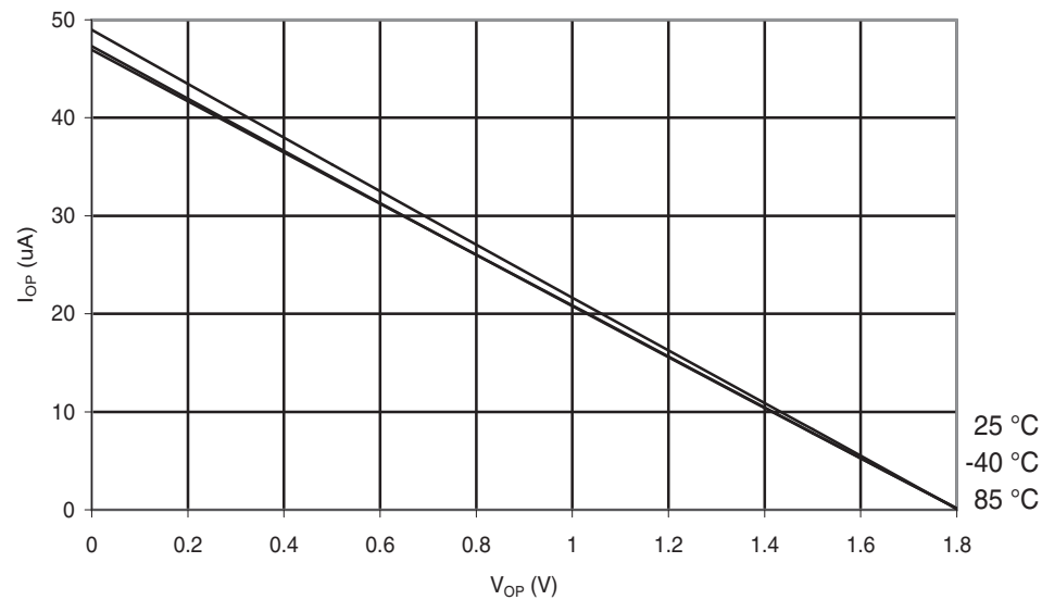
Figure 30-156.ATmega88PA: I/O Pin Pull-up Resistor Current vs. Input Voltage ( V_{CC} = 1.8\text{ V} )
