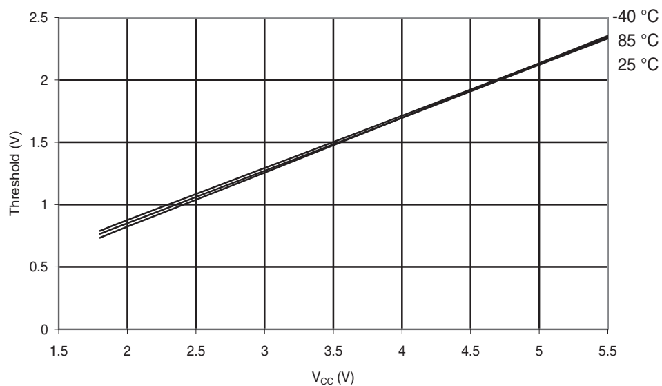
Figure 30-217. ATmega168A: Reset Input Threshold Voltage vs. V_{CC} ( V_{IL} , I/O Pin read as '0')
