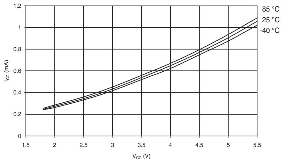
Figure 30-193. ATmega168A: Active Supply Current vs. V_{CC} (Internal RC Oscillator, 8MHz)
