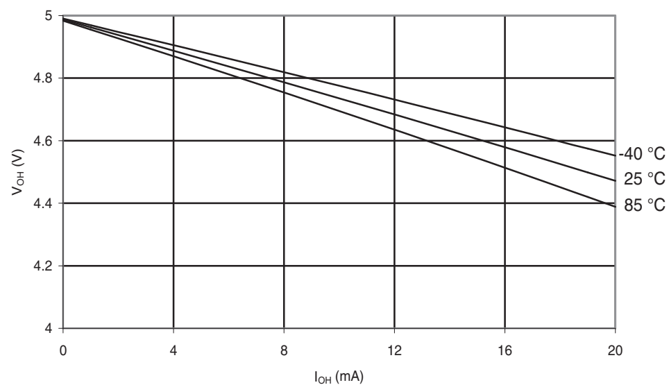
Figure 30-259. ATmega168PA: I/O Pin Output Voltage vs. Source Current ( V_{CC} = 5\text{ V} )
