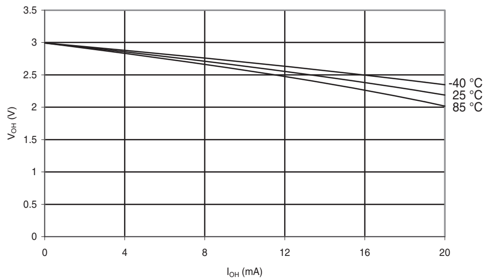
Figure 30-258. ATmega168PA: I/O Pin Output Voltage vs. Source Current ( V_{CC} = 3\text{ V} )
