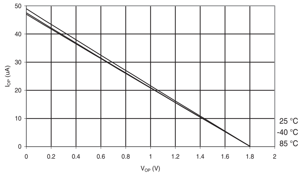
Figure 30-203.ATmega168A: I/O Pin Pull-up Resistor Current vs. Input Voltage ( V_{CC} = 1.8\text{ V} )
