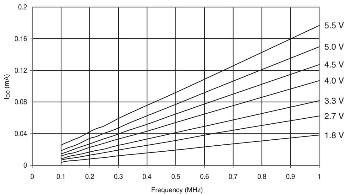
Figure 30-335. ATmega328P: Idle Supply Current vs. Low Frequency (0.1-1.0MHz)
