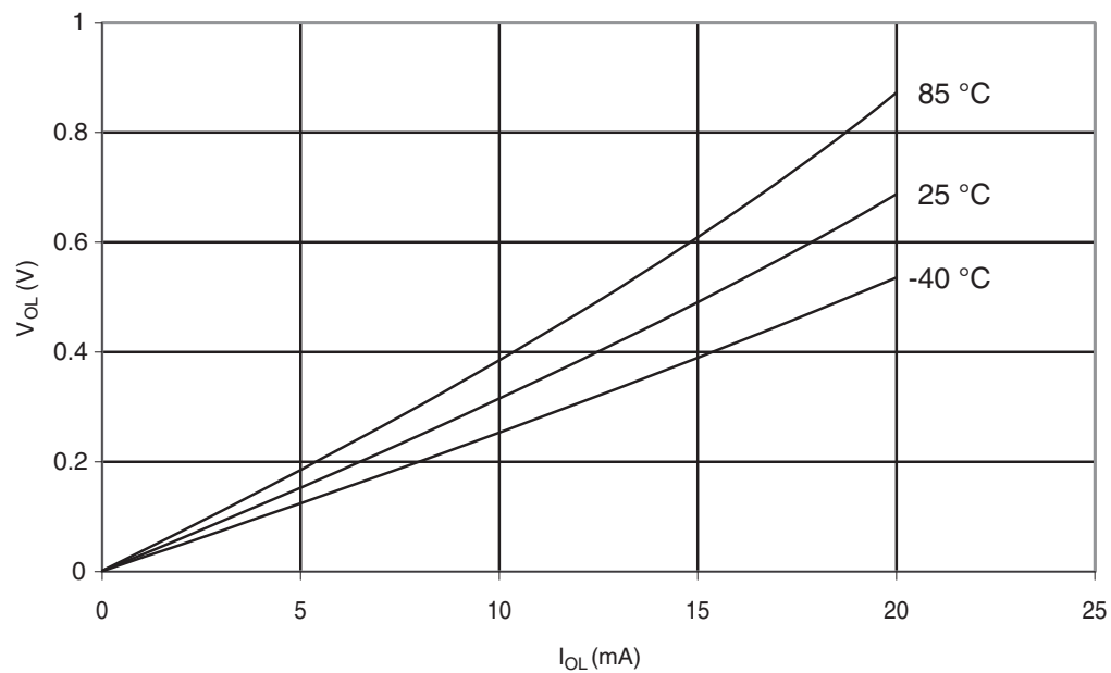
Figure 30-303. ATmega328: I/O Pin Output Voltage vs. Sink Current ( V_{CC} = 3\text{ V} )
