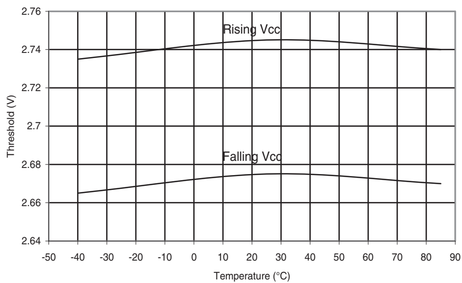
Figure 30-173.ATmega88PA: BOD Thresholds vs. Temperature (BODLEVEL is 2.7 V)
