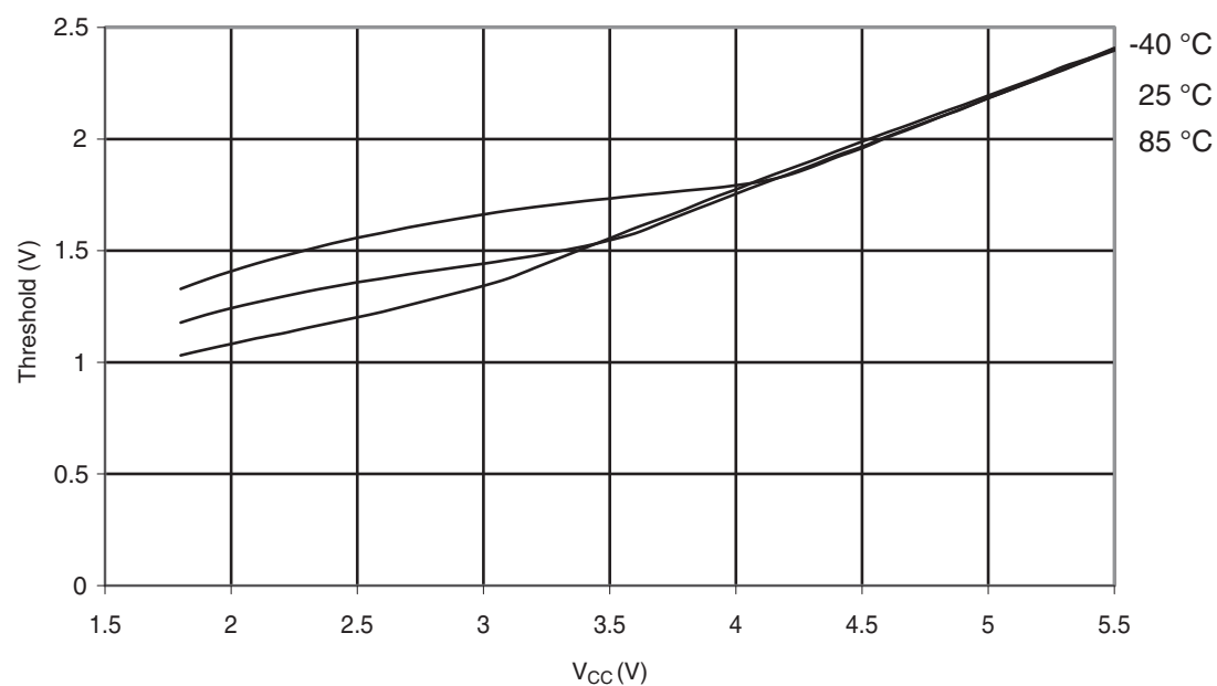
Figure 30-357. ATmega328P: Reset Input Threshold Voltage vs. V_{CC} ( V_{IH} , I/O Pin read as '1')
