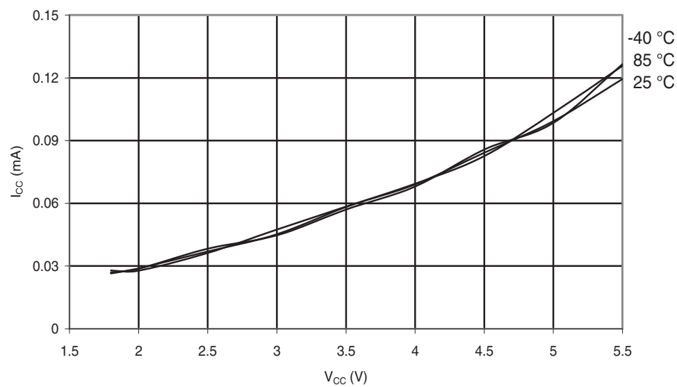
Figure 30-238. ATmega168PA: Active Supply Current vs. V_{CC} (Internal RC Oscillator, 128kHz)
