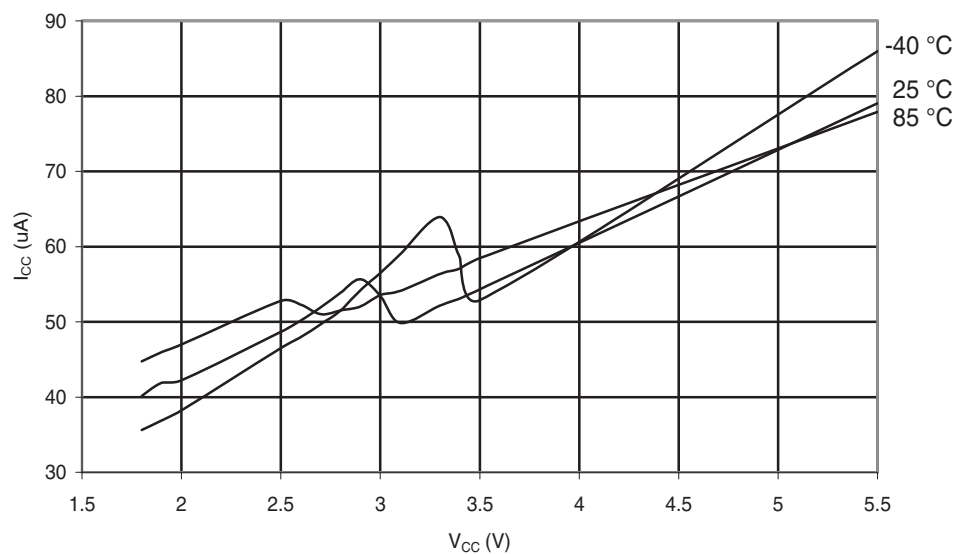
Figure 30-276. ATmega168PA: Analog Comparator Current vs. V_{CC}
