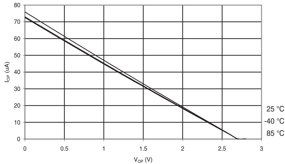
Figure 30-157.ATmega88PA: I/O Pin Pull-up Resistor Current vs. Input Voltage ( V_{CC} = 2.7\text{ V} )
