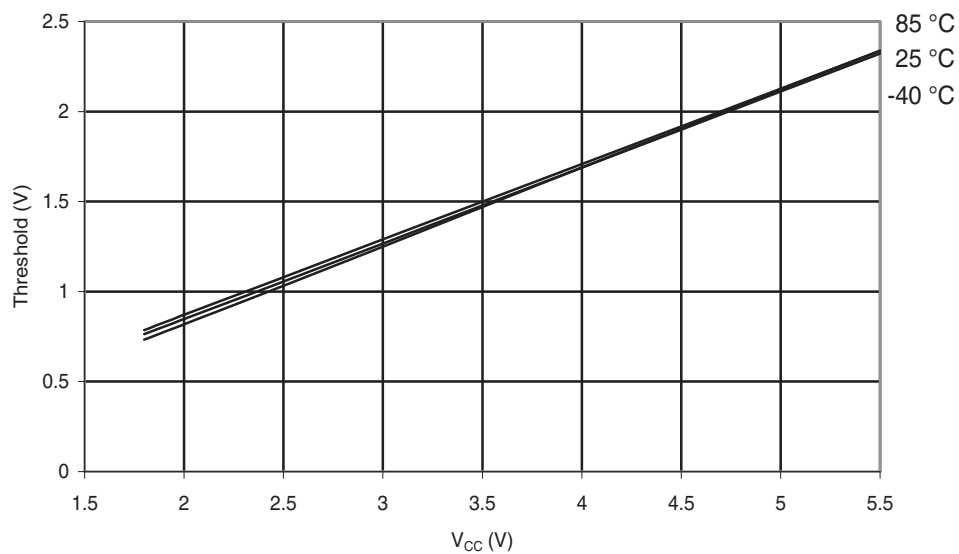
Figure 30-170. ATmega88PA: Reset Input Threshold Voltage vs. V_{CC} ( V_{IL} , I/O Pin read as '0')
