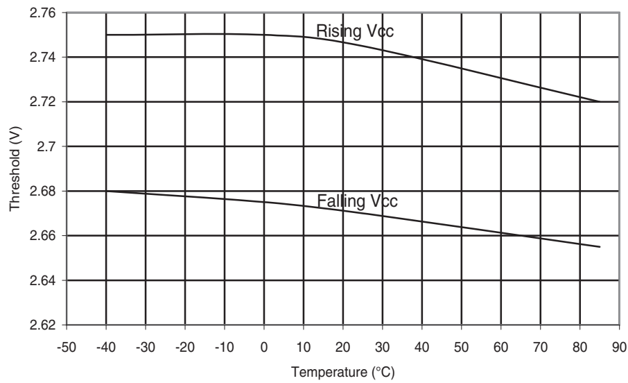
Figure 30-79. ATmega48PA: BOD Thresholds vs. Temperature (BODLEVEL is 2.7 V)
