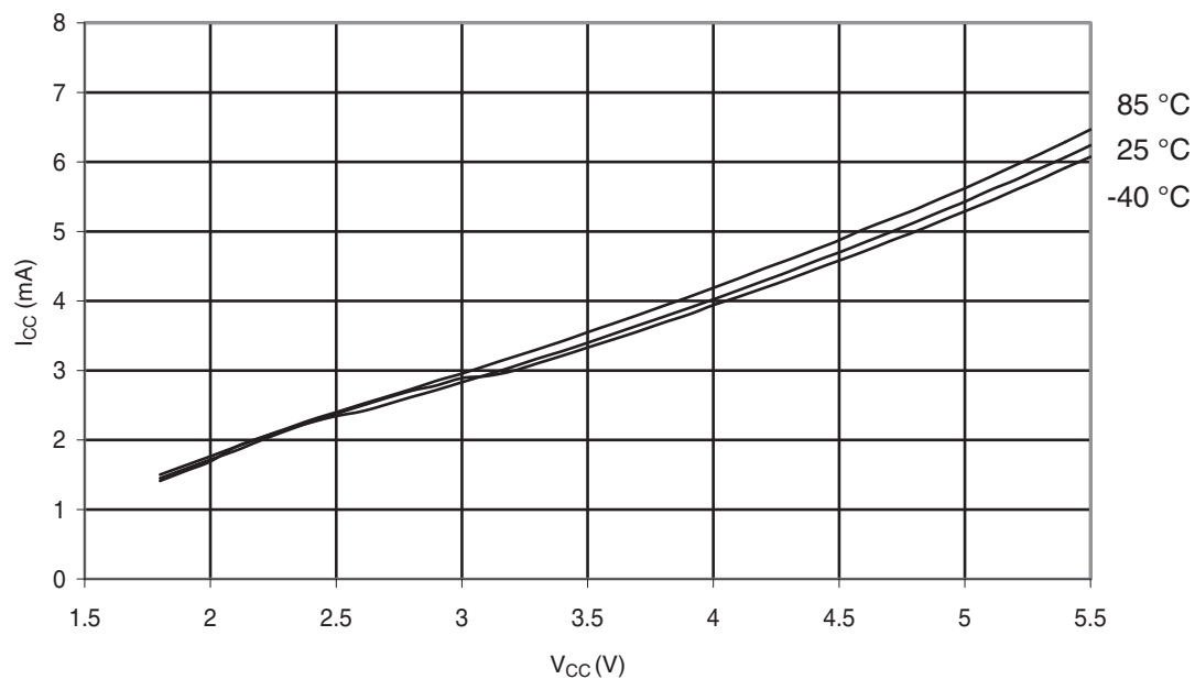
Figure 30-287. ATmega328: Active Supply Current vs. V_{CC} (Internal RC Oscillator, 8MHz)
