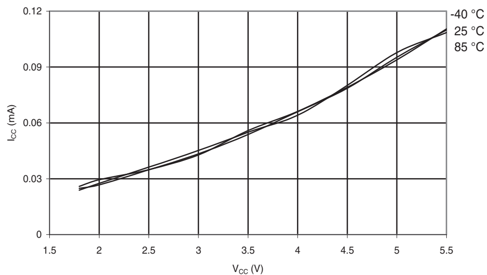
Figure 30-144. ATmega88PA: Active Supply Current vs. V_{CC} (Internal RC Oscillator, 128kHz)
