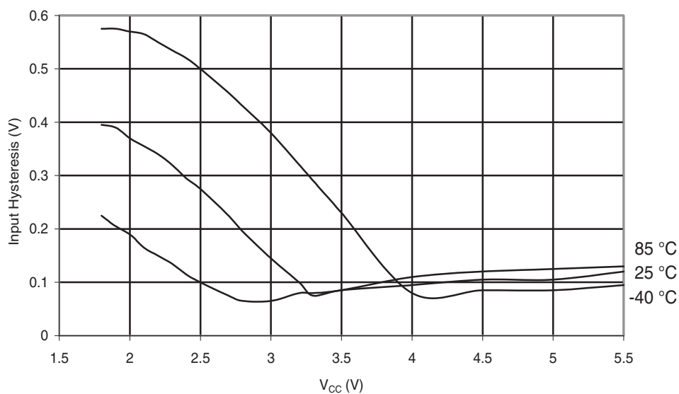
Figure 30-124. ATmega88A: Reset Pin Input Hysteresis vs. V_{CC}
