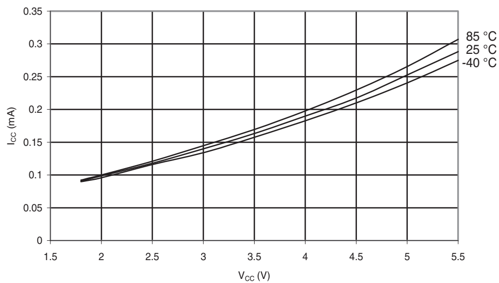
Figure 30-56. ATmega48PA: Idle Supply Current vs. V_{CC} (Internal RC Oscillator, 1MHz)
