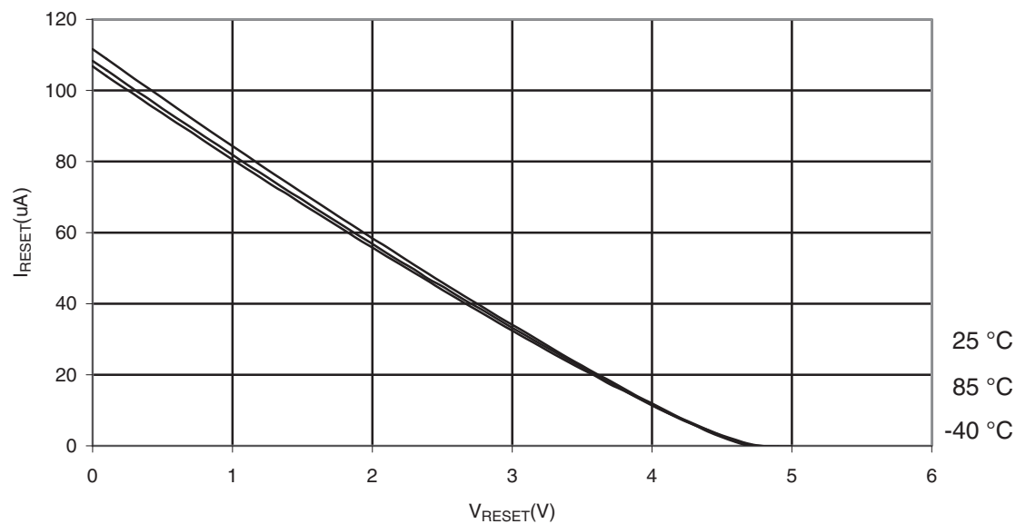
Figure 30-302. ATmega328: Reset Pull-up Resistor Current vs. Reset Pin Voltage ( V_{CC} = 5\text{ V} )
