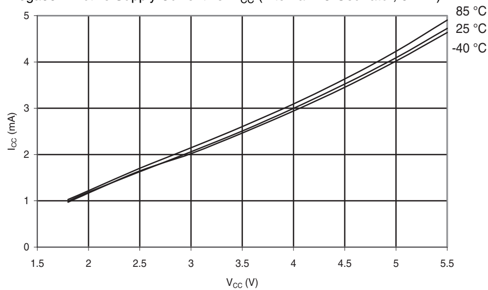
Figure 30-99. ATmega88A: Active Supply Current vs. V_{CC} (Internal RC Oscillator, 8MHz)
