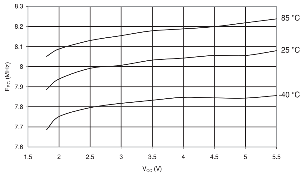
Figure 30-131. ATmega88A: Calibrated 8MHz RC Oscillator Frequency vs. V_{CC}
