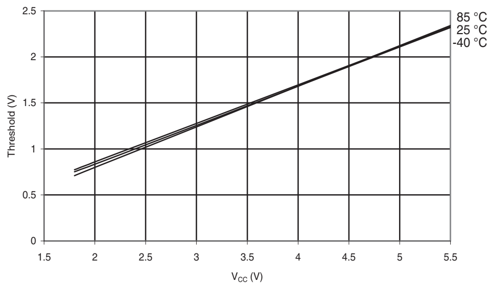
Figure 30-76. ATmega48PA: Reset Input Threshold Voltage vs. V_{CC} ( V_{IL} , I/O Pin read as '0')
