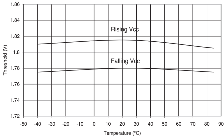
Figure 30-266.ATmega168PA: BOD Thresholds vs. Temperature (BODLEVEL is 1.8 V)
