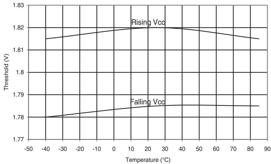
Figure 30-172.ATmega88PA: BOD Thresholds vs. Temperature (BODLEVEL is 1.8 V)
