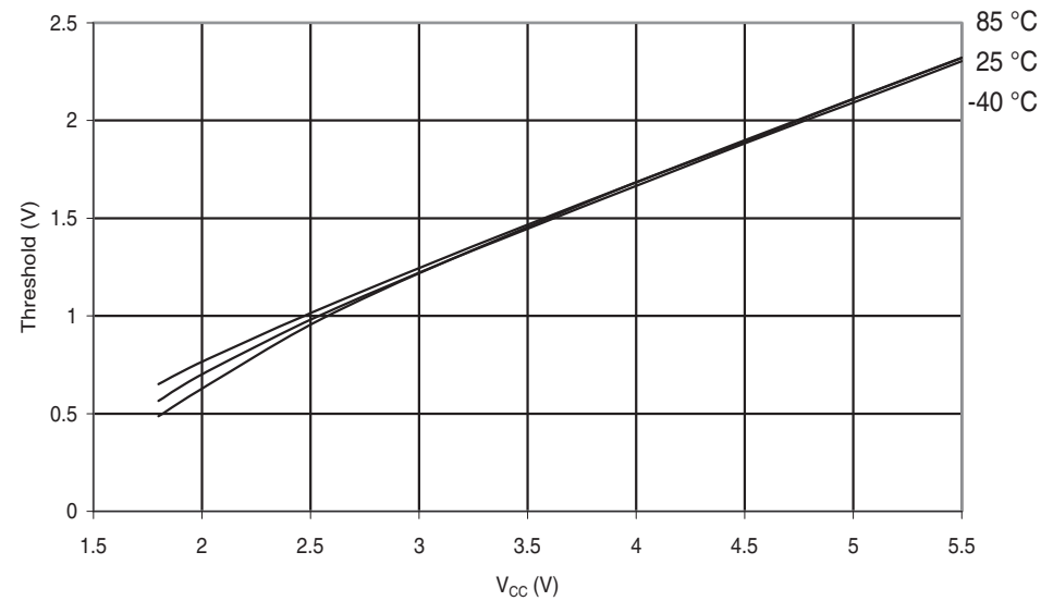
Figure 30-261. ATmega168PA: I/O Pin Input Threshold Voltage vs. V_{CC} ( V_{IL} , I/O Pin read as '0')
