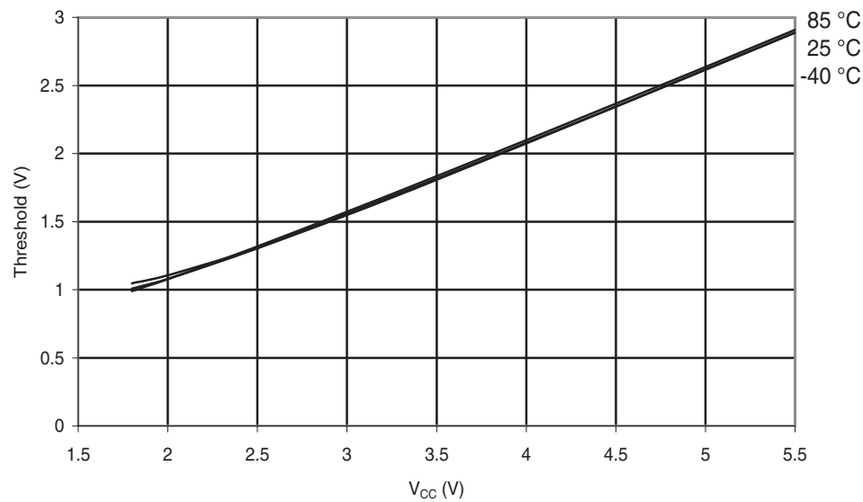
Figure 30-260. ATmega168PA: I/O Pin Input Threshold Voltage vs. V_{CC} ( V_{IH} , I/O Pin read as '1')
