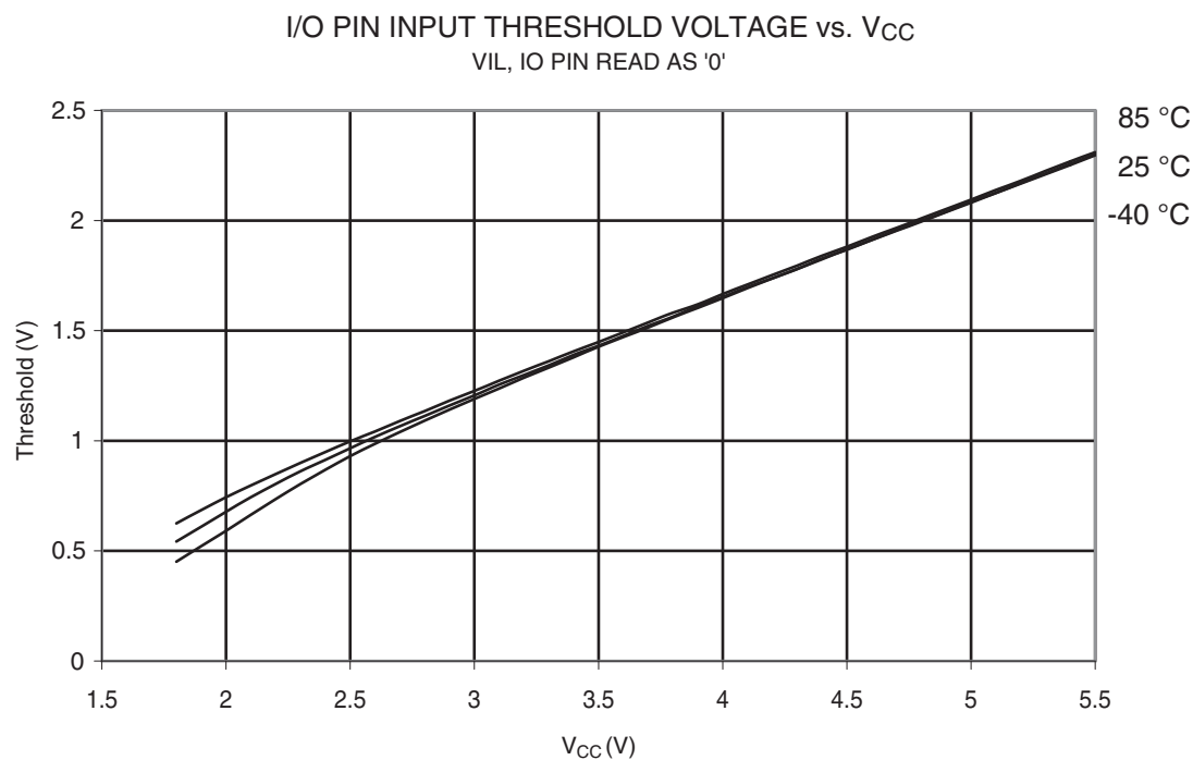
Figure 30-308. ATmega328: I/O Pin Input Threshold Voltage vs. V_{CC} ( V_{IL} , I/O Pin read as '0')
