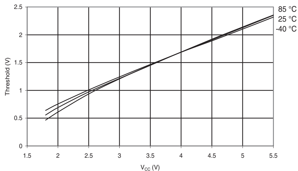
Figure 30-73. ATmega48PA: I/O Pin Input Threshold Voltage vs. V_{CC} ( V_{IL} , I/O Pin read as '0')
