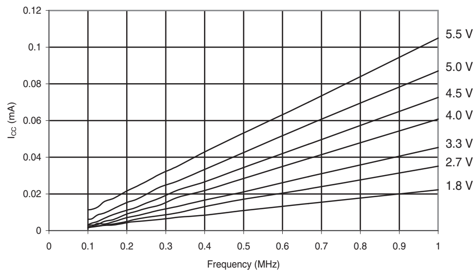
Figure 30-139. ATmega88A: Reset Supply Current vs. Low Frequency (0.1 - 1.0MHz)
