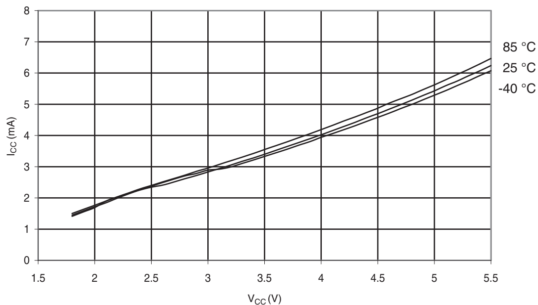
Figure 30-334. ATmega328P: Active Supply Current vs. V_{CC} (Internal RC Oscillator, 8MHz)
