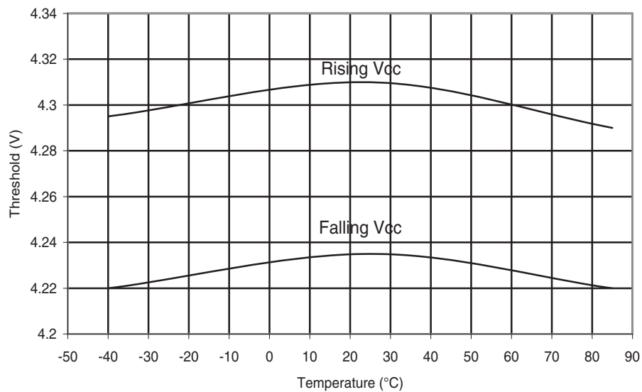
Figure 30-268. ATmega168PA: BOD Thresholds vs. Temperature (BODLEVEL is 4.3 V)
