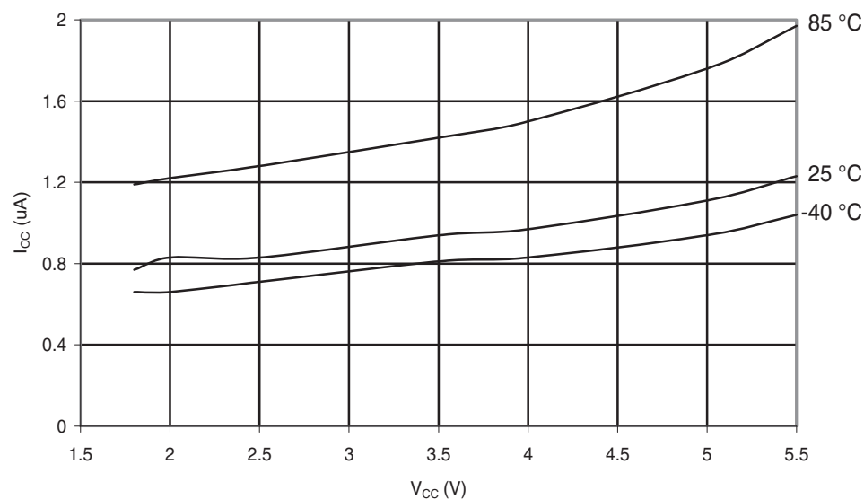
Figure 30-13. ATmega48A: Power-Save Supply Current vs. V_{CC} (Watchdog Timer Disabled and 32kHz Crystal Oscillator Running)
