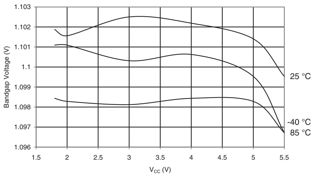
Figure 30-175. ATmega88PA: Bandgap Voltage vs. V_{CC}
