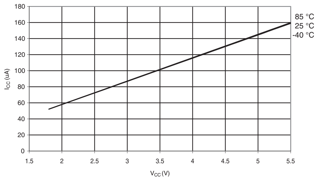
Figure 30-324. ATmega328: AREF External Reference Current vs. V_{CC}
