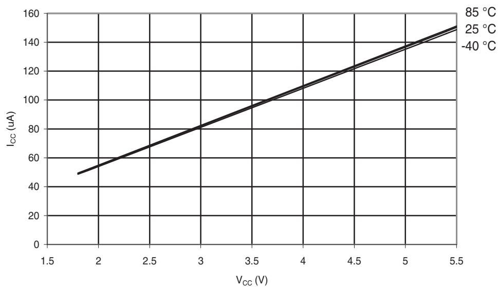
Figure 30-136. ATmega88A: AREF External Reference Current vs. V_{CC}
