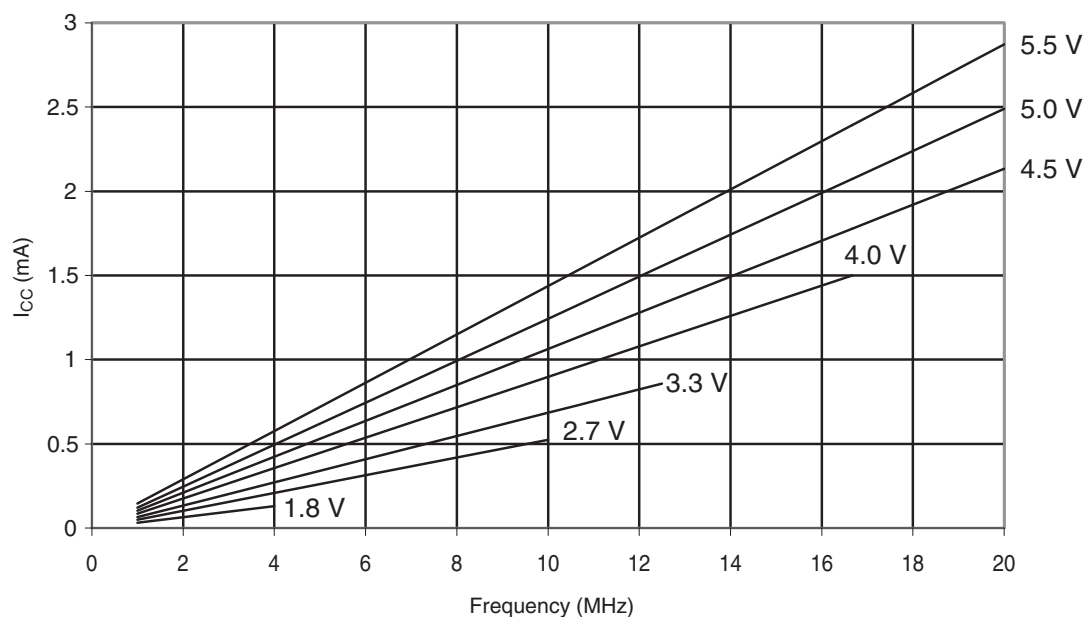
Figure 30-328. ATmega328: Reset Supply Current vs. Frequency (1 - 20MHz)
