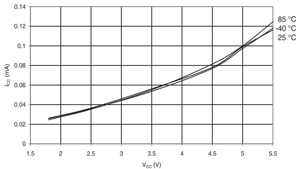
Figure 30-50. ATmega48PA: Active Supply Current vs. V_{CC} (Internal RC Oscillator, 128kHz)
