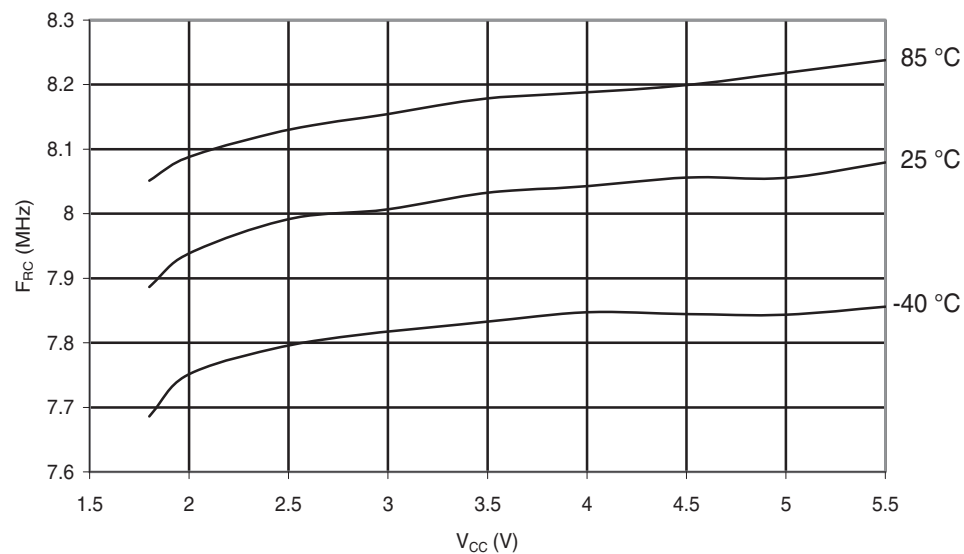
Figure 30-178. ATmega88PA: Calibrated 8MHz RC Oscillator Frequency vs. V_{CC}
