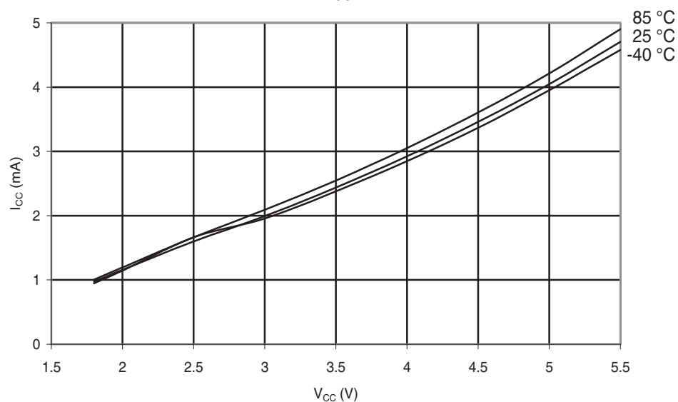
Figure 30-5. ATmega48A: Active Supply Current vs. V_{CC} (Internal RC Oscillator, 8MHz)
