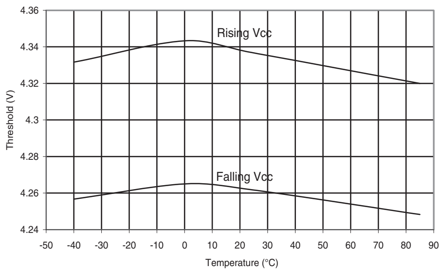
Figure 30-33. ATmega48A: BOD Thresholds vs. Temperature (BODLEVEL is 4.3 V)
