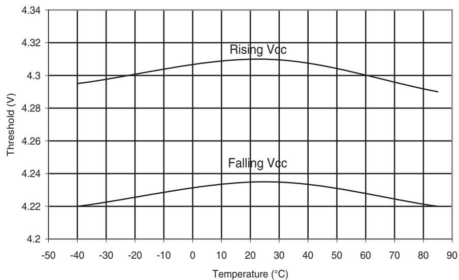
Figure 30-221. ATmega168A: BOD Thresholds vs. Temperature (BODLEVEL is 4.3 V)
