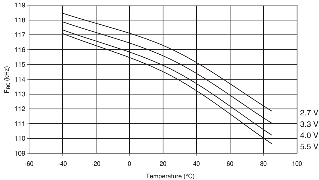
Figure 30-364. ATmega328P: Watchdog Oscillator Frequency vs. Temperature
