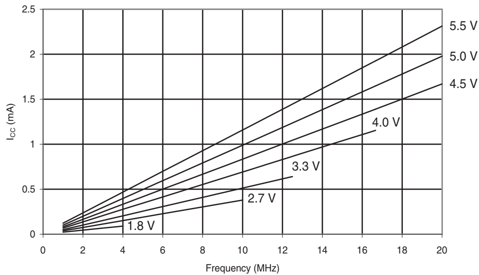
Figure 30-93. ATmega48PA: Reset Supply Current vs. Frequency (1 - 20MHz)
