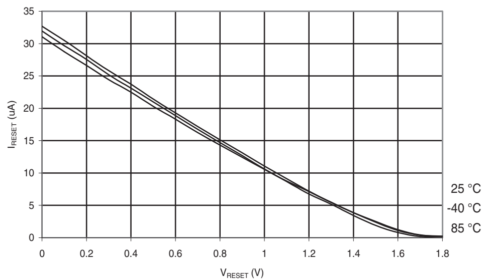
Figure 30-18. ATmega48A: Reset Pull-up Resistor Current vs. Reset Pin Voltage ( V_{CC} = 1.8V )
