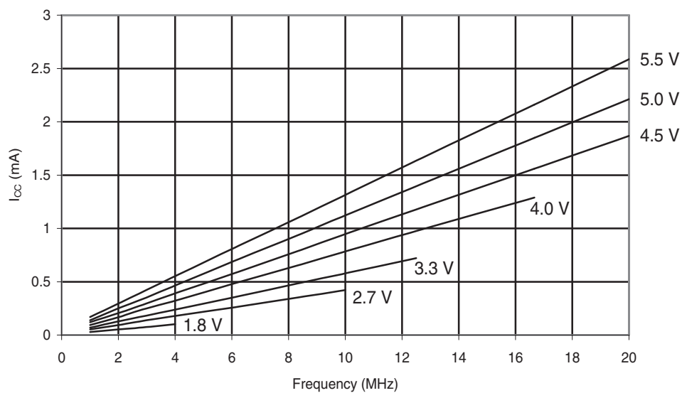
Figure 30-7. ATmega48A: Idle Supply Current vs. Frequency (1-20MHz)
