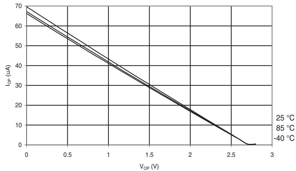
Figure 30-16. ATmega48A: I/O Pin Pull-up Resistor Current vs. Input Voltage ( V_{CC} = 2.7\text{ V} )
