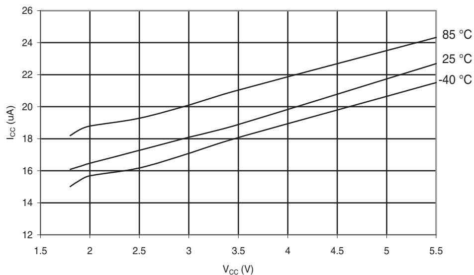
Figure 30-278. ATmega168PA: Brownout Detector Current vs. V_{CC}
