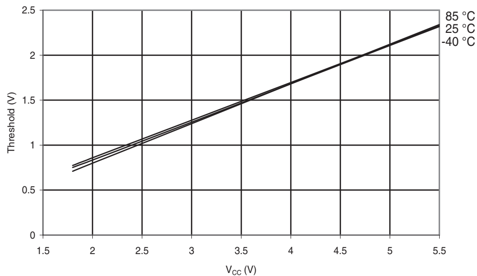
Figure 30-29. )ATmega48A: Reset Input Threshold Voltage vs. V_{CC} ( V_{IL} , I/O Pin read as '0')
