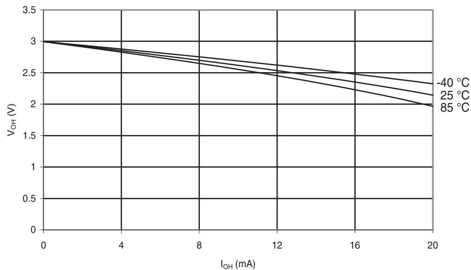
Figure 30-23. ATmega48A: I/O Pin Output Voltage vs. Source Current ( V_{CC} = 3\text{ V} )
