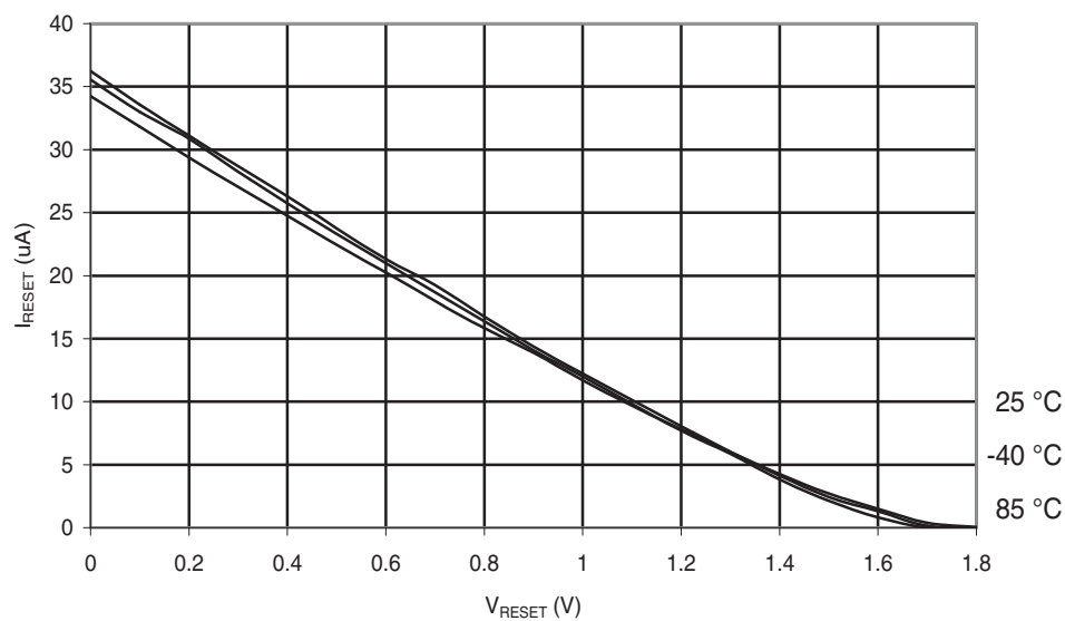
Figure 30-159. ATmega88PA: Reset Pull-up Resistor Current vs. Reset Pin Voltage ( V_{CC} = 1.8\text{ V} )
