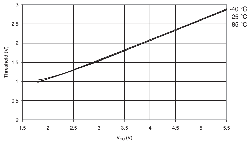
Figure 30-72. ATmega48PA: I/O Pin Input Threshold Voltage vs. V_{CC} ( V_{IH} , I/O Pin read as '1')
