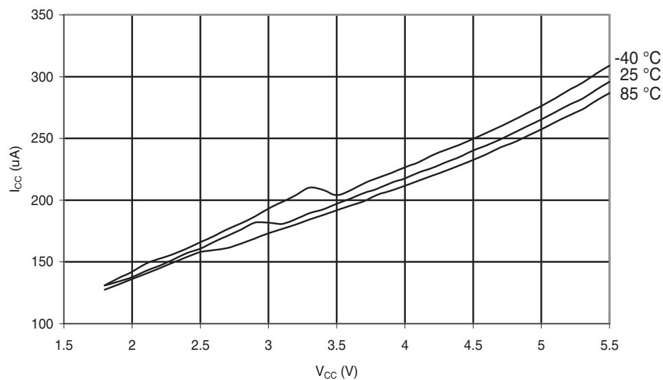
Figure 30-275. ATmega168PA: ADC Current vs. V_{CC} (AREF = AV_{CC} )
