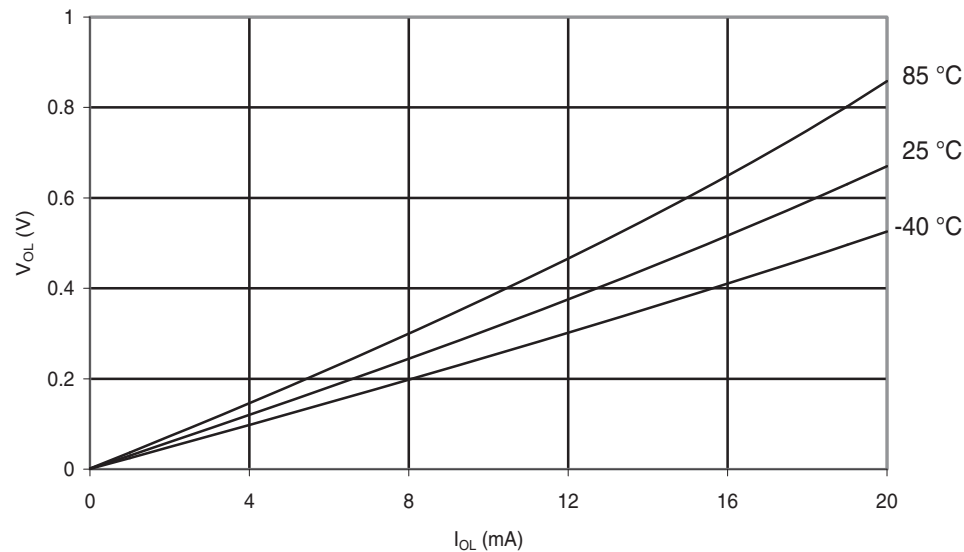
Figure 30-115. ATmega88A: I/O Pin Output Voltage vs. Sink Current ( V_{CC} = 3\text{ V} )
