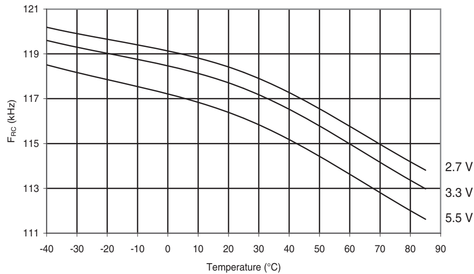
Figure 30-270.ATmega168PA: Watchdog Oscillator Frequency vs. Temperature
