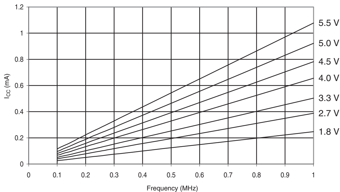
Figure 30-330. ATmega328P: Active Supply Current vs. Low Frequency (0.1-1.0MHz)
