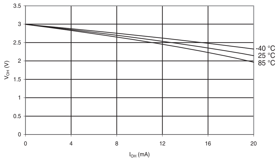
Figure 30-70. ATmega48PA: I/O Pin Output Voltage vs. Source Current ( V_{CC} = 3\text{ V} )
