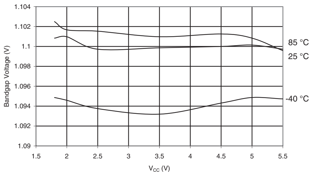
Figure 30-34. ATmega48A: Bandgap Voltage vs. V_{CC}
