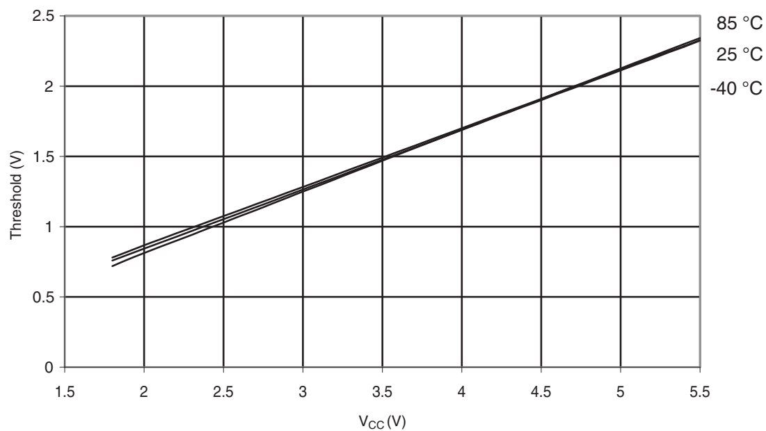
Figure 30-358. ATmega328P: Reset Input Threshold Voltage vs. V_{CC} ( V_{IL} , I/O Pin read as '0')
