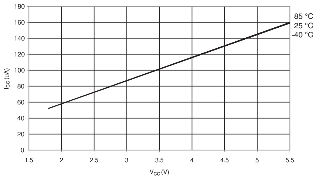
Figure 30-371. ATmega328P: AREF External Reference Current vs. V_{CC}
