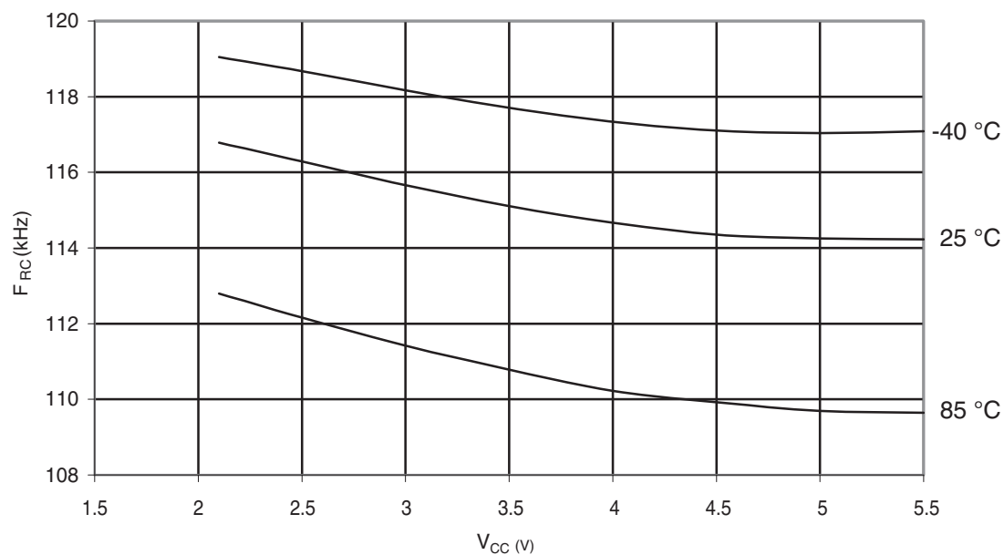
Figure 30-318. ATmega328: Watchdog Oscillator Frequency vs. V_{CC}
