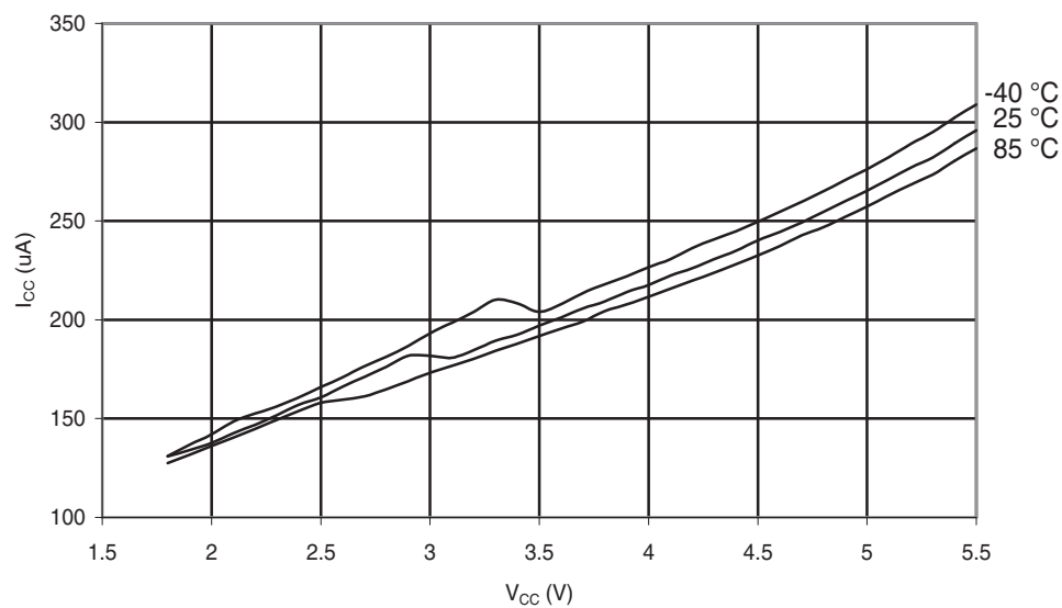
Figure 30-228. ATmega168A: ADC Current vs. V_{CC} ( A_{REF} = A_{V_{CC}} )
