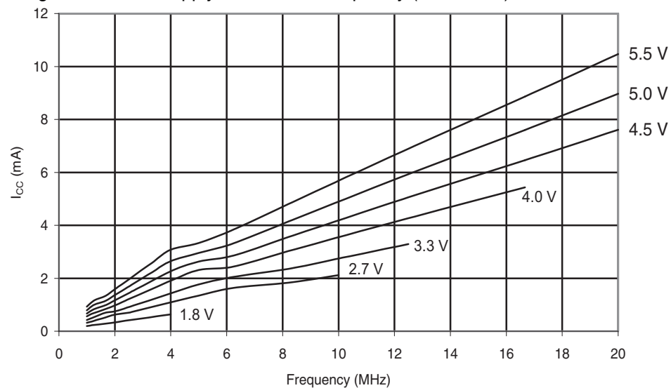
Figure 30-96. ATmega88A: Active Supply Current vs. Frequency (1 - 20MHz)
