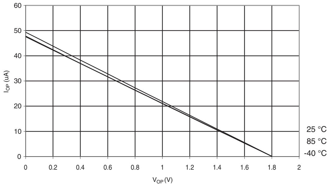
Figure 30-344. ATmega328P: I/O Pin Pull-up Resistor Current vs. Input Voltage ( V_{CC} = 1.8\text{ V} )
