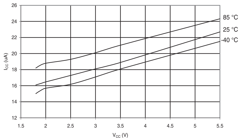
Figure 30-232. ATmega168A: Programming Current vs. V_{CC}
