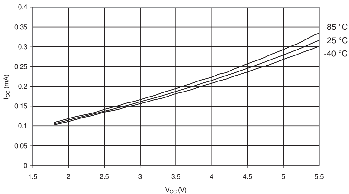
Figure 30-291. ATmega328: Idle Supply Current vs. V_{CC} (Internal RC Oscillator, 1MHz)
