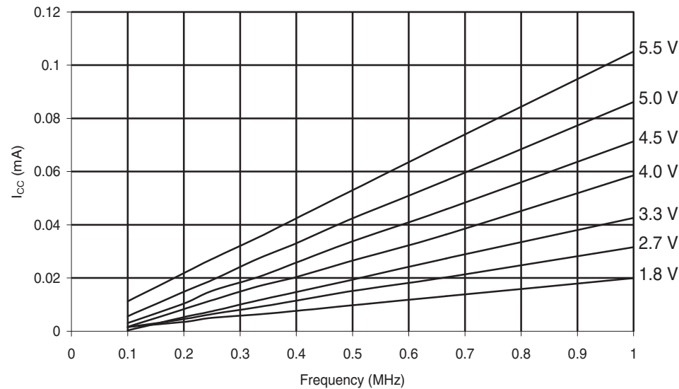
Figure 30-233.ATmega168A: Reset Supply Current vs. Low Frequency (0.1 - 1.0MHz)
