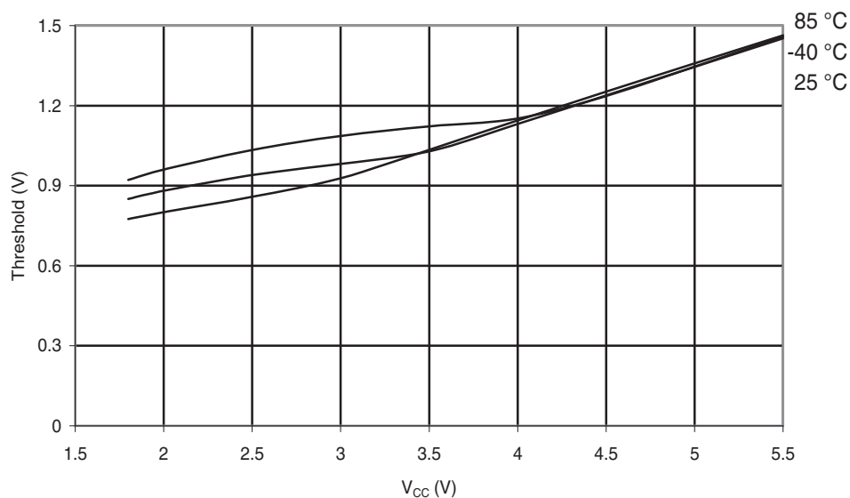
Figure 30-263. ATmega168PA: Reset Input Threshold Voltage vs. V_{CC} ( V_{IH} , I/O Pin read as '1')
