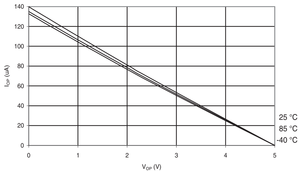
Figure 30-111. ATmega88A: I/O Pin Pull-up Resistor Current vs. Input Voltage ( V_{CC} = 5\text{ V} )
