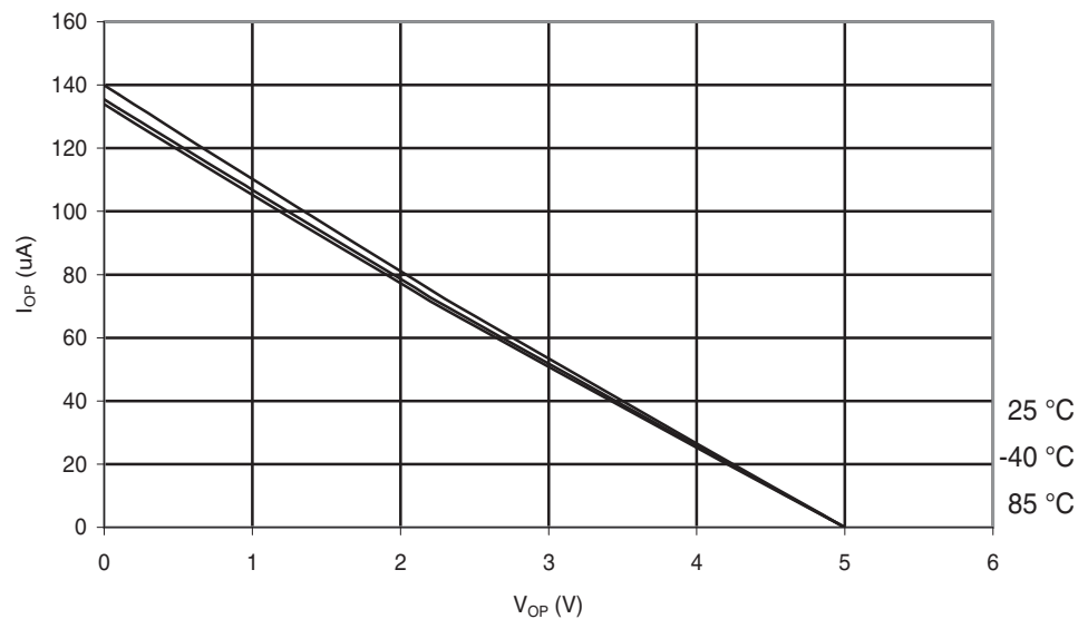
Figure 30-205. ATmega168A: I/O Pin Pull-up Resistor Current vs. Input Voltage ( V_{CC} = 5\text{ V} )
