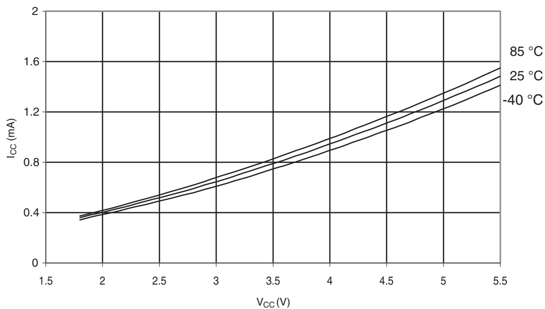
Figure 30-339. ATmega328P: Idle Supply Current vs. V_{CC} (Internal RC Oscillator, 8MHz)
