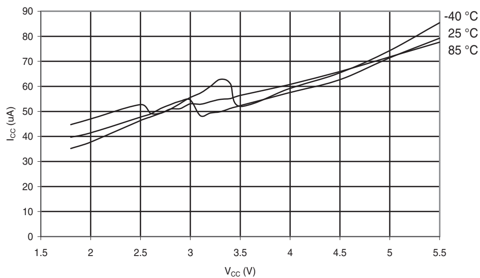
Figure 30-135. ATmega88A: Analog Comparator Current vs. V_{CC}
