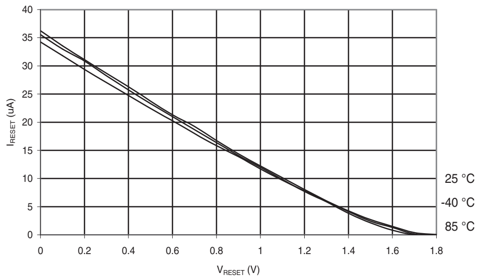
Figure 30-112. ATmega88A: Reset Pull-up Resistor Current vs. Reset Pin Voltage ( V_{CC} = 1.8\text{ V} )
