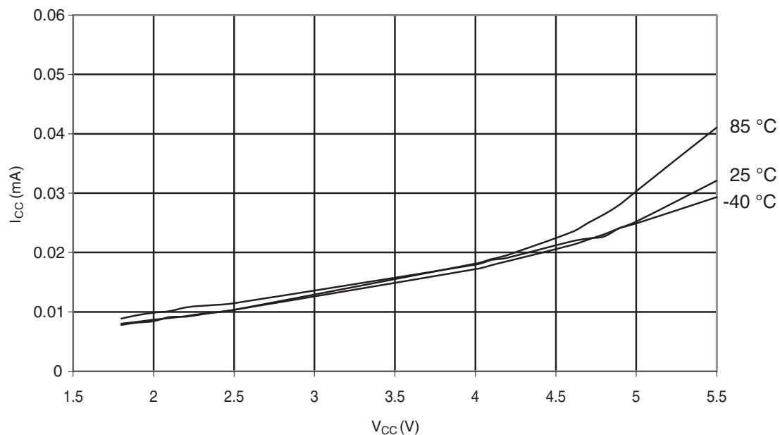
Figure 30-290. ATmega328: Idle Supply Current vs. V_{CC} (Internal RC Oscillator, 128kHz)
