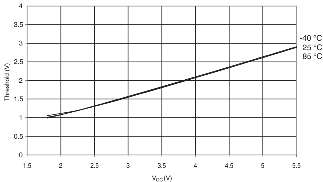
Figure 30-307. ATmega328: I/O Pin Input Threshold Voltage vs. V_{CC} ( V_{IH} , I/O Pin read as '1')
