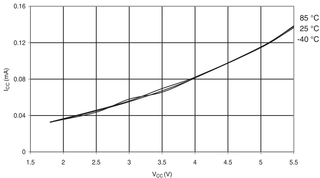
Figure 30-285. ATmega328: Active Supply Current vs. V_{CC} (Internal RC Oscillator, 128kHz)
