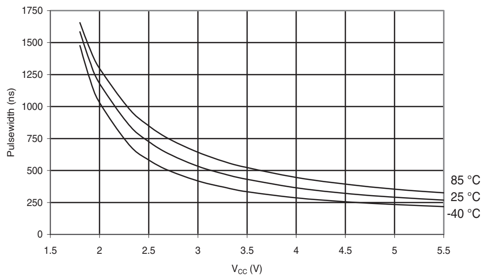
Figure 30-282. ATmega168PA: Minimum Reset Pulse width vs. V_{CC}
