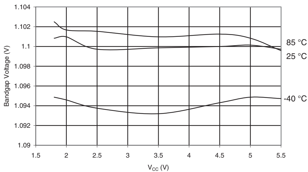
Figure 30-81. ATmega48PA: Bandgap Voltage vs. V_{CC}
