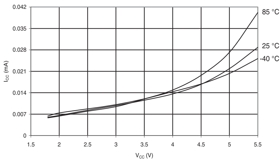
Figure 30-55. ATmega48PA: Idle Supply Current vs. V_{CC} (Internal RC Oscillator, 128kHz)
