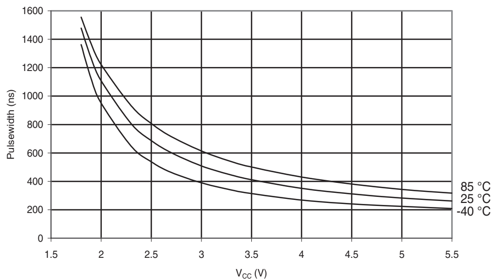
Figure 30-94. ATmega48PA: Minimum Reset Pulse width vs. V_{CC}
