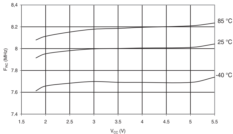
Figure 30-272. ATmega168PA: Calibrated 8MHz RC Oscillator Frequency vs. V_{CC}
