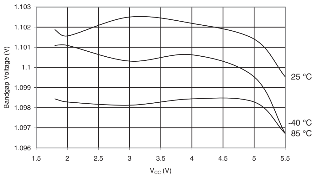
Figure 30-128. ATmega88A: Bandgap Voltage vs. V_{CC}
