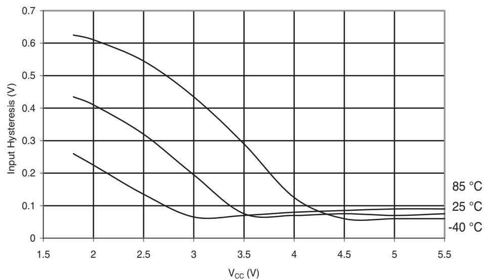
Figure 30-265. ATmega168PA: Reset Pin Input Hysteresis vs. V_{CC}
