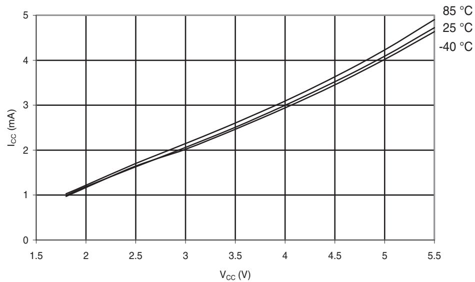
Figure 30-146. ATmega88PA: Active Supply Current vs. V_{CC} (Internal RC Oscillator, 8MHz)
