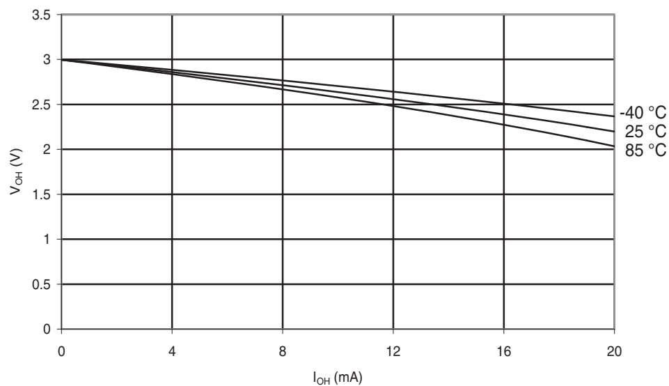
Figure 30-164. ATmega88PA: I/O Pin Output Voltage vs. Source Current ( V_{CC} = 3\text{ V} )
