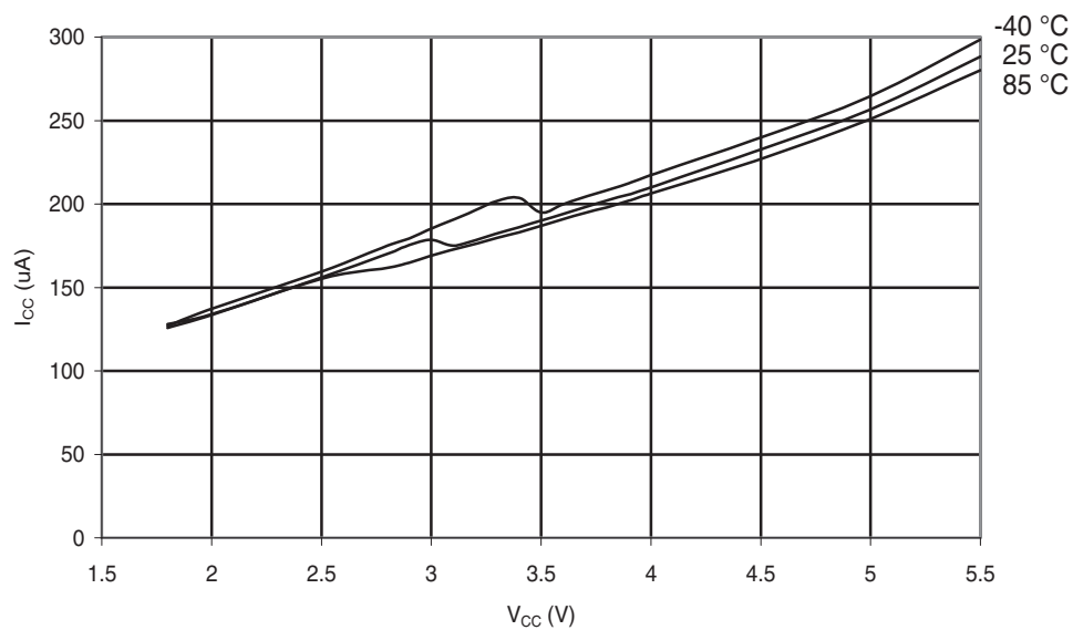
Figure 30-134. ATmega88A: ADC Current vs. V_{CC} (AREF = AV_{CC} )
