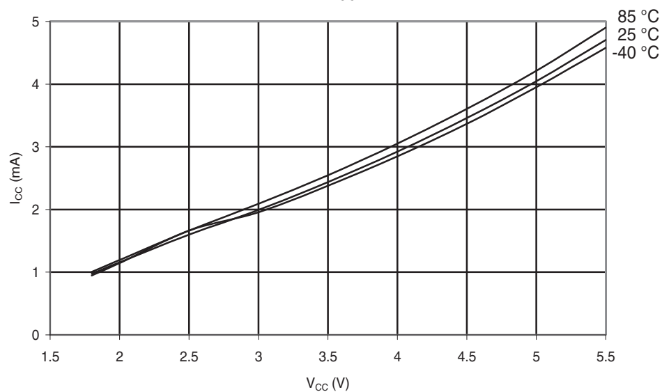
Figure 30-52. ATmega48PA: Active Supply Current vs. V_{CC} (Internal RC Oscillator, 8MHz)
