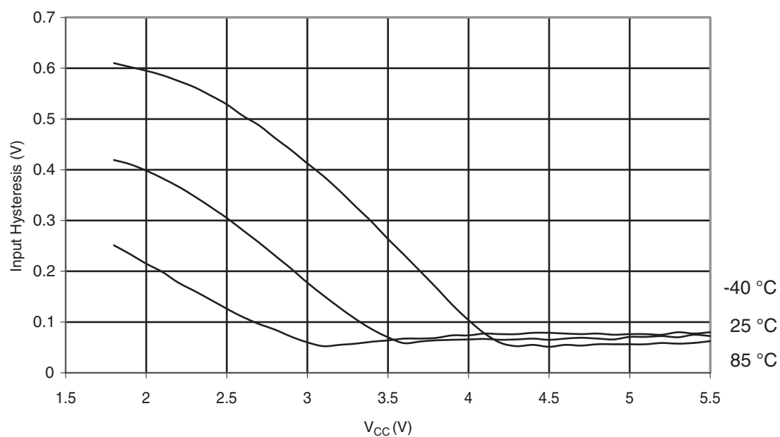
Figure 30-359. ATmega328P: Reset Pin Input Hysteresis vs. V_{CC}
