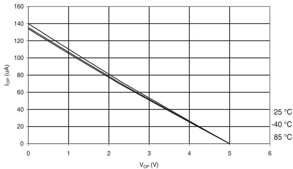
Figure 30-252. ATmega168PA: I/O Pin Pull-up Resistor Current vs. Input Voltage ( V_{CC} = 5\text{ V} )
