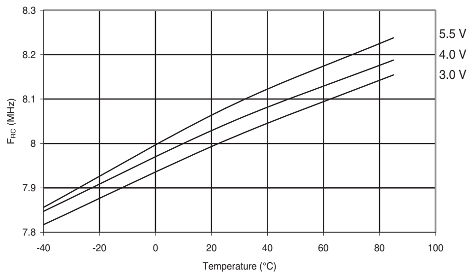
Figure 30-179. ATmega88PA: Calibrated 8MHz RC Oscillator Frequency vs. Temperature
