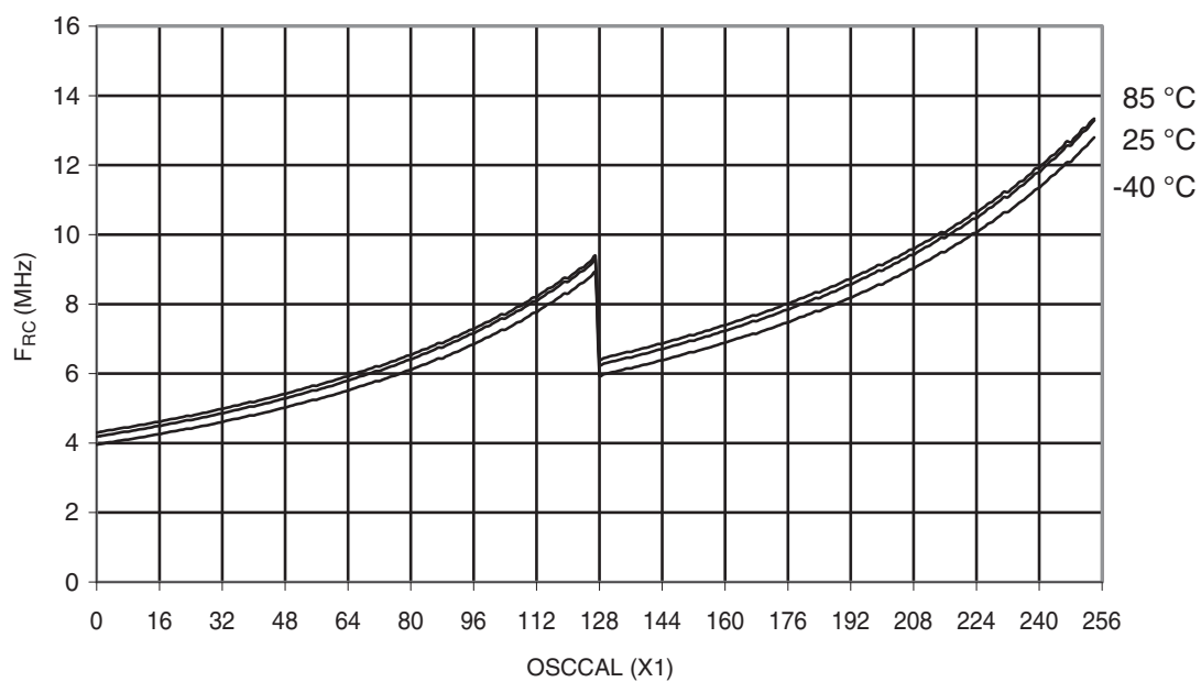
Figure 30-321. ATmega328: Calibrated 8MHz RC Oscillator Frequency vs. OSCCAL Value
