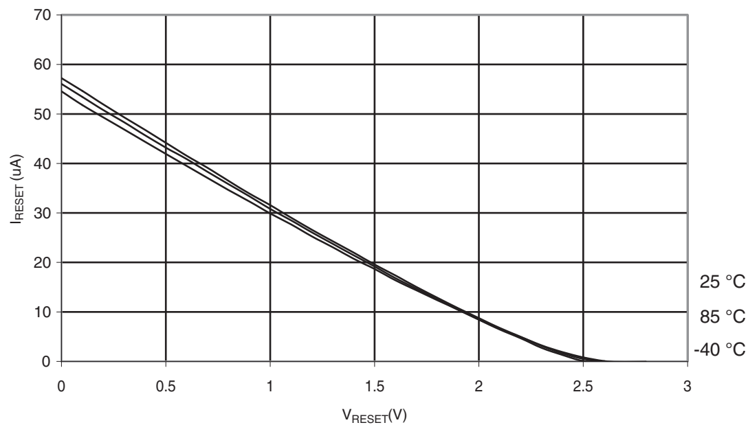
Figure 30-301. ATmega328: Reset Pull-up Resistor Current vs. Reset Pin Voltage ( V_{CC} = 2.7\text{ V} )
