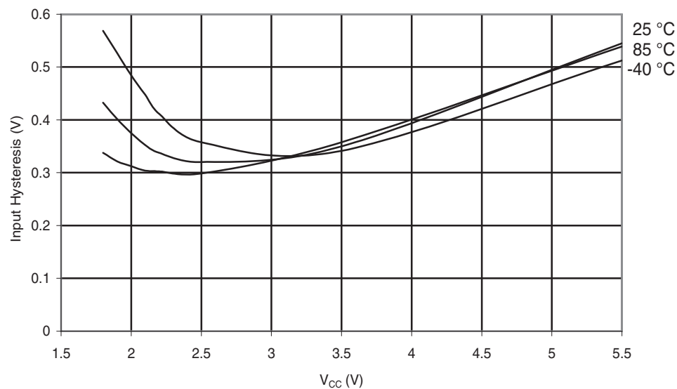
Figure 30-27. ATmega48A: I/O Pin Input Hysteresis vs. V_{CC}
