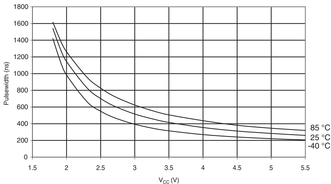
Figure 30-329. ATmega328: Minimum Reset Pulse width vs. V_{CC}
