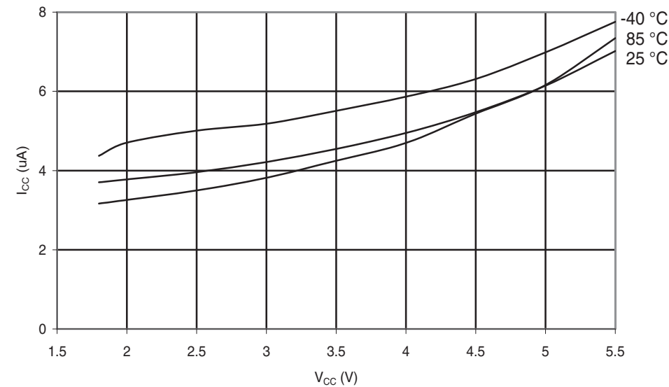
Figure 30-200.ATmega168A: Power-Down Supply Current vs. V CC (Watchdog Timer Enabled)
