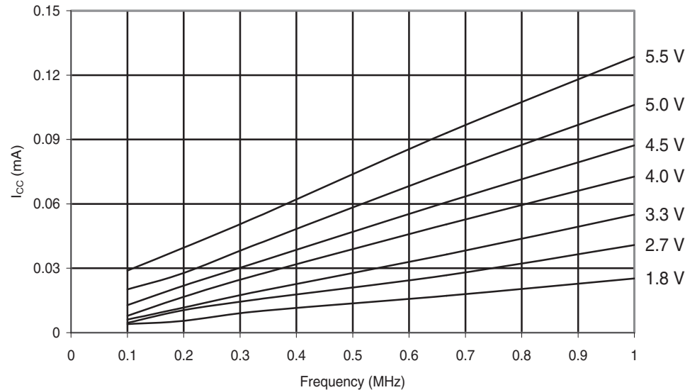
Figure 30-100.ATmega88A: Idle Supply Current vs. Low Frequency (0.1-1.0MHz)
