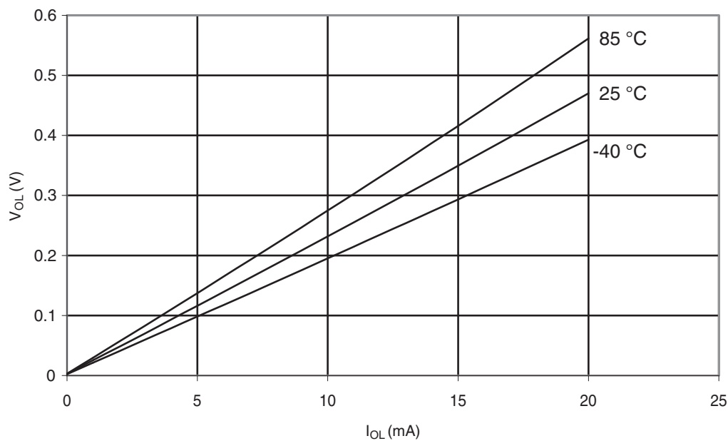
Figure 30-351. ATmega328P: I/O Pin Output Voltage vs. Sink Current ( V_{CC} = 5\text{ V} )
