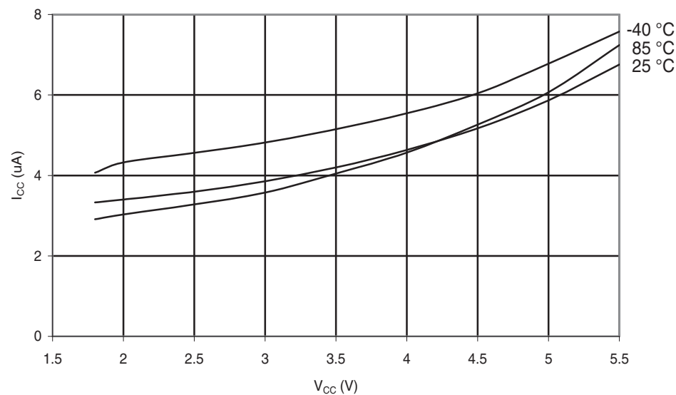
Figure 30-12. ATmega48A: Power-Down Supply Current vs. V_{CC} (Watchdog Timer Enabled)
