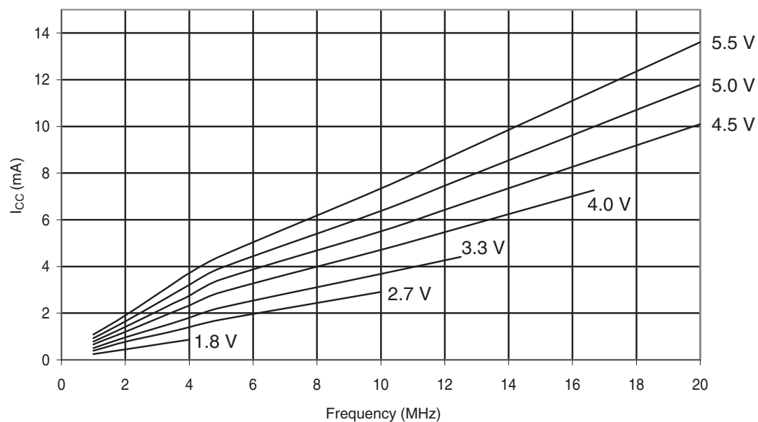
Figure 30-284. ATmega328: Active Supply Current vs. Frequency (1-20MHz)
