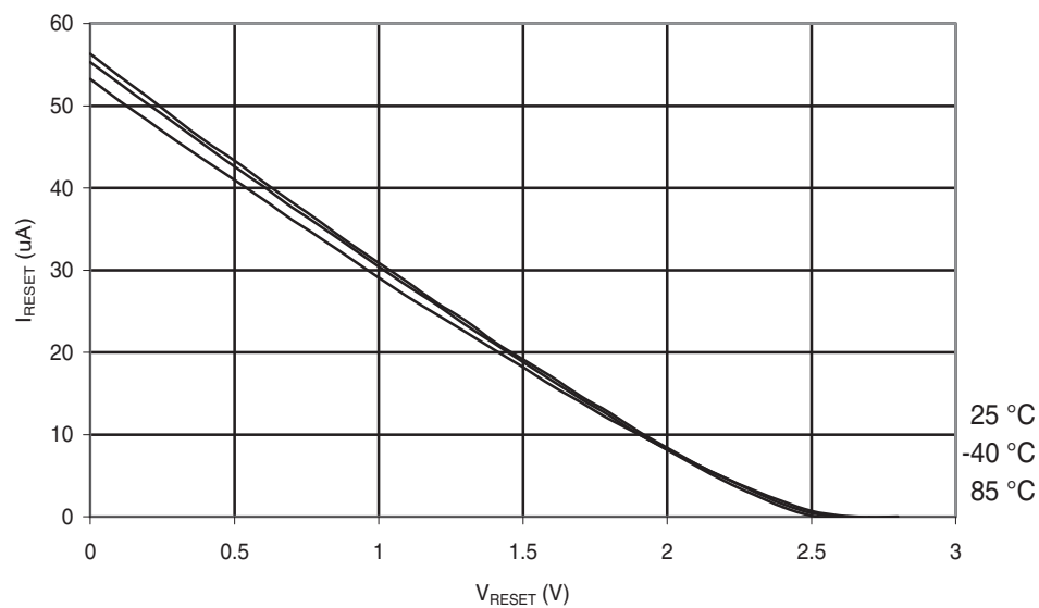
Figure 30-254. ATmega168PA: Reset Pull-up Resistor Current vs. Reset Pin Voltage ( V_{CC} = 2.7\text{ V} )
