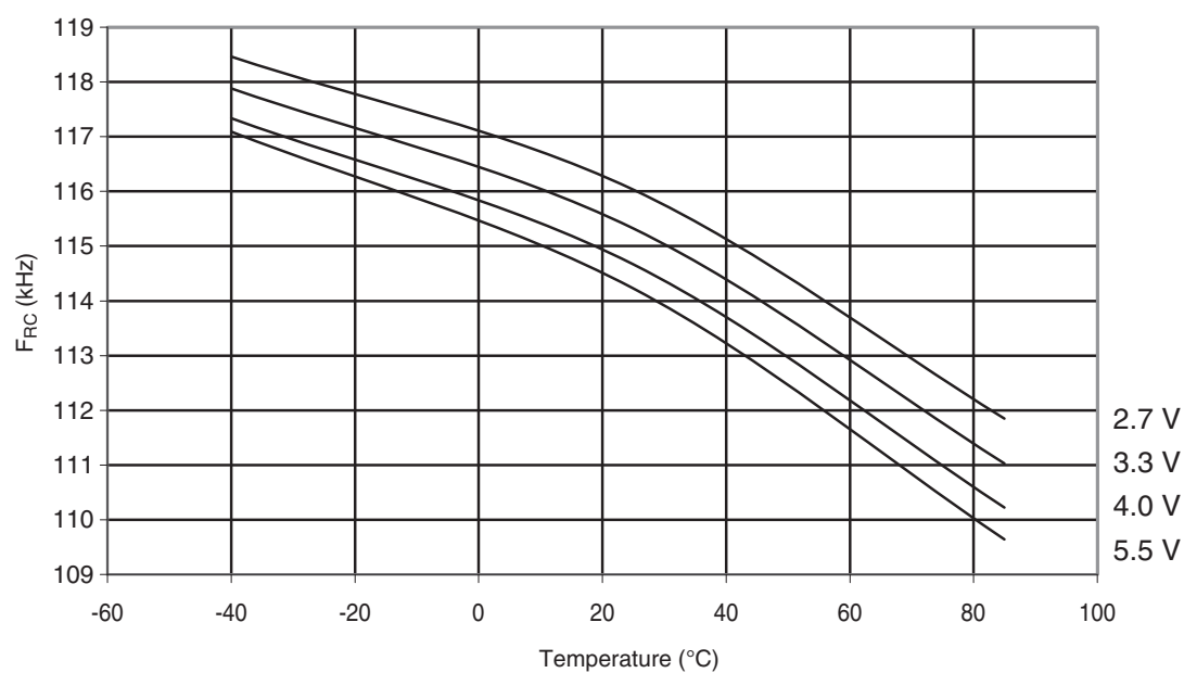
Figure 30-317. ATmega328: Watchdog Oscillator Frequency vs. Temperature
