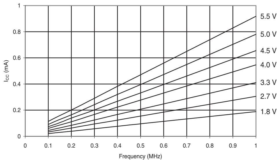
Figure 30-48. ATmega48PA: Active Supply Current vs. Low Frequency (0.1-1.0MHz)
