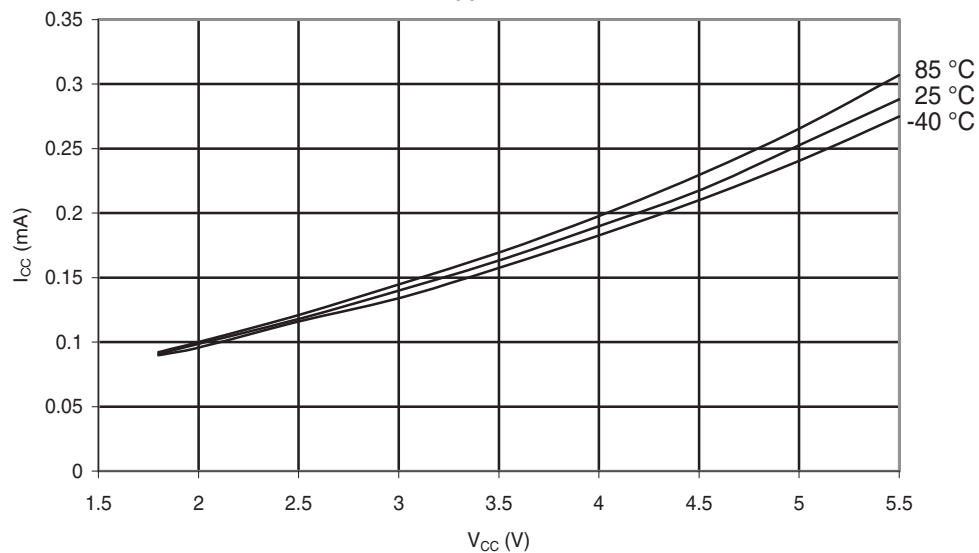
Figure 30-9. ATmega48A: Idle Supply Current vs. V_{CC} (Internal RC Oscillator, 1MHz)
