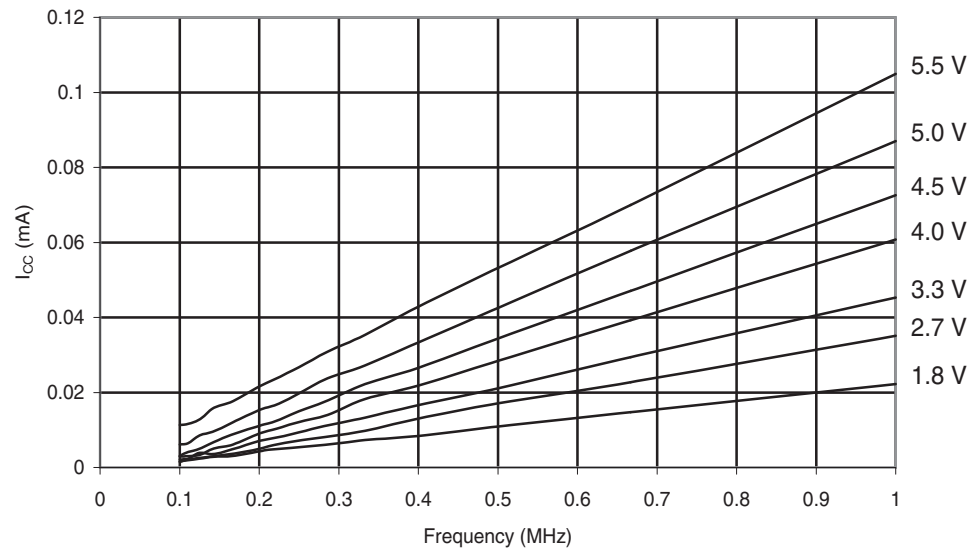
Figure 30-186.ATmega88PA: Reset Supply Current vs. Low Frequency (0.1 - 1.0MHz)
