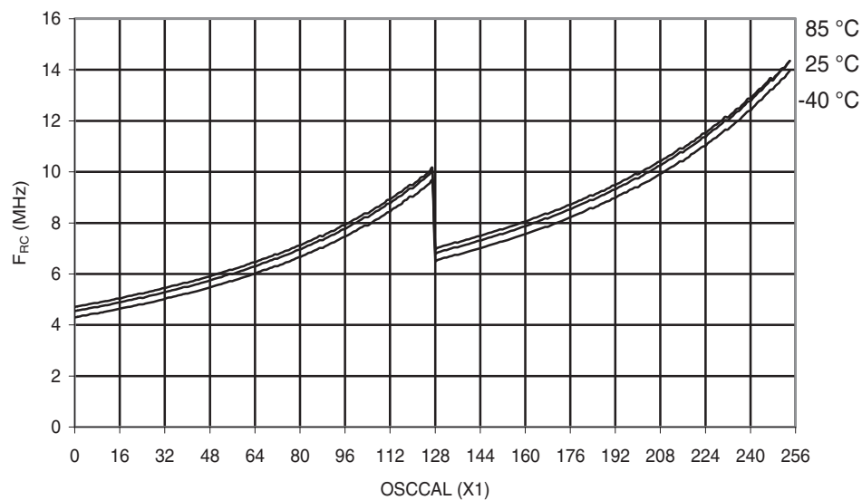
Figure 30-274. ATmega168PA: Calibrated 8MHz RC Oscillator Frequency vs. OSCCAL Value
