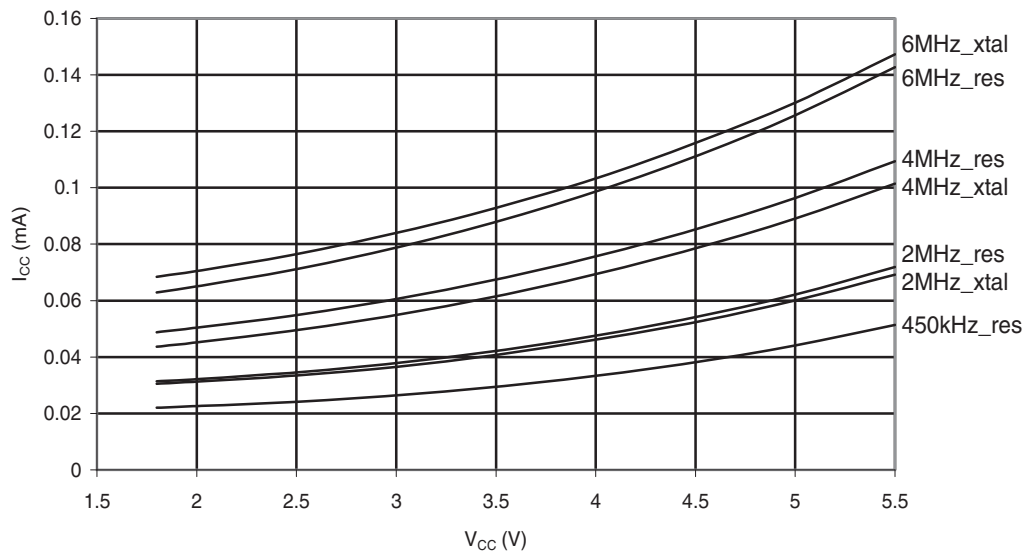
Figure 30-61. ATmega48PA: Standby Supply Current vs. V_{CC} (Watchdog Timer Disabled)
