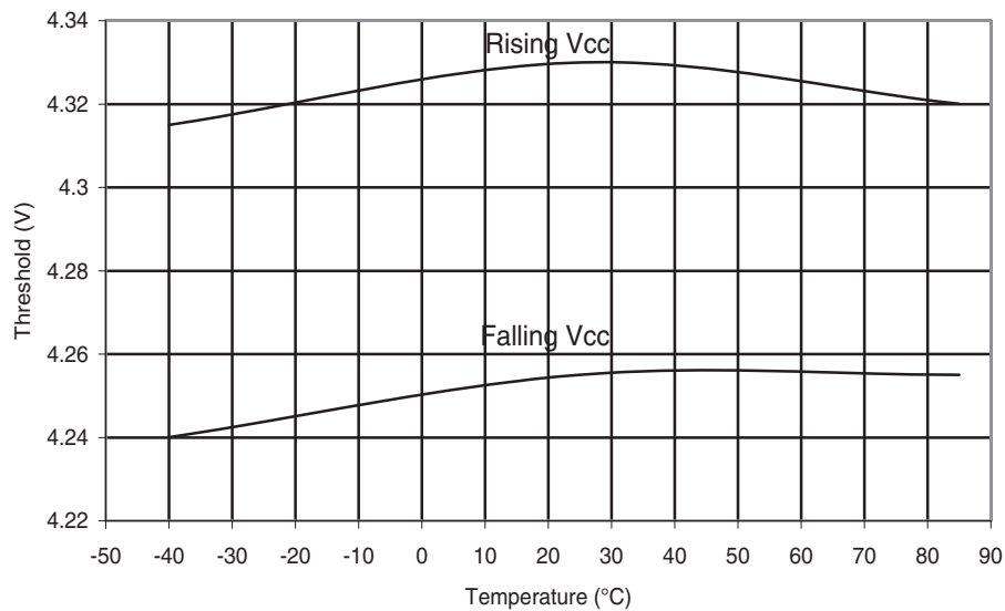
Figure 30-127. ATmega88A: BOD Thresholds vs. Temperature (BODLEVEL is 4.3 V)
