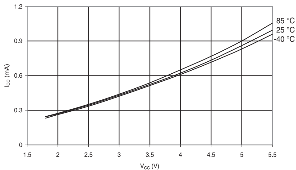
Figure 30-151. ATmega88PA: Idle Supply Current vs. V CC (Internal RC Oscillator, 8MHz)
