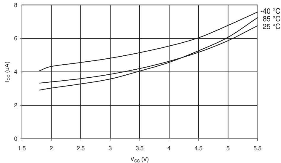
Figure 30-59. ATmega48PA: Power-Down Supply Current vs. V_{CC} (Watchdog Timer Enabled)
