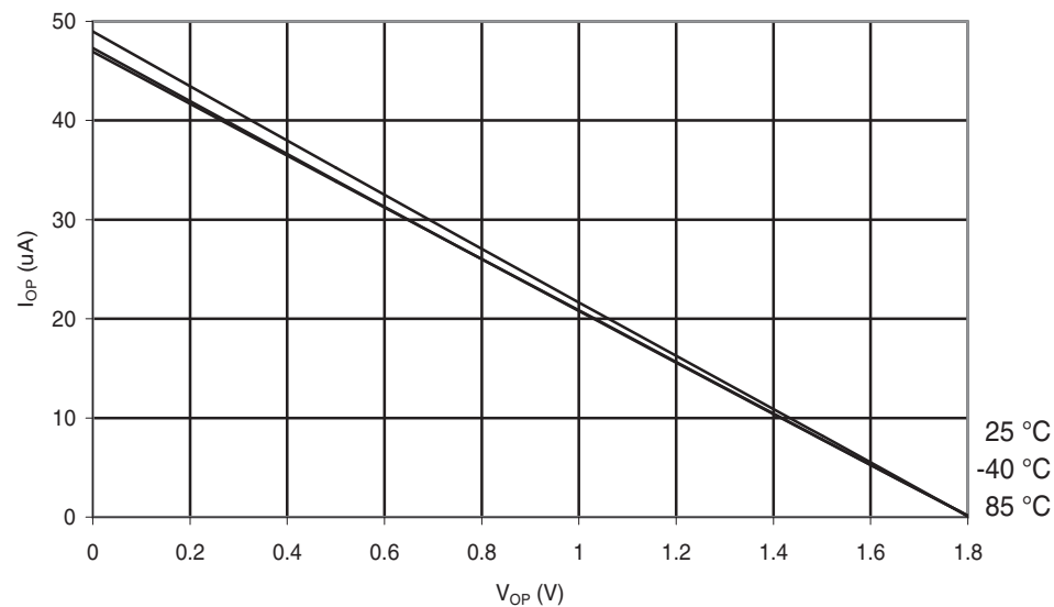
Figure 30-109.ATmega88A: I/O Pin Pull-up Resistor Current vs. Input Voltage ( V_{CC} = 1.8\text{ V} )
