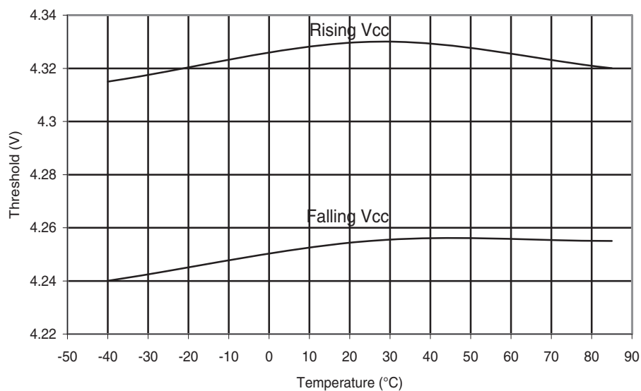
Figure 30-174. ATmega88PA: BOD Thresholds vs. Temperature (BODLEVEL is 4.3 V)
