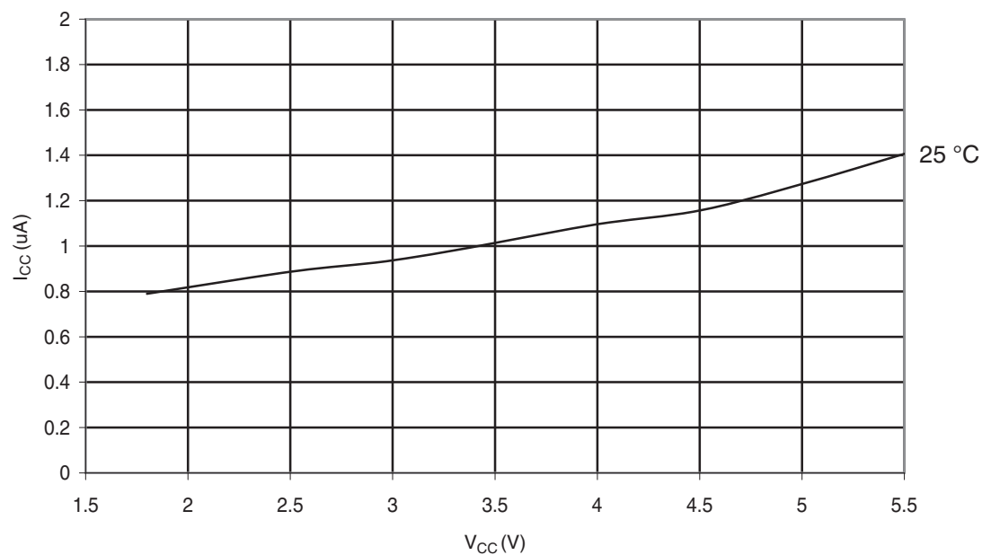
Figure 30-295. ATmega328: Power-Save Supply Current vs. V_{CC} (Watchdog Timer Disabled and 32kHz Crystal Oscillator Running)
