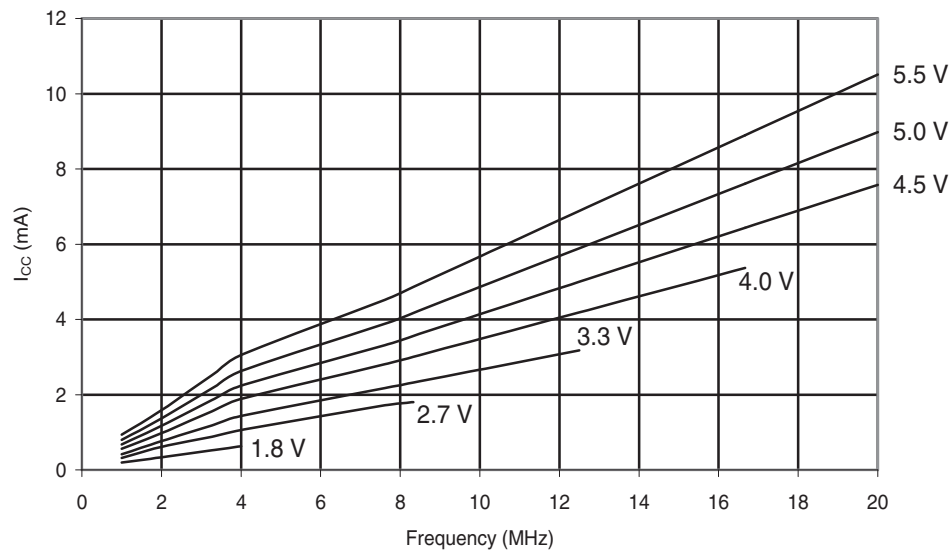
Figure 30-2. ATmega48A: Active Supply Current vs. Frequency (1-20MHz)
