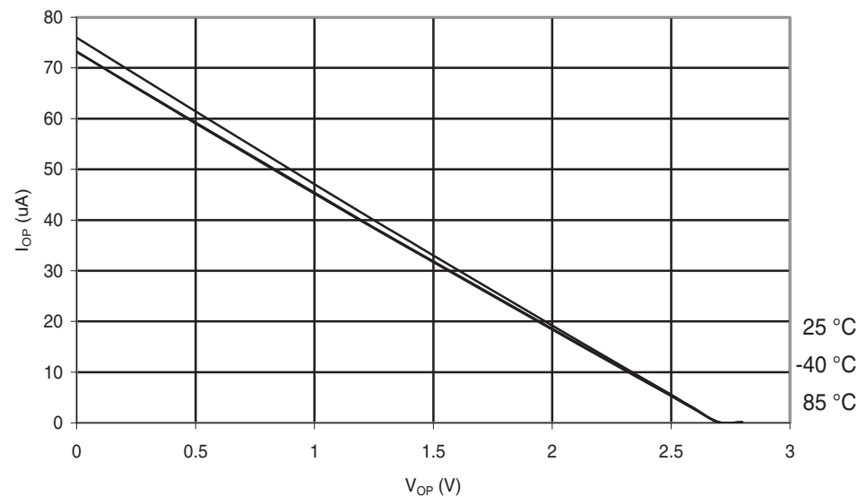
Figure 30-251.ATmega168PA: I/O Pin Pull-up Resistor Current vs. Input Voltage ( V_{CC} = 2.7\text{ V} )
