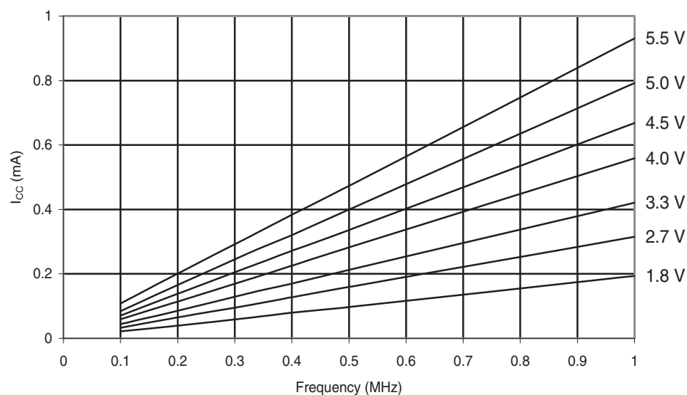
Figure 30-142. ATmega88PA: Active Supply Current vs. Low Frequency (0.1-1.0MHz)
