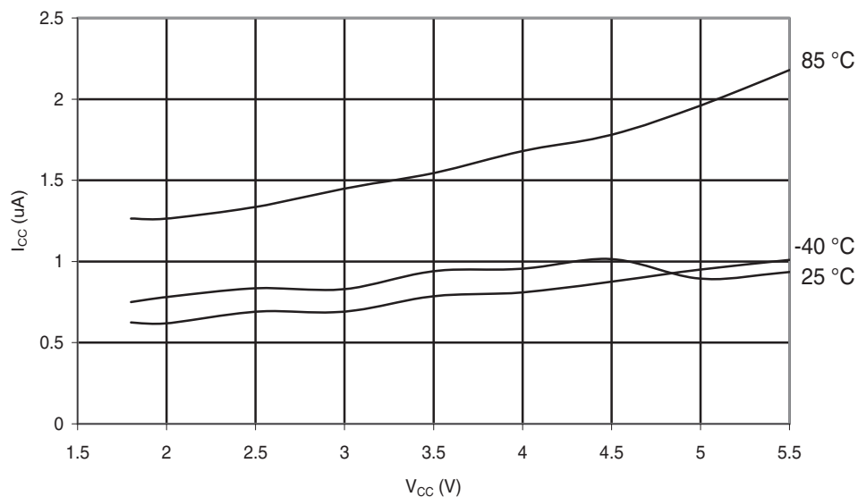
Figure 30-201. ATmega168A: Power-Save Supply Current vs. V_{CC} (Watchdog Timer Disabled and 32kHz Crystal Oscillator Running)
