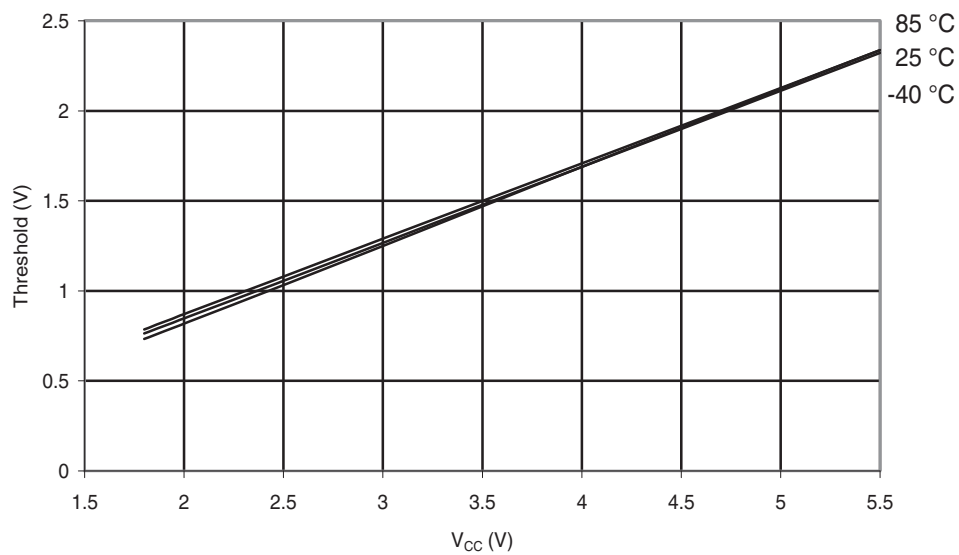
Figure 30-123. ATmega88A: Reset Input Threshold Voltage vs. V_{CC} ( V_{IL} , I/O Pin read as '0')
