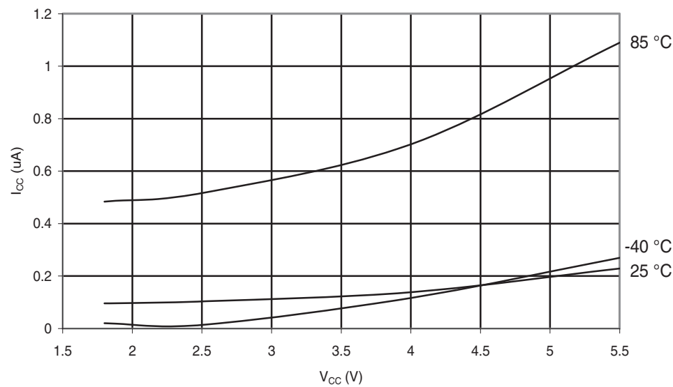
Figure 30-11. ATmega48A: Power-Down Supply Current vs. V_{CC} (Watchdog Timer Disabled)
