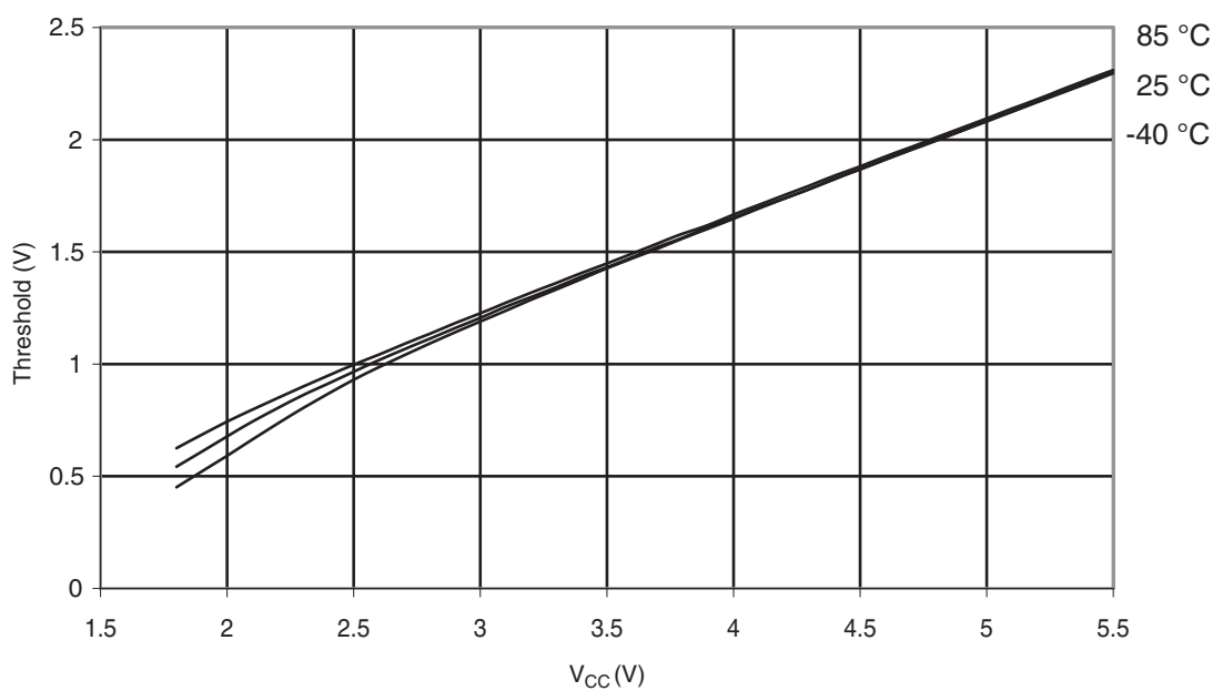
Figure 30-355. ATmega328P: I/O Pin Input Threshold Voltage vs. V_{CC} ( V_{IL} , I/O Pin read as '0')
