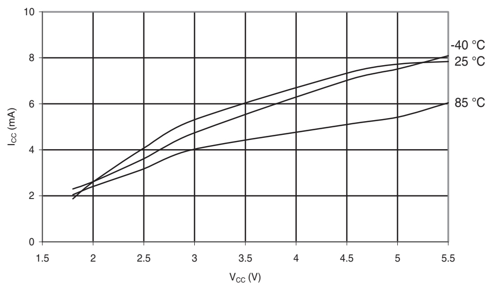
Figure 30-232. ATmega168A: Programming Current vs. V_{CC}
