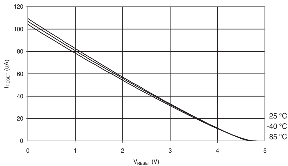
Figure 30-255. ATmega168PA: Reset Pull-up Resistor Current vs. Reset Pin Voltage ( V_{CC} = 5\text{ V} )
