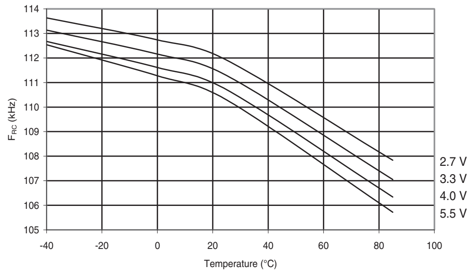
Figure 30-129.ATmega88A: Watchdog Oscillator Frequency vs. Temperature
