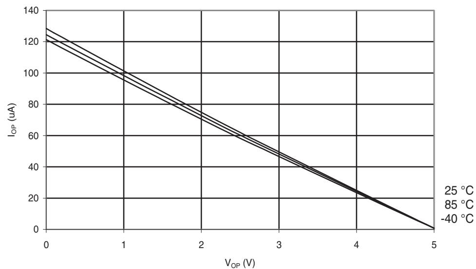
Figure 30-17. ATmega48A: I/O Pin Pull-up Resistor Current vs. Input Voltage ( V_{CC} = 5V )
