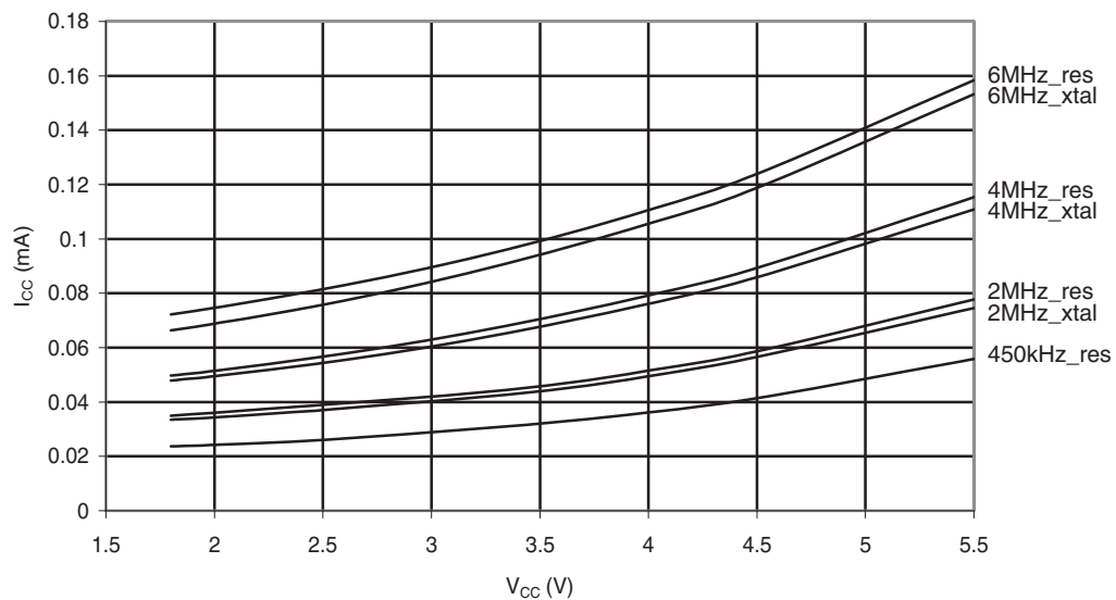
Figure 30-108. ATmega88A: Standby Supply Current vs. V_{CC} (Watchdog Timer Disabled)
