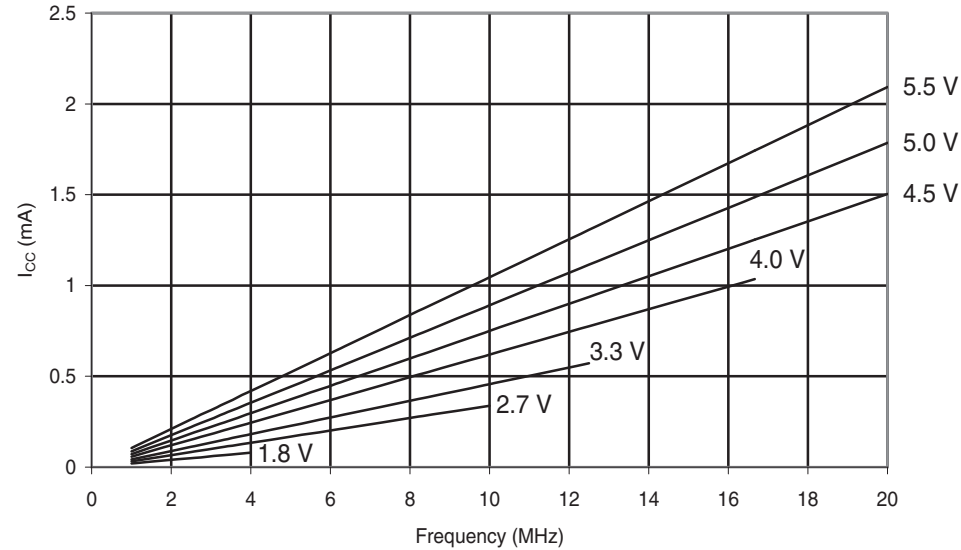
Figure 30-234.ATmega168A: Reset Supply Current vs. Frequency (1 - 20MHz)
