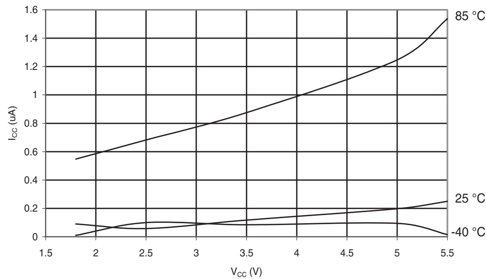
Figure 30-152. ATmega88PA: Power-Down Supply Current vs. V_{CC} (Watchdog Timer Disabled)
