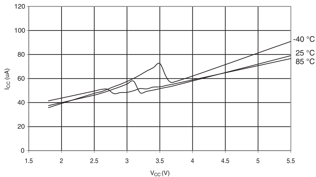
Figure 30-370. ATmega328P: Analog Comparator Current vs. V_{CC}
