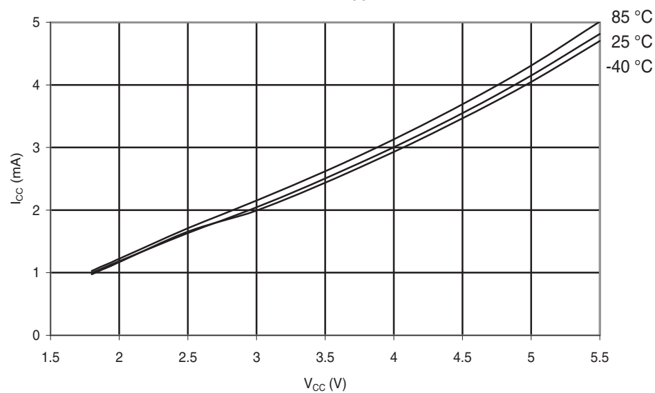
Figure 30-240. ATmega168PA: Active Supply Current vs. V_{CC} (Internal RC Oscillator, 8MHz)
