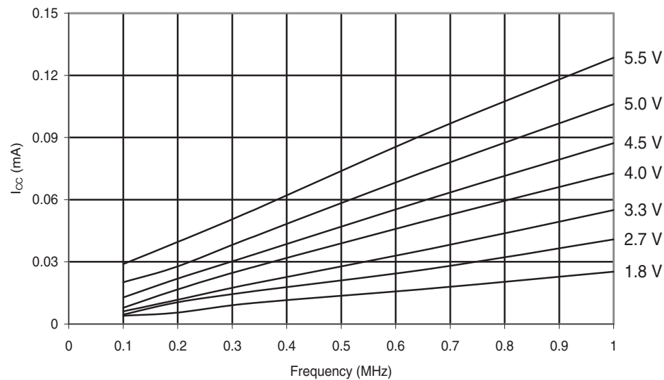
Figure 30-147.ATmega88PA: Idle Supply Current vs. Low Frequency (0.1-1.0MHz)
