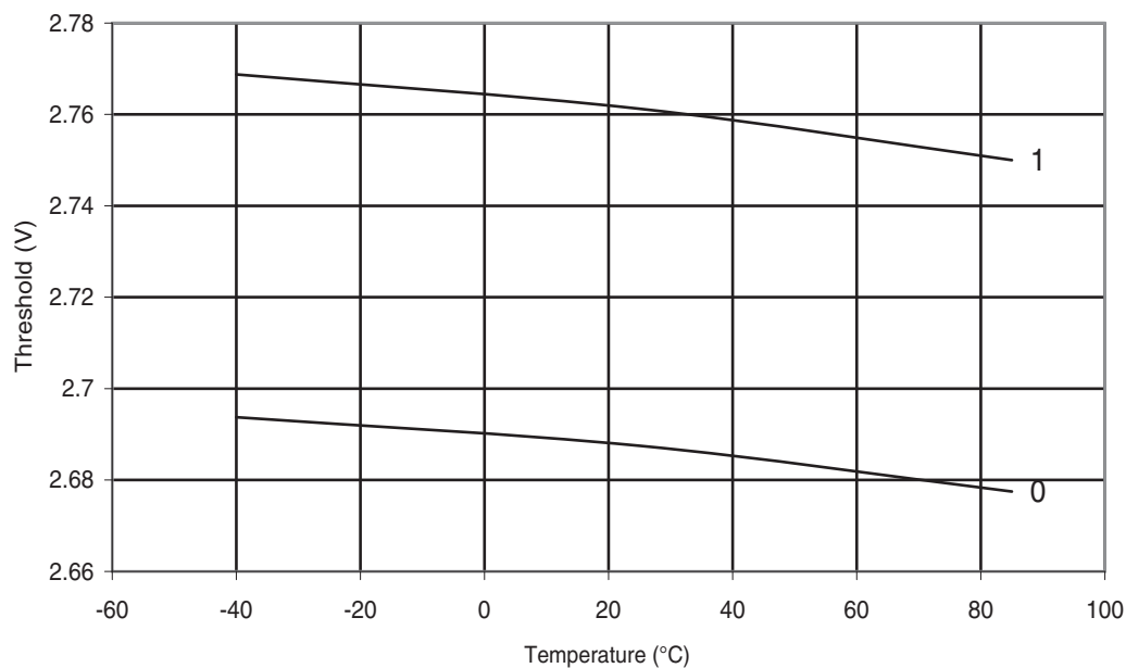
Figure 30-314. ATmega328: BOD Thresholds vs. Temperature (BODLEVEL is 2.7 V)
