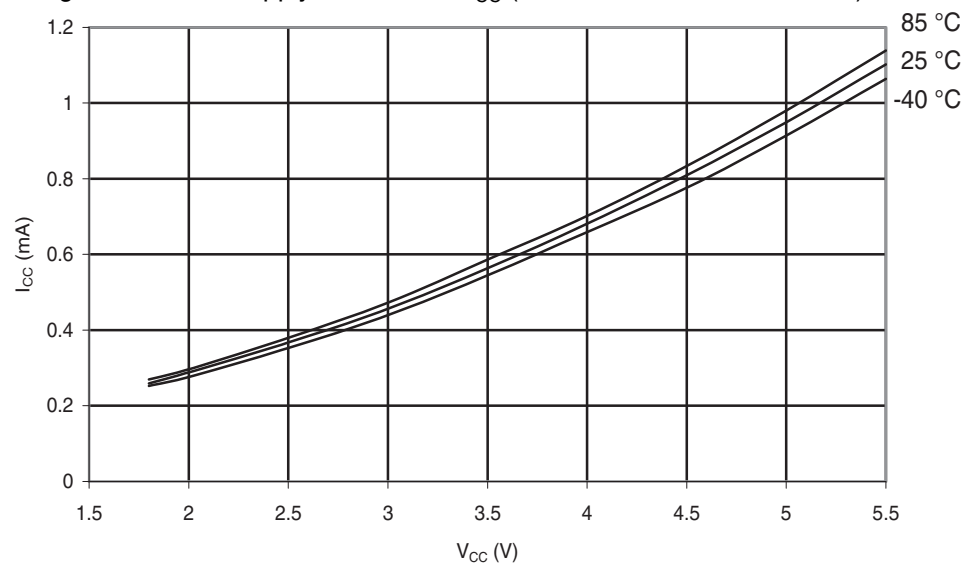
Figure 30-98. ATmega88A: Active Supply Current vs. V_{CC} (Internal RC Oscillator, 1MHz)
