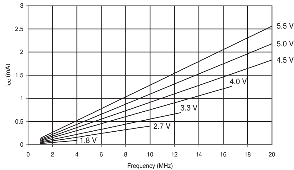
Figure 30-195. ATmega168A: Idle Supply Current vs. Frequency (1-20MHz)
