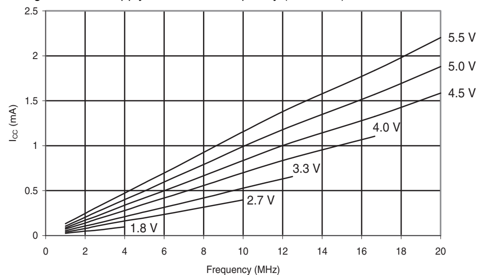
Figure 30-101.ATmega88A: Idle Supply Current vs. Frequency (1-20MHz)
