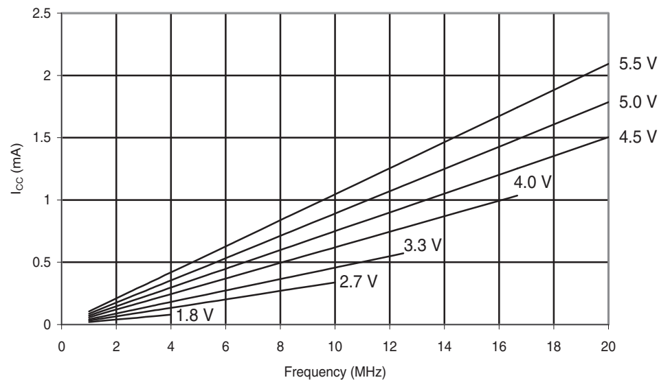
Figure 30-281.ATmega168PA: Reset Supply Current vs. Frequency (1 - 20MHz)
