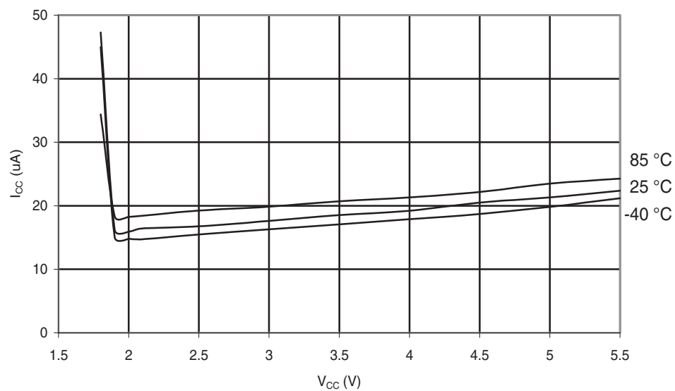
Figure 30-184. ATmega88PA: Brownout Detector Current vs. V_{CC}
