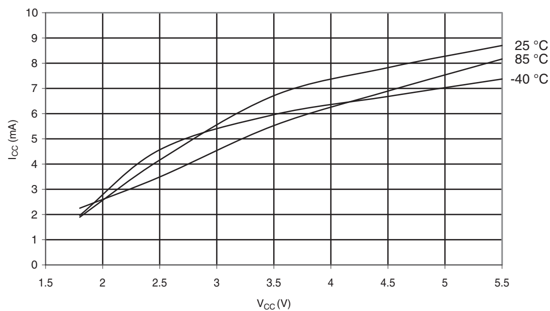
Figure 30-373. ATmega328P: Programming Current vs. V_{CC}
