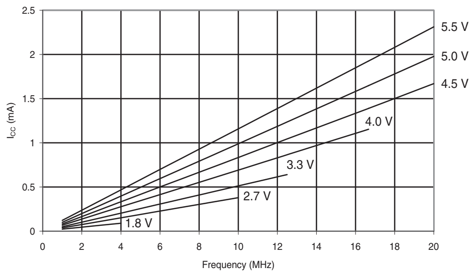
Figure 30-46. ATmega48A: Reset Supply Current vs. Frequency (1 - 20MHz)
