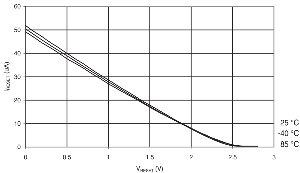
Figure 30-66. ATmega48PA: Reset Pull-up Resistor Current vs. Reset Pin Voltage ( V_{CC} = 2.7\text{ V} )
