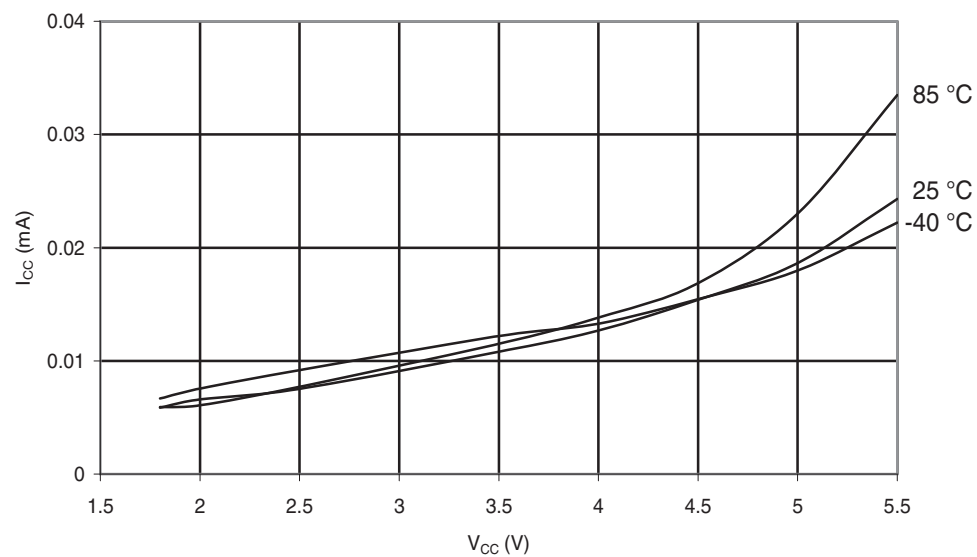
Figure 30-102. ATmega88A: Idle Supply Current vs. V_{CC} (Internal RC Oscillator, 128kHz)
