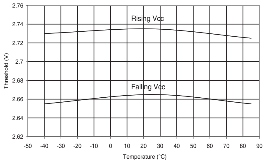
Figure 30-267.ATmega168PA: BOD Thresholds vs. Temperature (BODLEVEL is 2.7 V)
