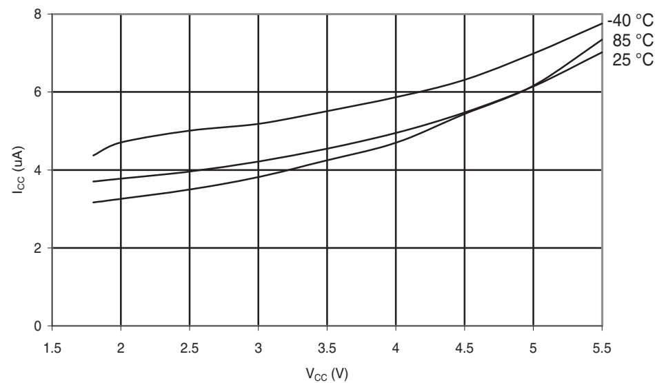
Figure 30-247. ATmega168PA: Power-Down Supply Current vs. V_{CC} (Watchdog Timer Enabled)
