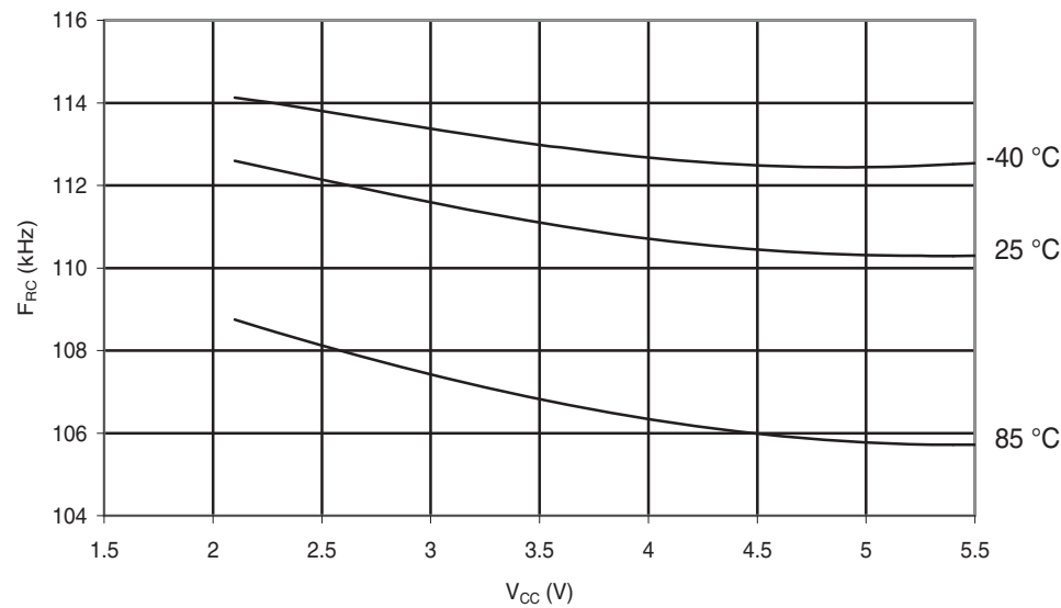
Figure 30-177.ATmega88PA: Watchdog Oscillator Frequency vs. V_{CC}
