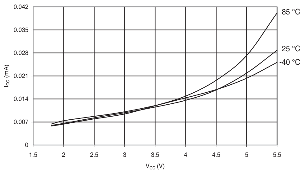
Figure 30-8. ATmega48A: Idle Supply Current vs. V_{CC} (Internal RC Oscillator, 128kHz)
