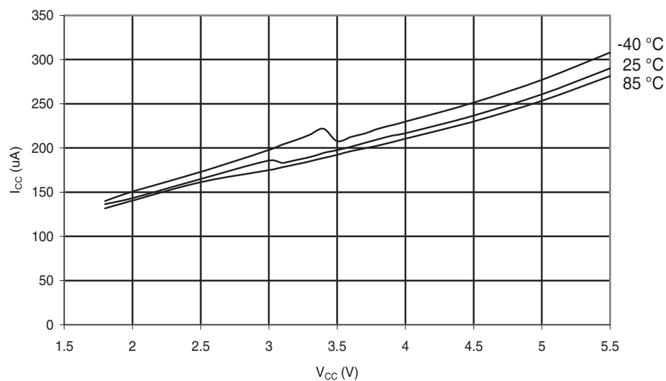
Figure 30-87. ATmega48PA: ADC Current vs. V_{CC} (AREF = AV_{CC} )
