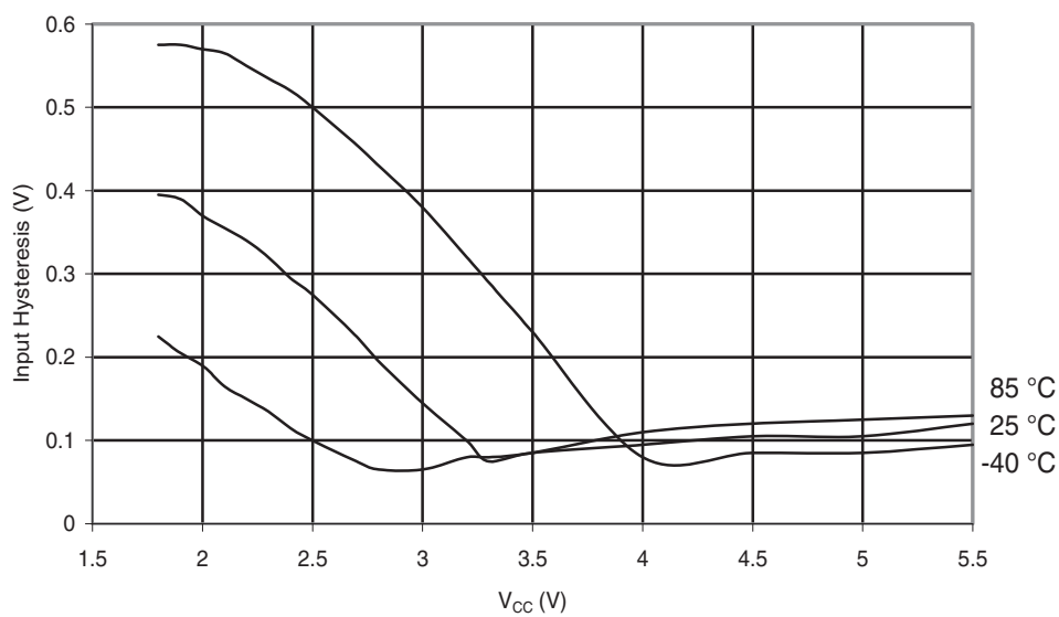
Figure 30-171. ATmega88PA: Reset Pin Input Hysteresis vs. V_{CC}
