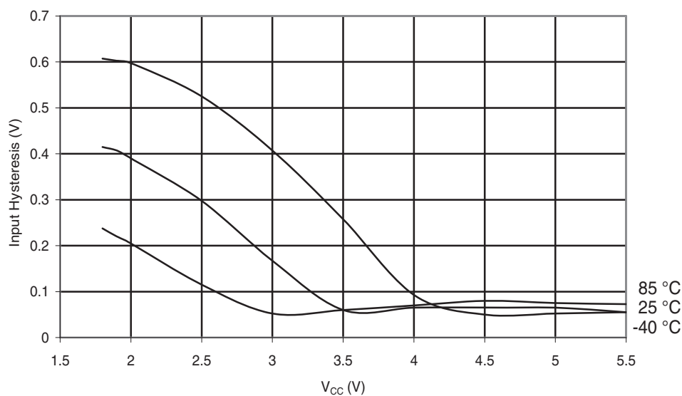
Figure 30-30. ATmega48A: Reset Pin Input Hysteresis vs. V_{CC}
