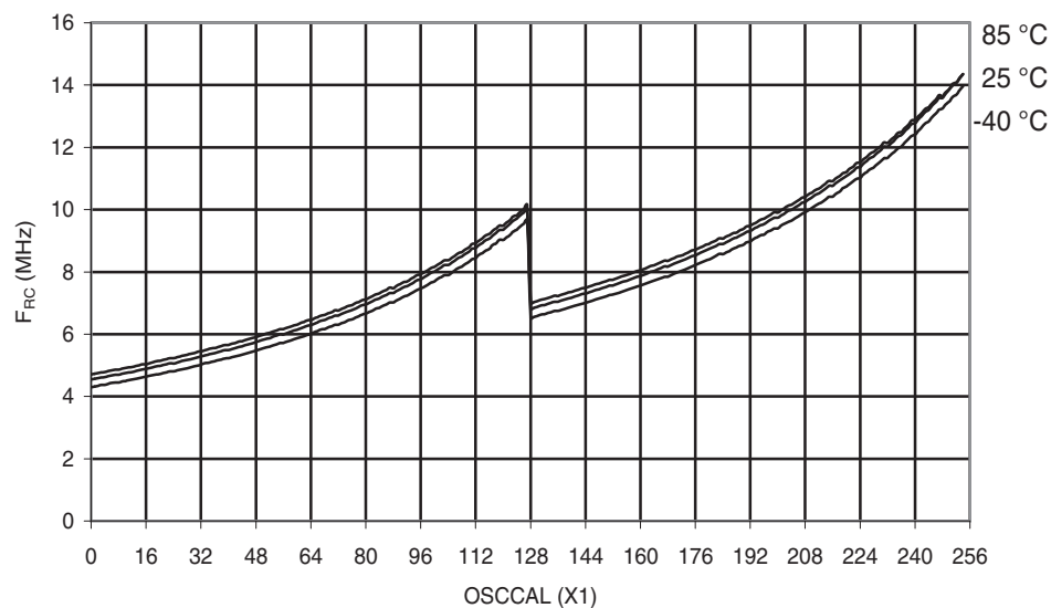
Figure 30-227. ATmega168A: Calibrated 8MHz RC Oscillator Frequency vs. OSCCAL Value
