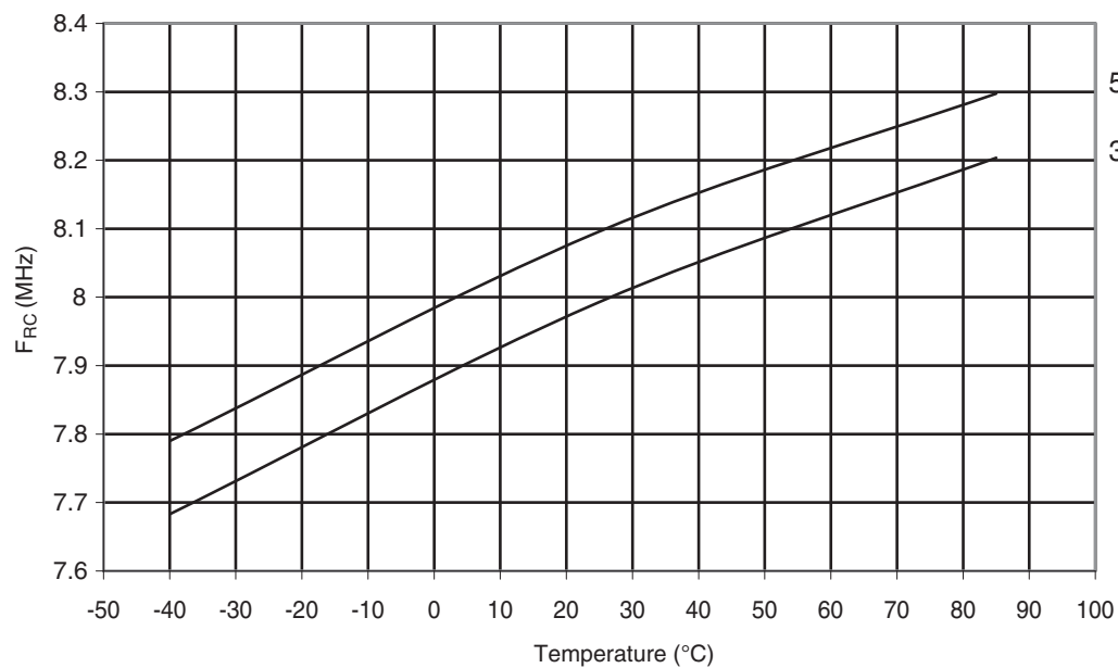
Figure 30-367. ATmega328P: Calibrated 8MHz RC Oscillator Frequency vs. Temperature
