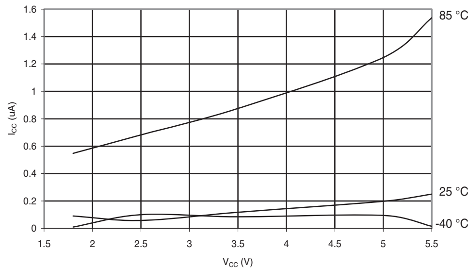
Figure 30-105.ATmega88A: Power-Down Supply Current vs. V CC (Watchdog Timer Disabled)
