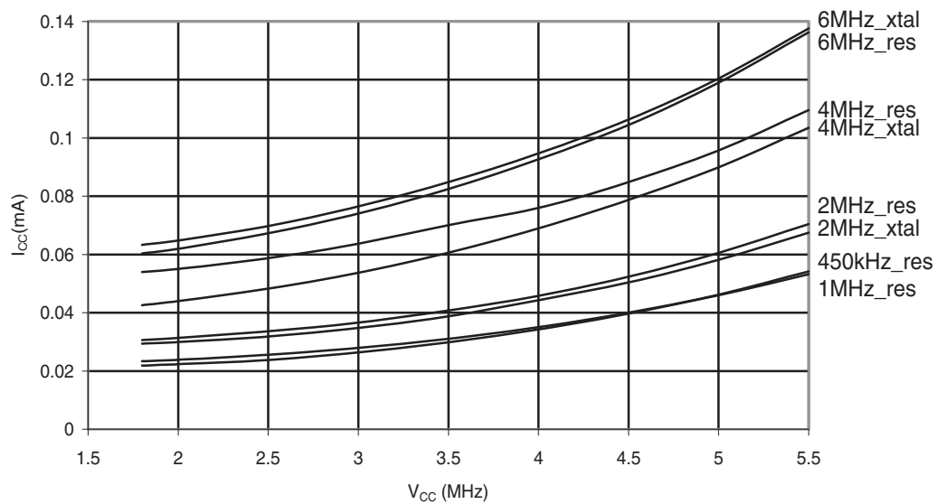
Figure 30-249. ATmega168PA: Standby Supply Current vs. V_{CC} (Watchdog Timer Disabled)
