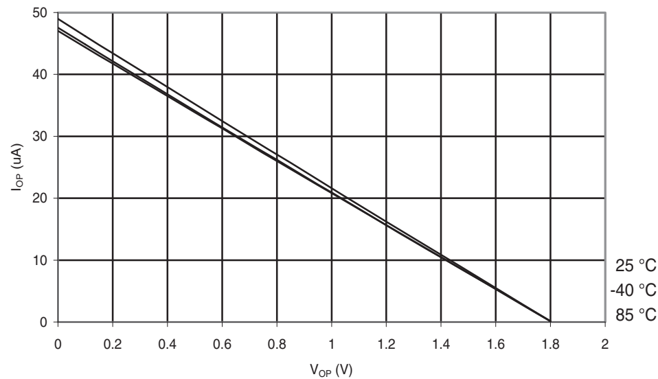
Figure 30-250.ATmega168PA: I/O Pin Pull-up Resistor Current vs. Input Voltage ( V_{CC} = 1.8\text{ V} )
