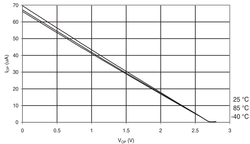
Figure 30-63. ATmega48PA: I/O Pin Pull-up Resistor Current vs. Input Voltage ( V_{CC} = 2.7\text{ V} )
