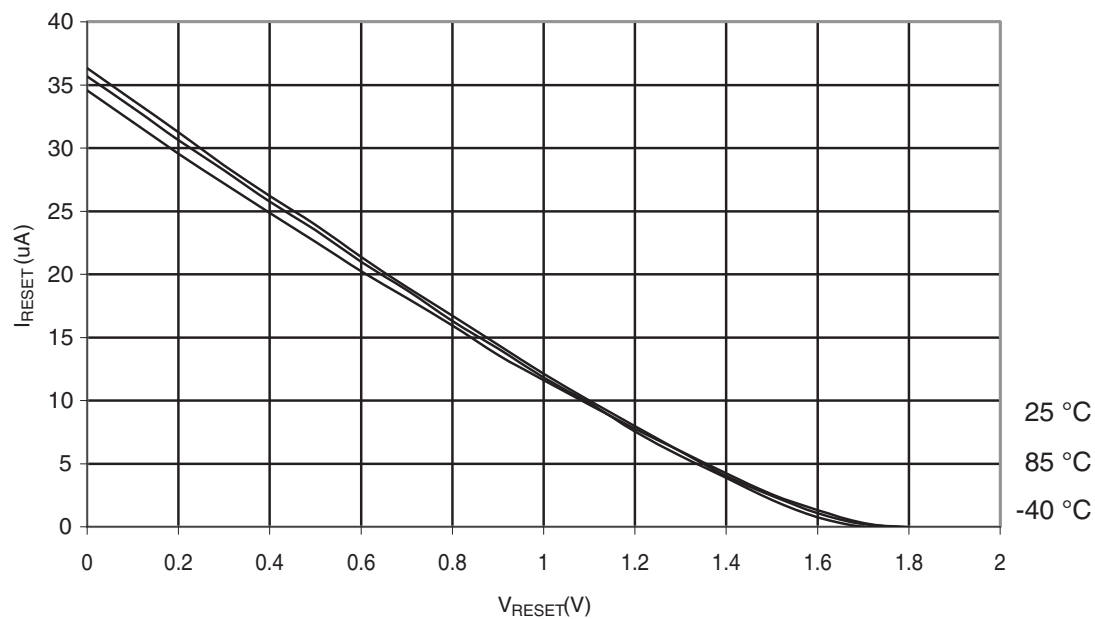
Figure 30-347. ATmega328P: Reset Pull-up Resistor Current vs. Reset Pin Voltage ( V_{CC} = 1.8\text{ V} )
