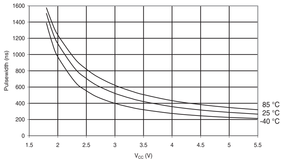
Figure 30-188. ATmega88PA: Minimum Reset Pulse width vs. V_{CC}
