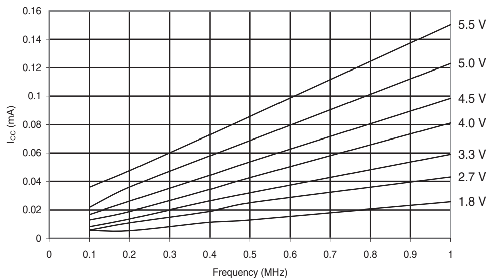
Figure 30-53. ATmega48PA: Idle Supply Current vs. Low Frequency (0.1-1.0MHz)
