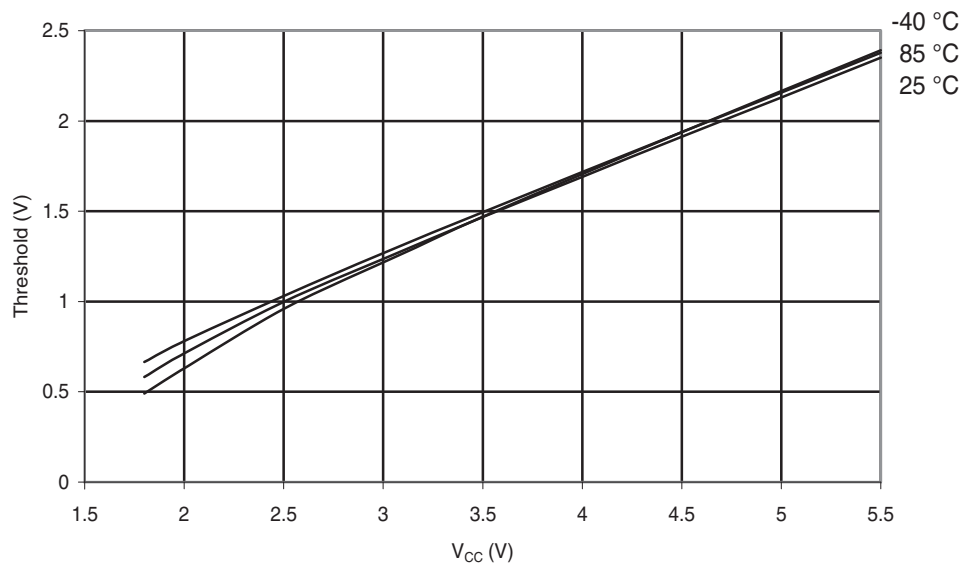
Figure 30-120. ATmega88A: I/O Pin Input Threshold Voltage vs. V_{CC} ( V_{IL} , I/O Pin read as '0')
