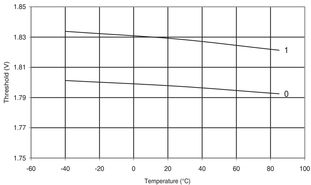
Figure 30-313. ATmega328: BOD Thresholds vs. Temperature (BODLEVEL is 1.8 V)
