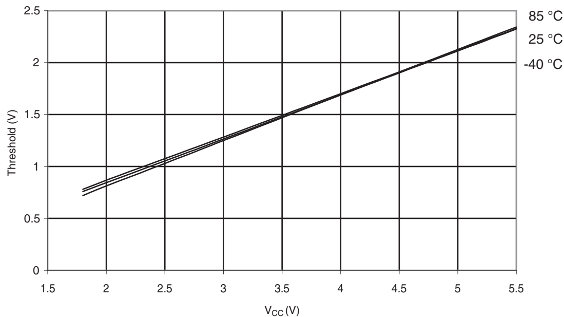
Figure 30-311. ATmega328: Reset Input Threshold Voltage vs. V_{CC} ( V_{IL} , I/O Pin read as '0')
