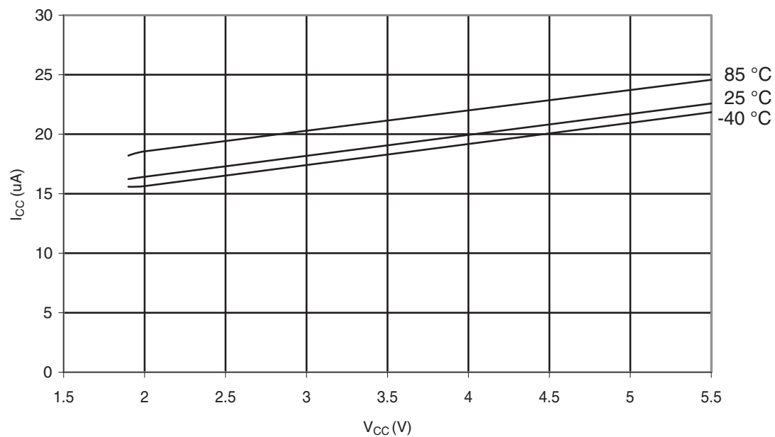
Figure 30-372. ATmega328P: Brownout Detector Current vs. V_{CC}
