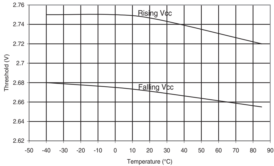
Figure 30-32. ATmega48A: BOD Thresholds vs. Temperature (BODLEVEL is 2.7 V)
