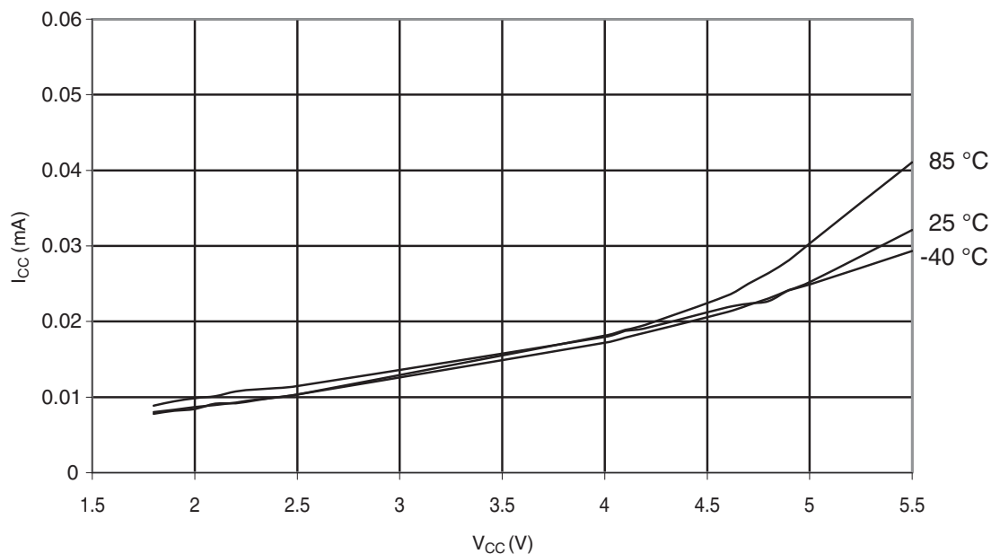
Figure 30-337. ATmega328P: Idle Supply Current vs. V_{CC} (Internal RC Oscillator, 128kHz)
