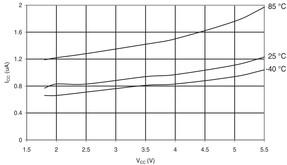
Figure 30-60. ATmega48PA: Power-Save Supply Current vs. V_{CC} (Watchdog Timer Disabled and 32kHz Crystal Oscillator Running)
