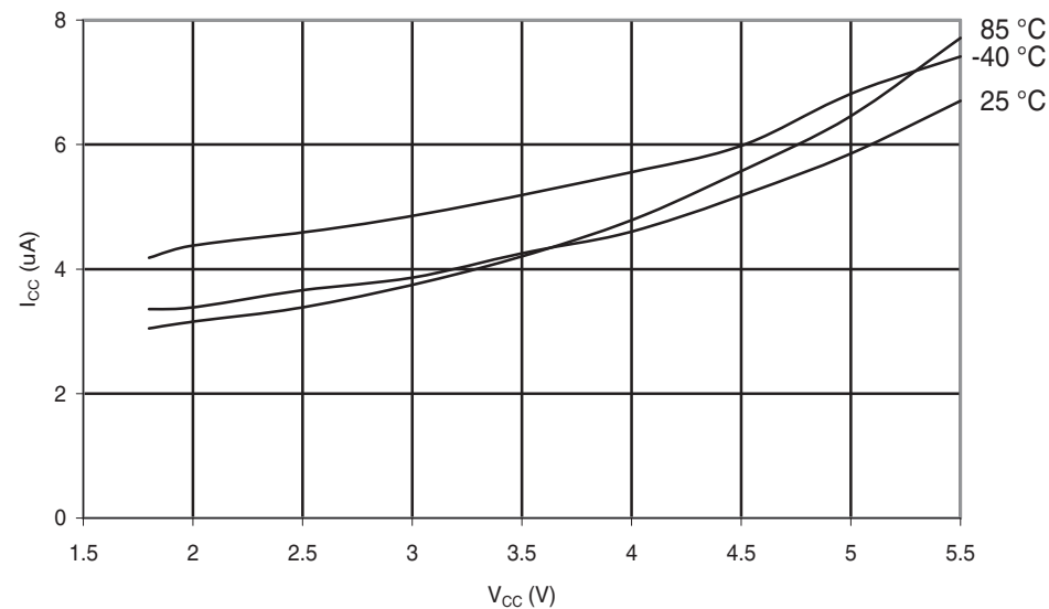
Figure 30-106.ATmega88A: Power-Down Supply Current vs. V CC (Watchdog Timer Enabled)
