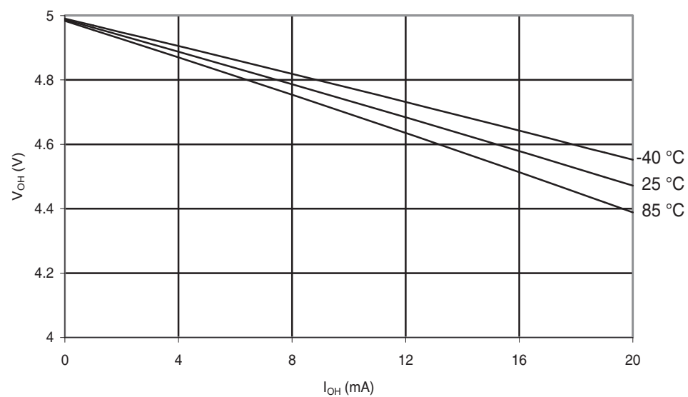
Figure 30-212. ATmega168A: I/O Pin Output Voltage vs. Source Current ( V_{CC} = 5\text{ V} )
