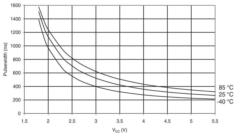
Figure 30-141. ATmega88A: Minimum Reset Pulse width vs. V_{CC}
