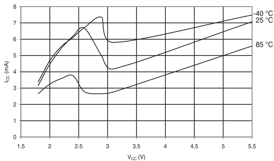
Figure 30-138. ATmega88A: Programming Current vs. V_{CC}
