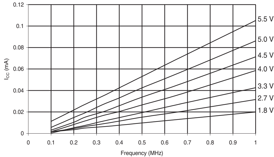
Figure 30-280.ATmega168PA: Reset Supply Current vs. Low Frequency (0.1 - 1.0MHz)
