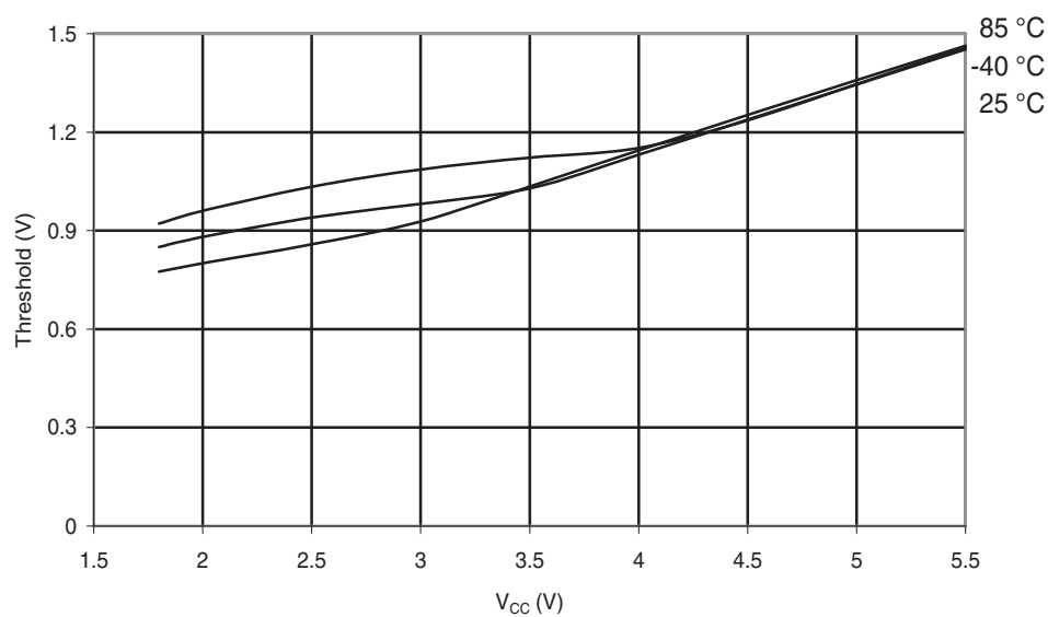
Figure 30-216. ATmega168A: Reset Input Threshold Voltage vs. V_{CC} ( V_{IH} , I/O Pin read as '1')
