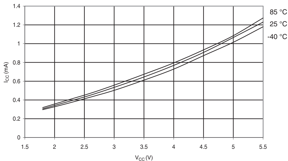
Figure 30-333. ATmega328P: Active Supply Current vs. V_{CC} (Internal RC Oscillator, 1MHz)
