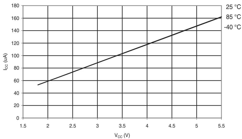
Figure 30-277. ATmega168PA: AREF External Reference Current vs. V_{CC}
