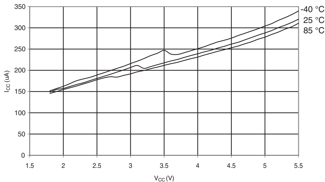
Figure 30-369. ATmega328P: ADC Current vs. V_{CC} (AREF = AV_{CC} )
