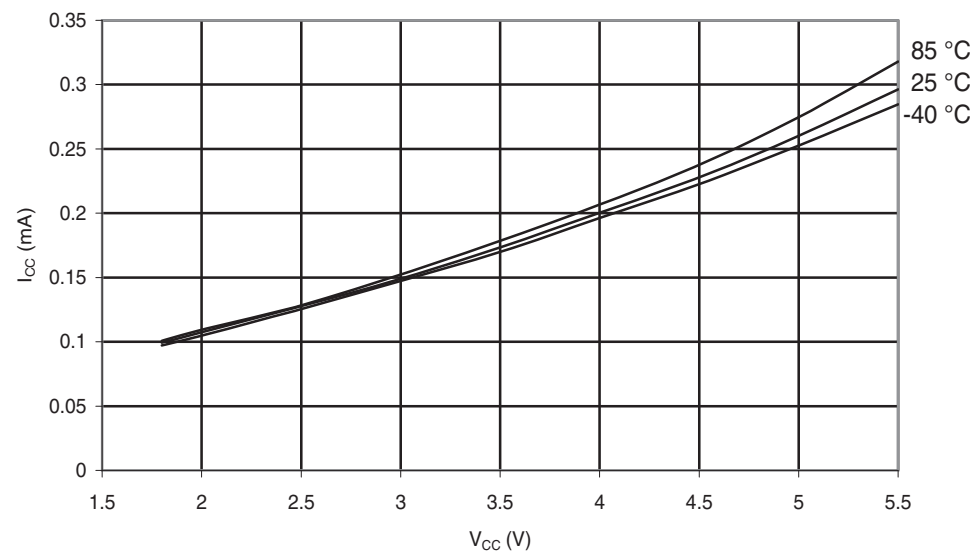
Figure 30-103. ATmega88A: Idle Supply Current vs. V_{CC} (Internal RC Oscillator, 1MHz)
