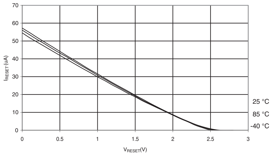
Figure 30-348. ATmega328P: Reset Pull-up Resistor Current vs. Reset Pin Voltage ( V_{CC} = 2.7\text{ V} )
