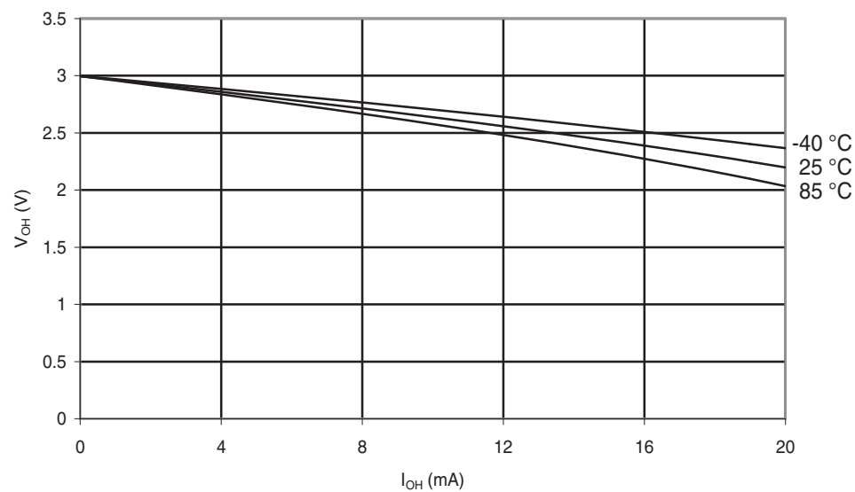
Figure 30-117. ATmega88A: I/O Pin Output Voltage vs. Source Current ( V_{CC} = 3\text{ V} )
