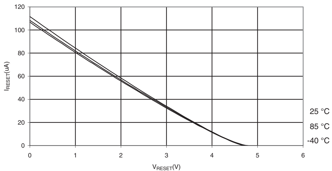
Figure 30-349. ATmega328P: Reset Pull-up Resistor Current vs. Reset Pin Voltage ( V_{CC} = 5\text{ V} )
