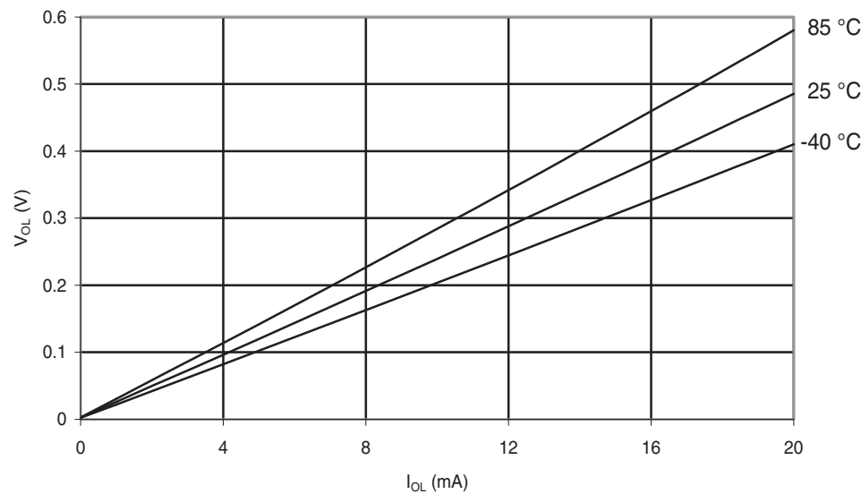
Figure 30-69. ATmega48PA: I/O Pin Output Voltage vs. Sink Current ( V_{CC} = 5\text{ V} )
