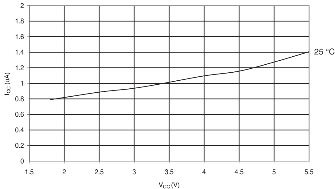
Figure 30-342. ATmega328P: Power-Save Supply Current vs. V CC (Watchdog Timer Disabled and 32kHz Crystal Oscillator Running)
