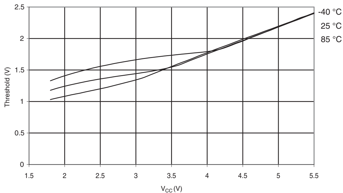
Figure 30-310. ATmega328: Reset Input Threshold Voltage vs. V_{CC} ( V_{IH} , I/O Pin read as '1')
