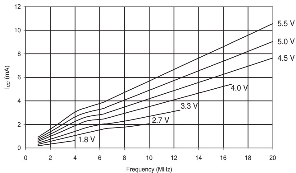
Figure 30-190. ATmega168A: Active Supply Current vs. Frequency (1-20MHz)
