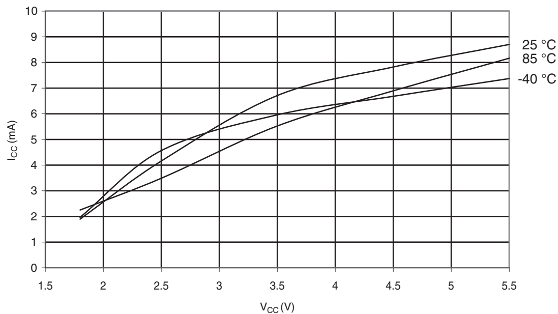
Figure 30-326. ATmega328: Programming Current vs. V_{CC}
