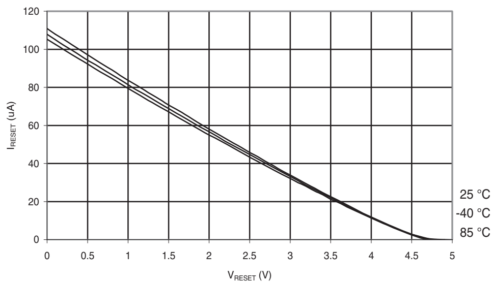
Figure 30-161. ATmega88PA: Reset Pull-up Resistor Current vs. Reset Pin Voltage ( V_{CC} = 5\text{ V} )
