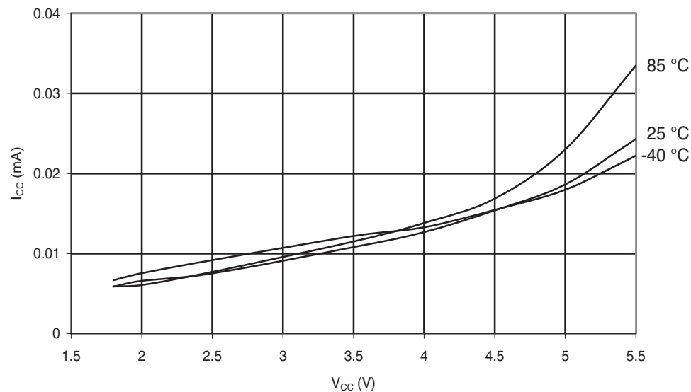
Figure 30-149. ATmega88PA: Idle Supply Current vs. V_{CC} (Internal RC Oscillator, 128kHz)
