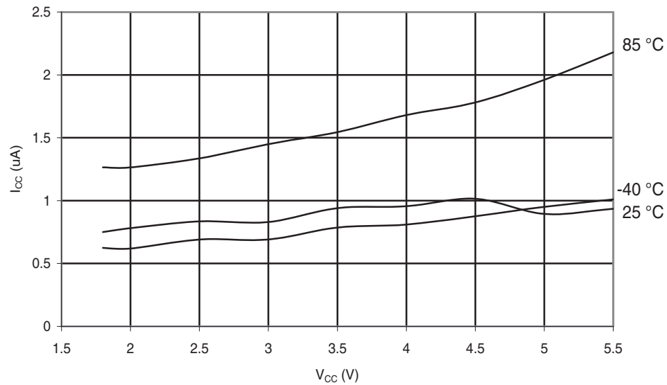
Figure 30-248. ATmega168PA: Power-Save Supply Current vs. V_{CC} (Watchdog Timer Disabled and 32kHz Crystal Oscillator Running)
