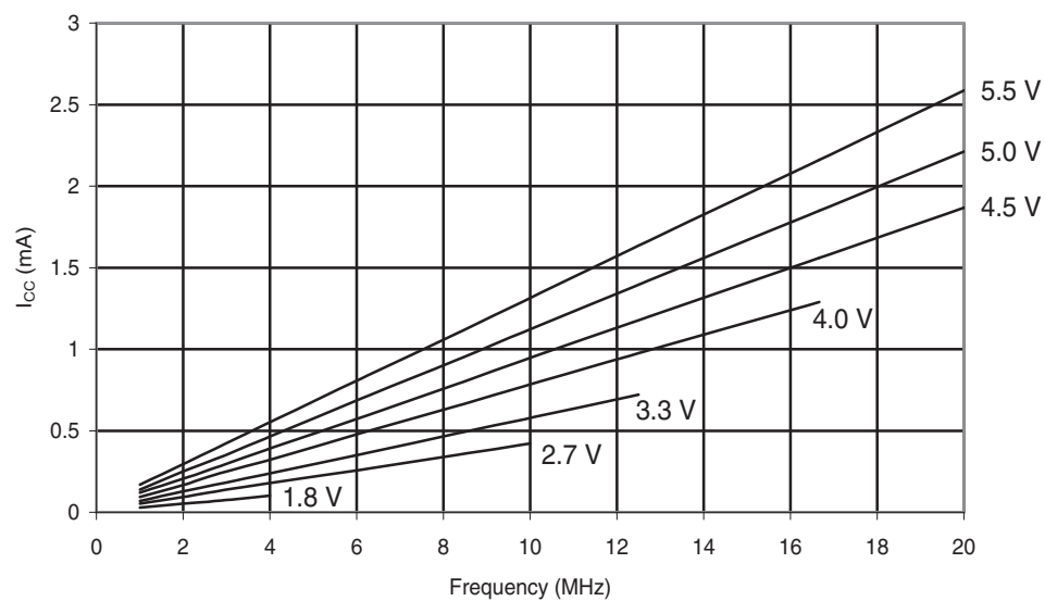
Figure 30-54. ATmega48PA: Idle Supply Current vs. Frequency (1-20MHz)
