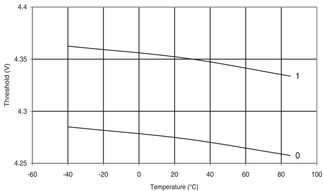
Figure 30-362. ATmega328P: BOD Thresholds vs. Temperature (BODLEVEL is 4.3 V)
