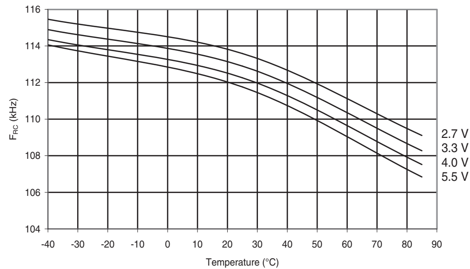
Figure 30-82. ATmega48PA: Watchdog Oscillator Frequency vs. Temperature
