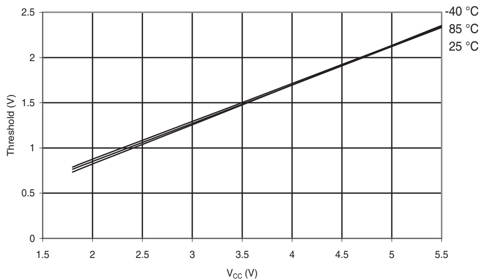
Figure 30-264. ATmega168PA: Reset Input Threshold Voltage vs. V_{CC} ( V_{IL} , I/O Pin read as '0')
