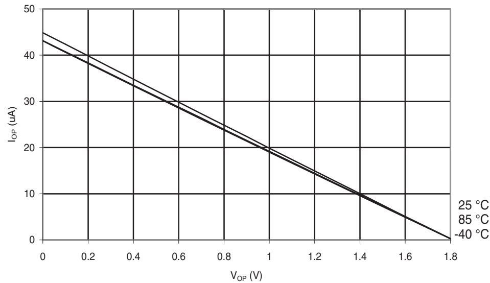
Figure 30-62. ATmega48PA: I/O Pin Pull-up Resistor Current vs. Input Voltage ( V_{CC} = 1.8\text{ V} )
