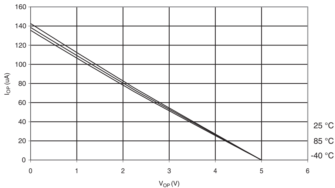
Figure 30-299. ATmega328: I/O Pin Pull-up Resistor Current vs. Input Voltage ( V_{CC} = 5\text{ V} )
