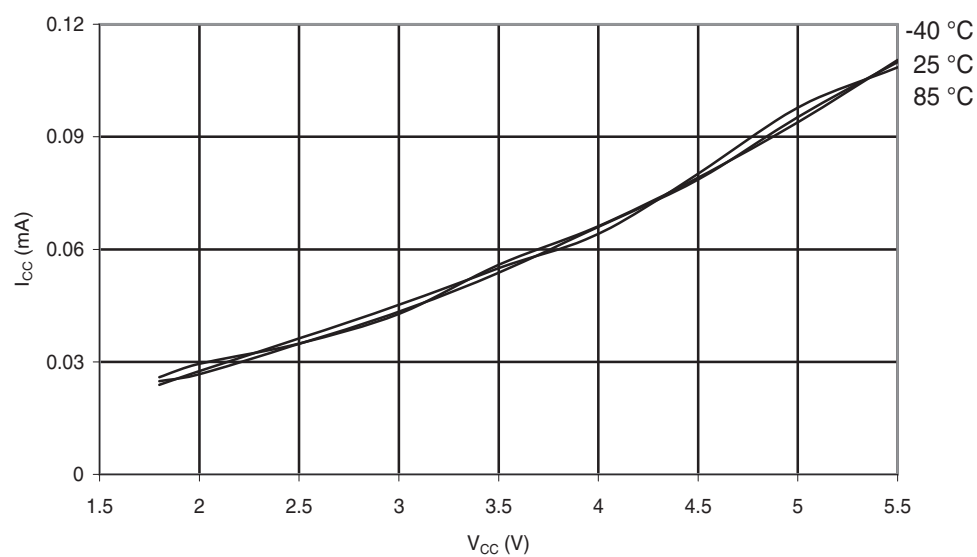
Figure 30-97. ATmega88A: Active Supply Current vs. V_{CC} (Internal RC Oscillator, 128kHz)
