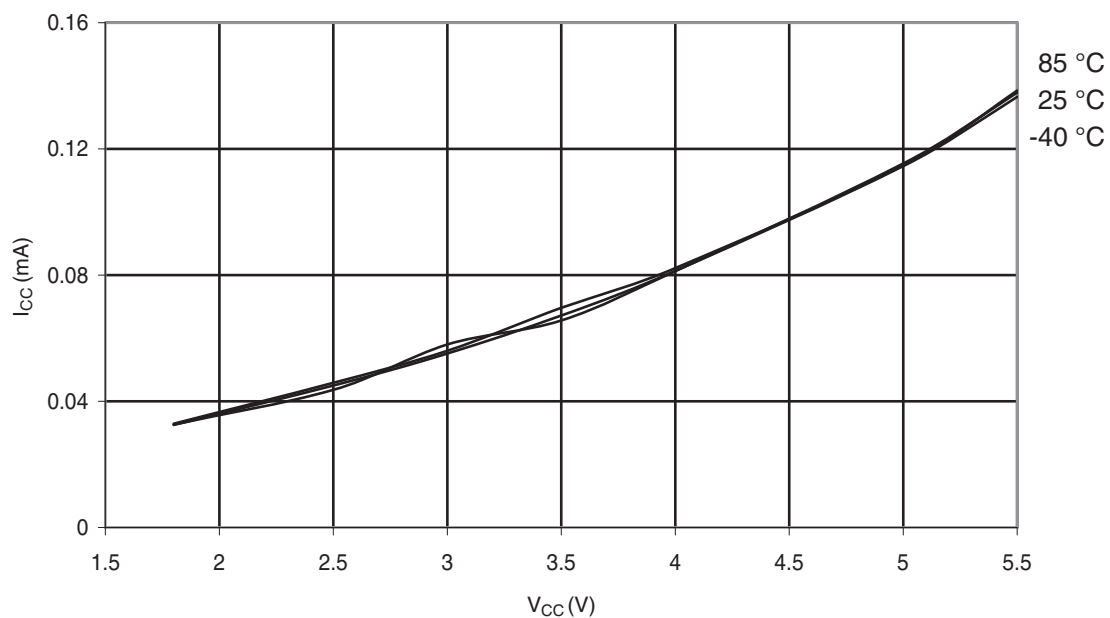
Figure 30-332. ATmega328P: Active Supply Current vs. V_{CC} (Internal RC Oscillator, 128kHz)
