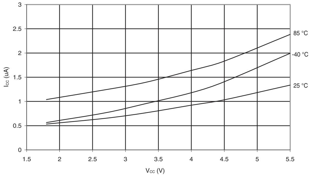
Figure 30-107. ATmega88A: Power-Save Supply Current vs. V_{CC} (Watchdog Timer Disabled and 32kHz Crystal Oscillator Running)
