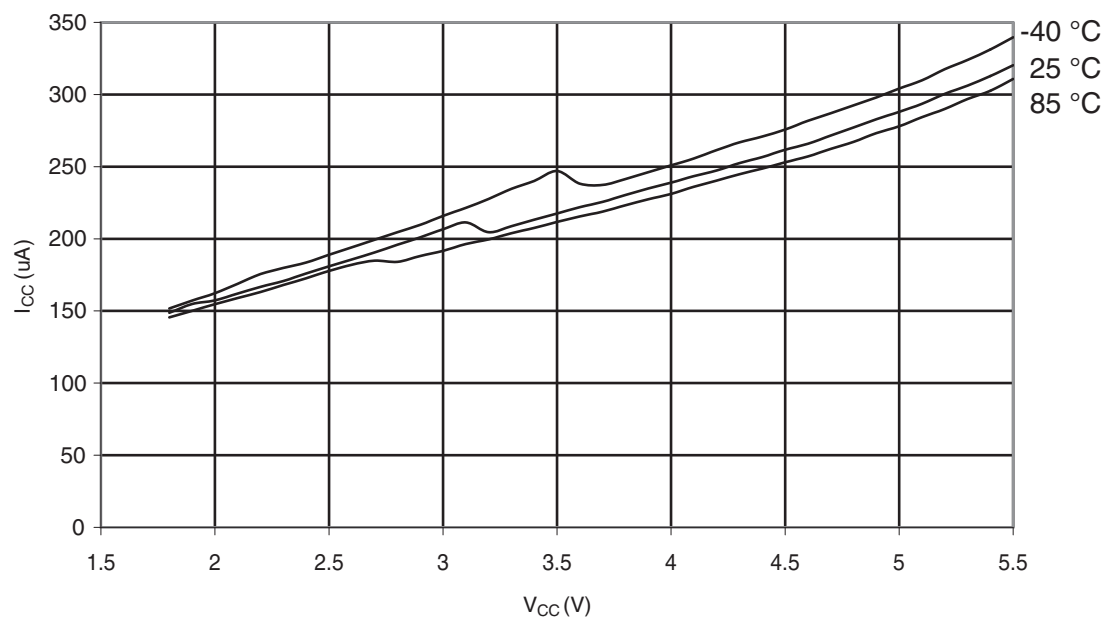
Figure 30-322. ATmega328: ADC Current vs. V_{CC} (AREF = AV_{CC} )
