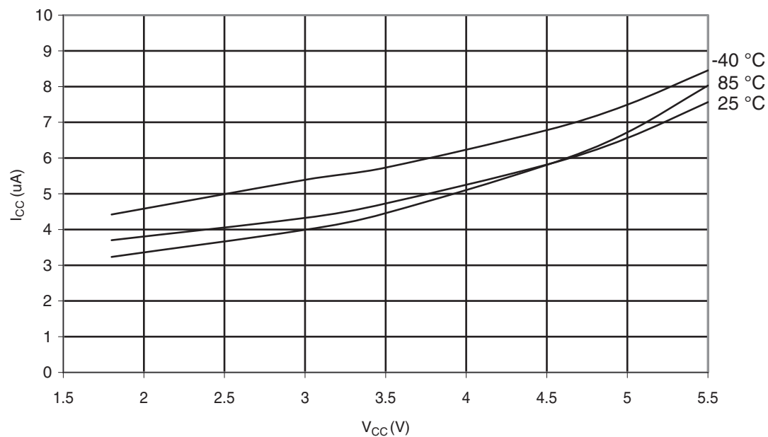
Figure 30-294. ATmega328: Power-Down Supply Current vs. V_{CC} (Watchdog Timer Enabled)
