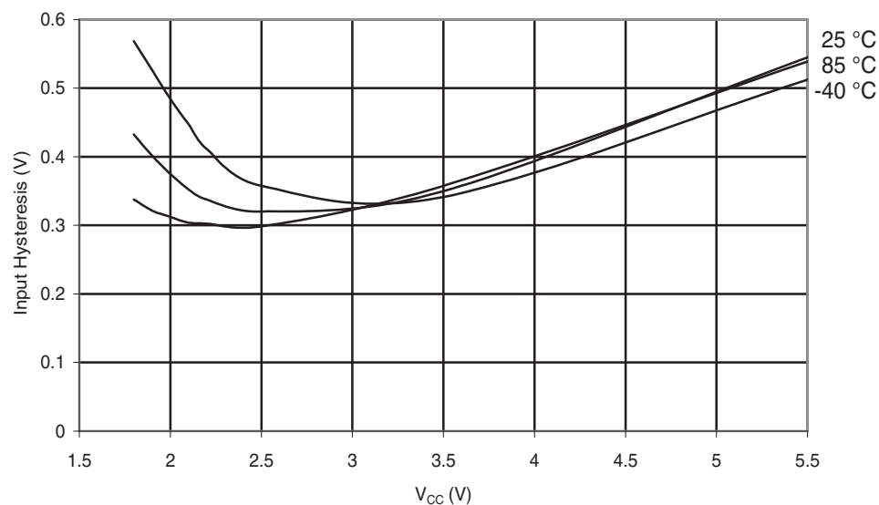
Figure 30-74. ATmega48PA: I/O Pin Input Hysteresis vs. V_{CC}
