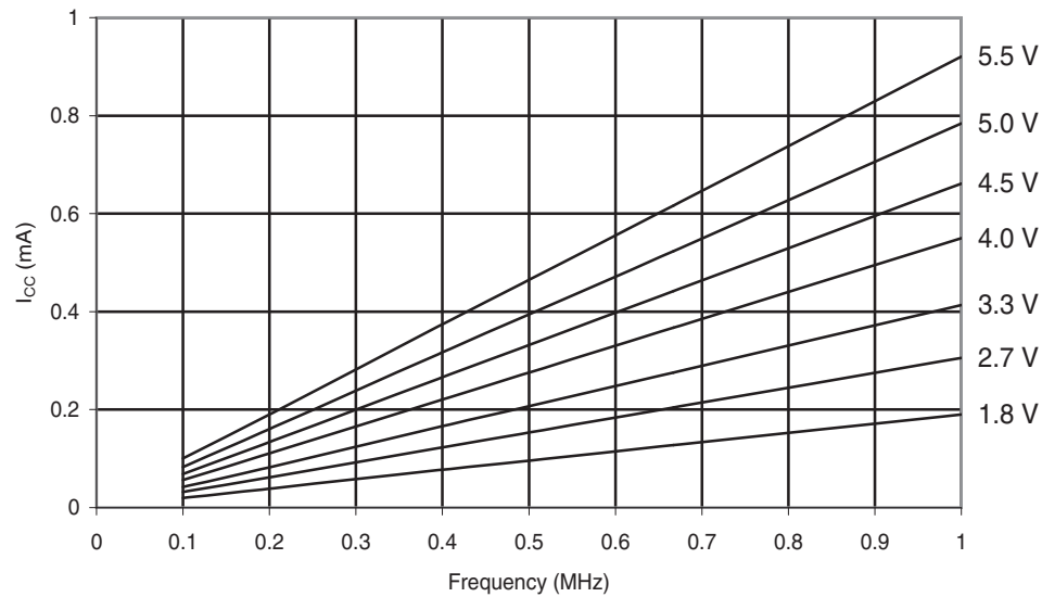
Figure 30-236. ATmega168PA: Active Supply Current vs. Low Frequency (0.1-1.0MHz)
