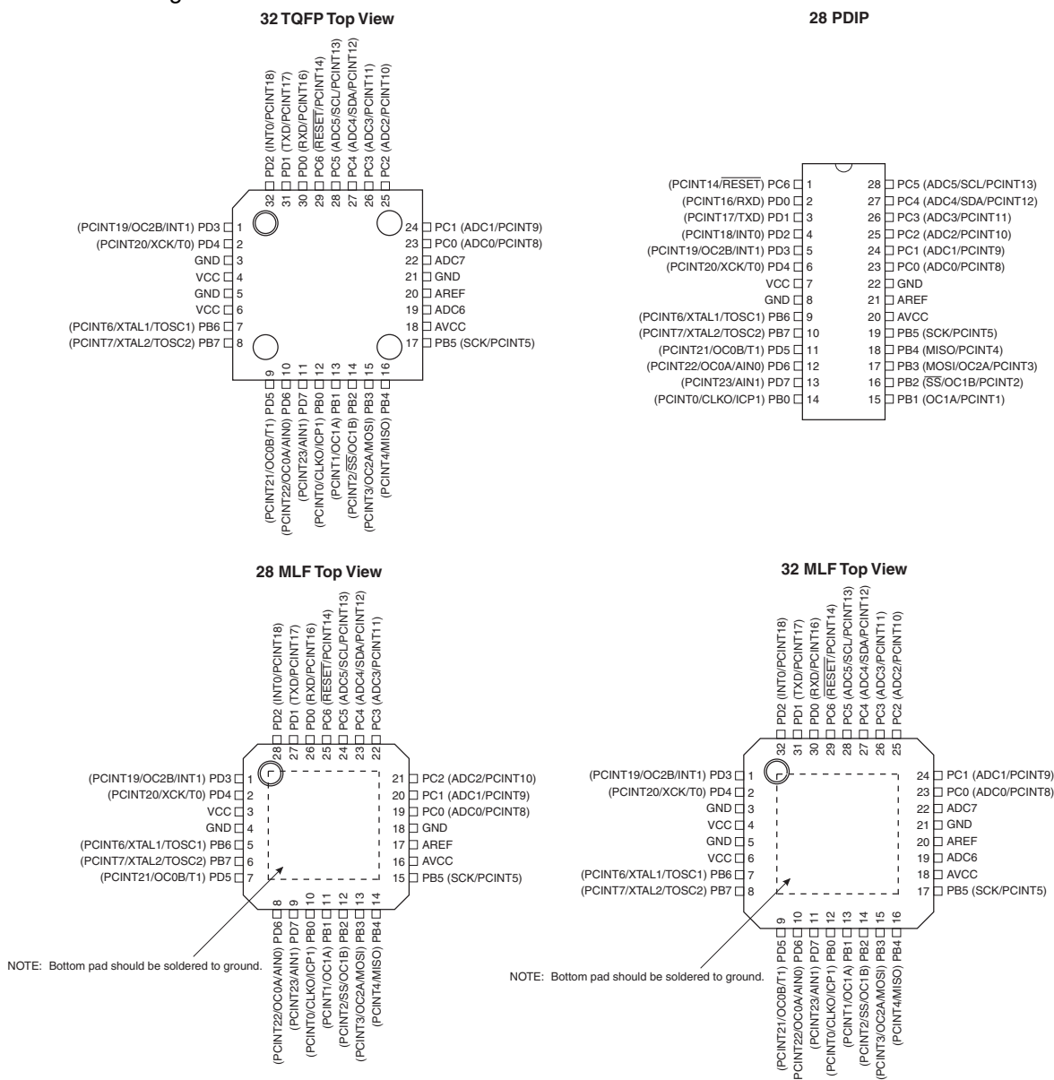
Figure 1-1. Pinout ATmega48A/PA/88A/PA/168A/PA/328/P
