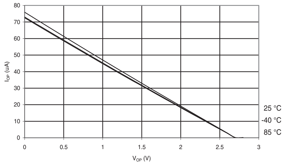
Figure 30-110.ATmega88A: I/O Pin Pull-up Resistor Current vs. Input Voltage ( V_{CC} = 2.7\text{ V} )
