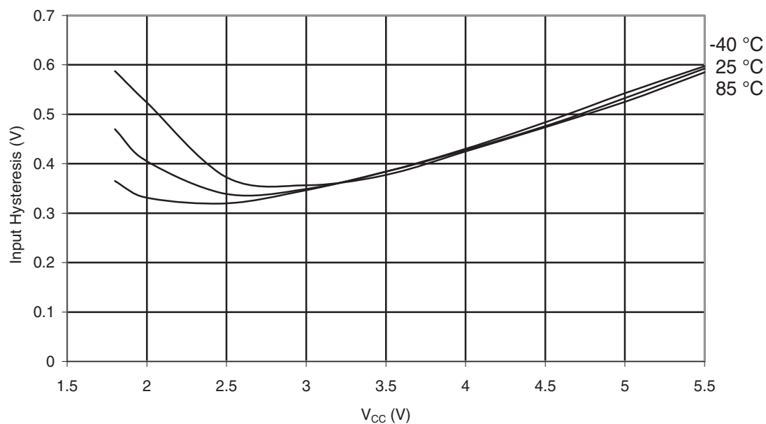
Figure 30-356. ATmega328P: I/O Pin Input Hysteresis vs. V_{CC}
