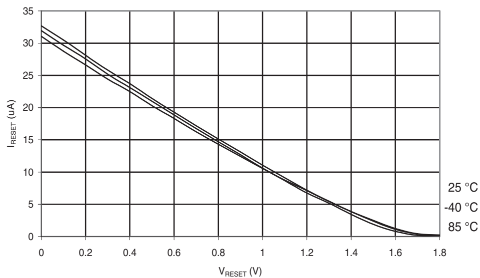
Figure 30-65. ATmega48PA: Reset Pull-up Resistor Current vs. Reset Pin Voltage ( V_{CC} = 1.8\text{ V} )
