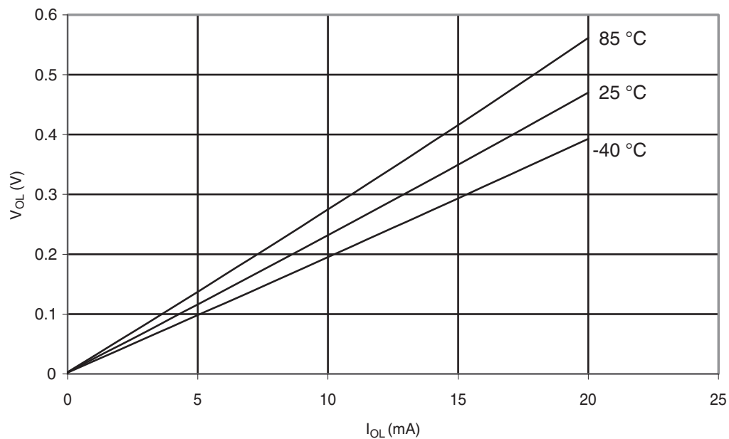
Figure 30-304. ATmega328: I/O Pin Output Voltage vs. Sink Current ( V_{CC} = 5\text{ V} )
