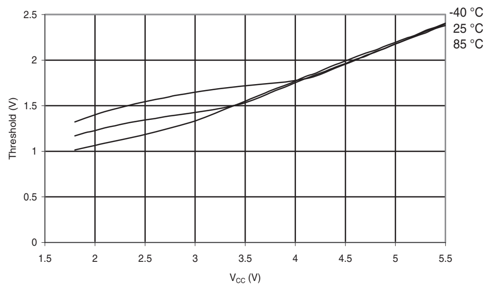
Figure 30-75. ATmega48PA: Reset Input Threshold Voltage vs. V_{CC} ( V_{IH} , I/O Pin read as '1')
