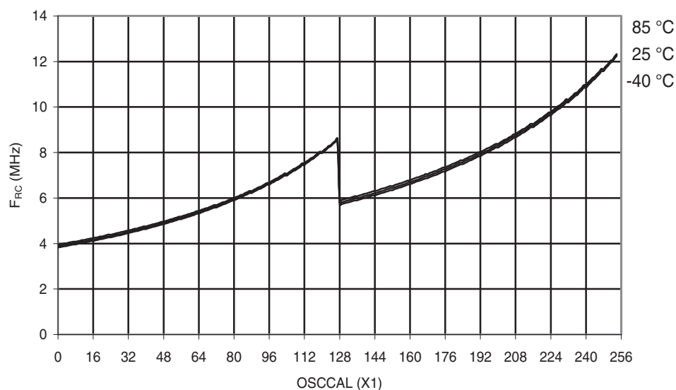
Figure 30-180. ATmega88PA: Calibrated 8MHz RC Oscillator Frequency vs. OSCCAL Value
