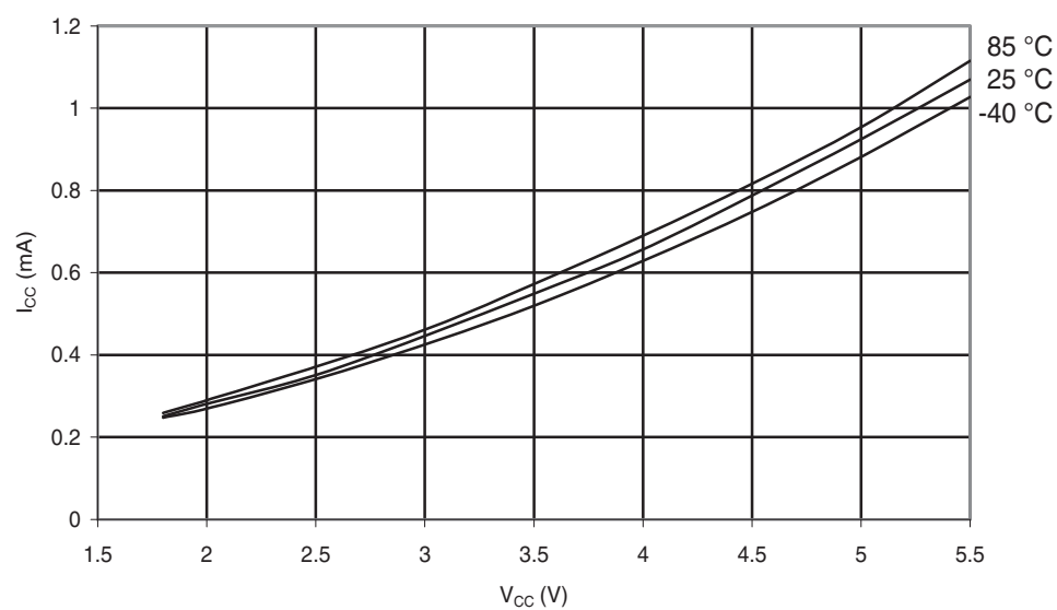
Figure 30-51. ATmega48PA: Active Supply Current vs. V_{CC} (Internal RC Oscillator, 1MHz)
