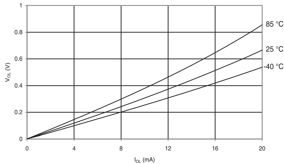
Figure 30-256. ATmega168PA: I/O Pin Output Voltage vs. Sink Current ( V_{CC} = 3\text{ V} )
