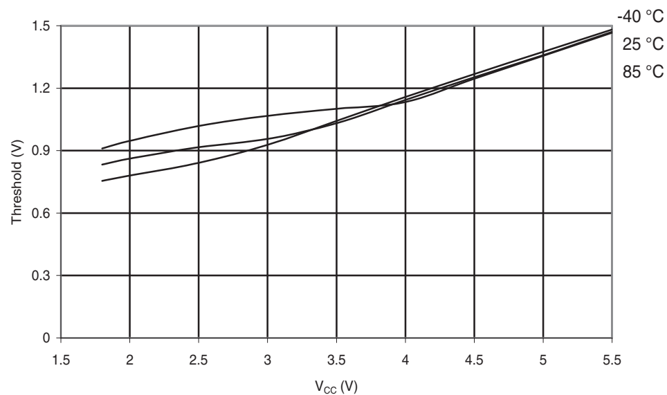
Figure 30-122. ATmega88A: Reset Input Threshold Voltage vs. V_{CC} ( V_{IH} , I/O Pin read as '1')
