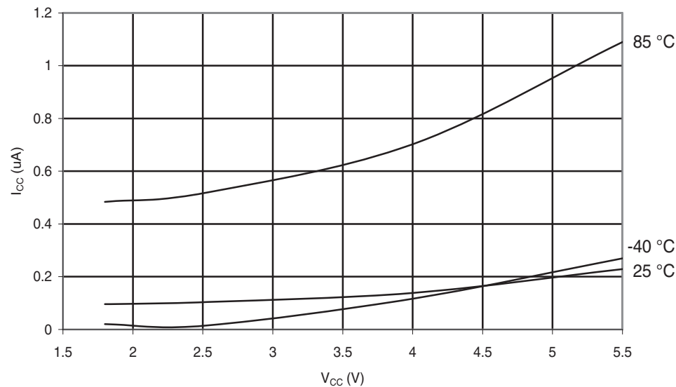
Figure 30-58. ATmega48PA: Power-Down Supply Current vs. V_{CC} (Watchdog Timer Disabled)
