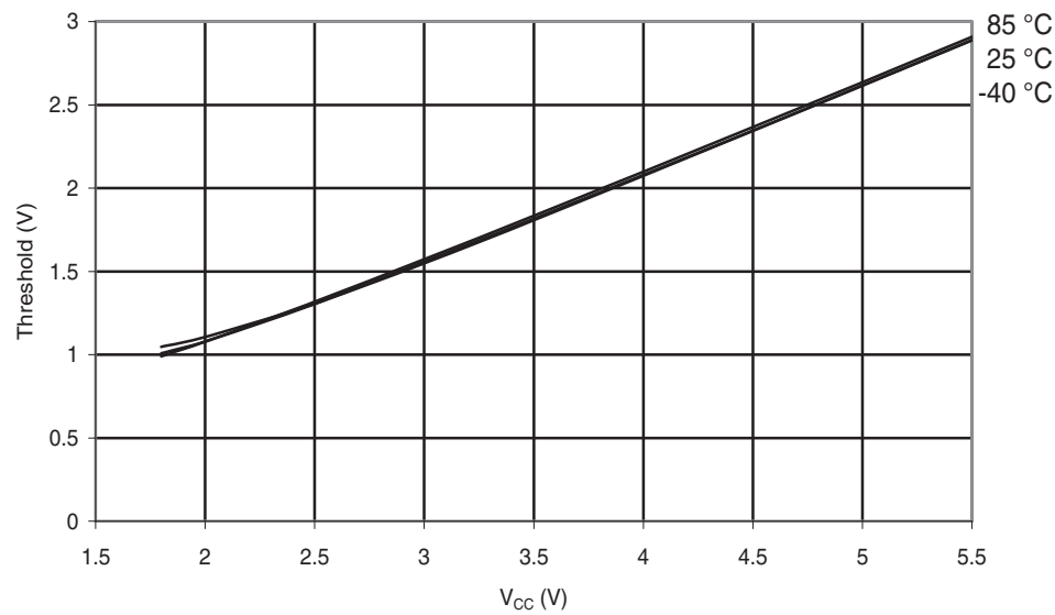
Figure 30-213. ATmega168A: I/O Pin Input Threshold Voltage vs. V_{CC} ( V_{IH} , I/O Pin read as '1')
