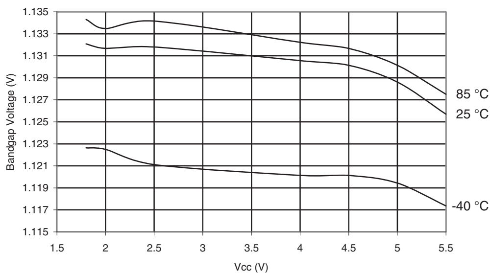
Figure 30-222. ATmega168A: Bandgap Voltage vs. V_{CC}
