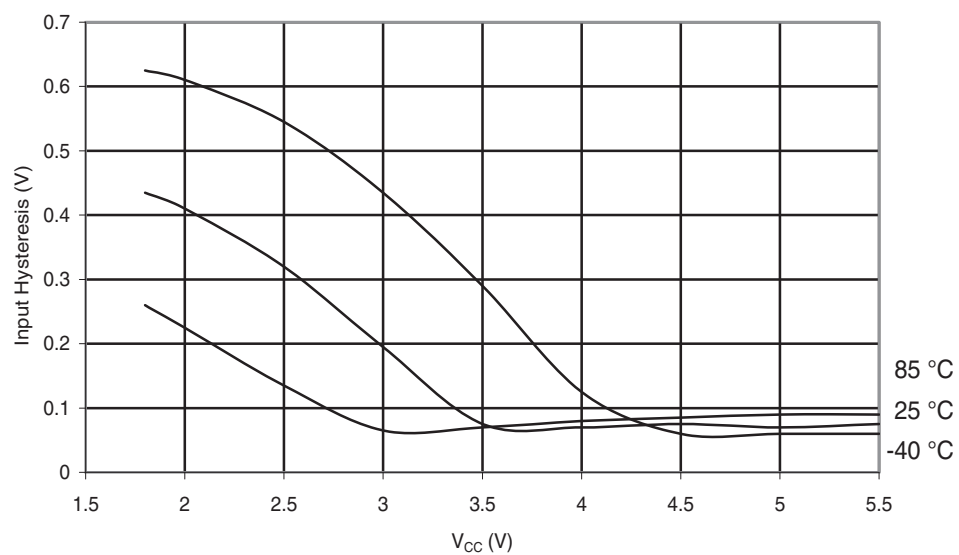
Figure 30-218. ATmega168A: Reset Pin Input Hysteresis vs. V_{CC}
