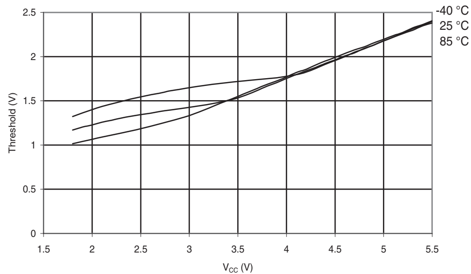
Figure 30-28. ATmega48A: Reset Input Threshold Voltage vs. V_{CC} ( V_{IH} , I/O Pin read as '1')
