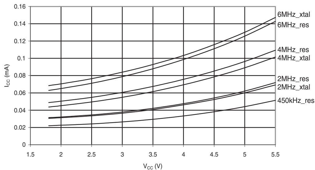
Figure 30-14. ATmega48A: Standby Supply Current vs. V_{CC} (Watchdog Timer Disabled)
