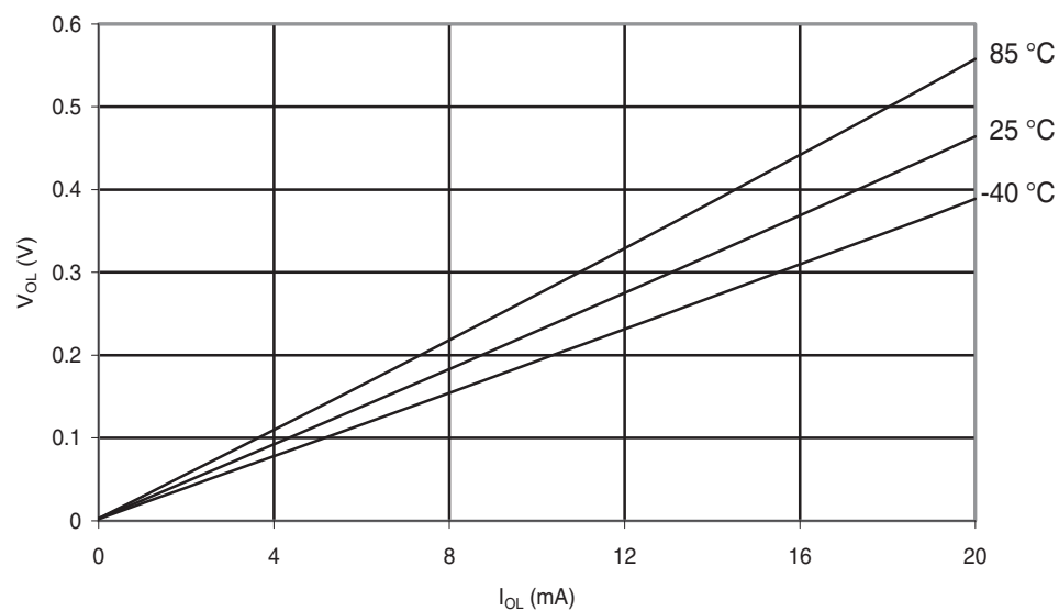
Figure 30-163. ATmega88PA: I/O Pin Output Voltage vs. Sink Current ( V_{CC} = 5\text{ V} )
