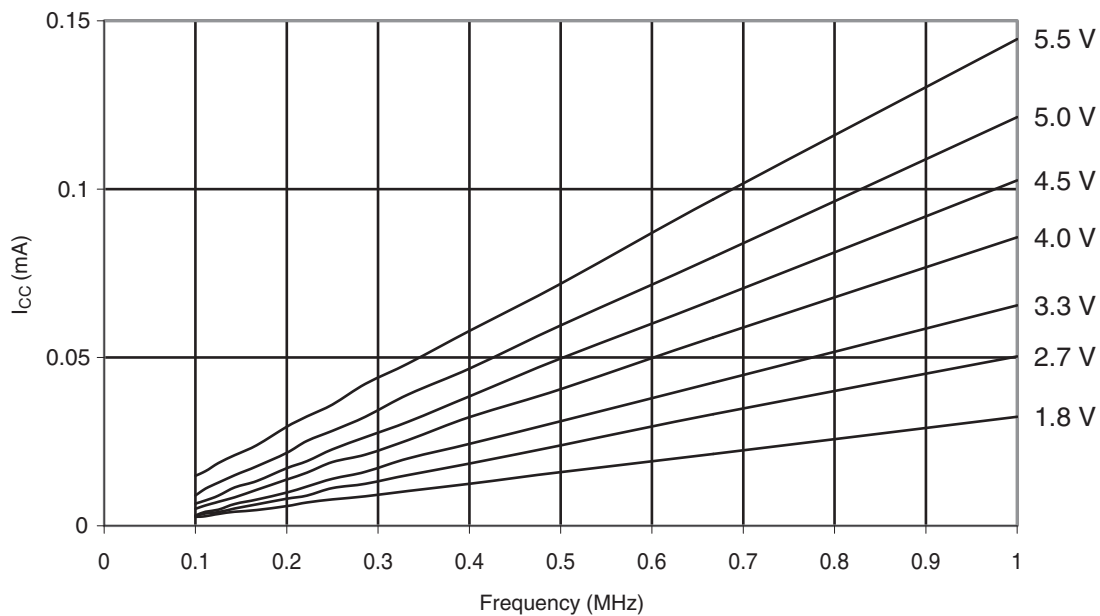
Figure 30-327. ATmega328: Reset Supply Current vs. Low Frequency (0.1 - 1.0MHz)
