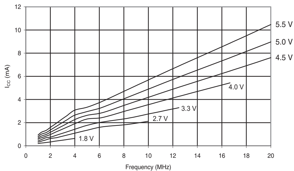
Figure 30-143. ATmega88PA: Active Supply Current vs. Frequency (1 - 20MHz)
