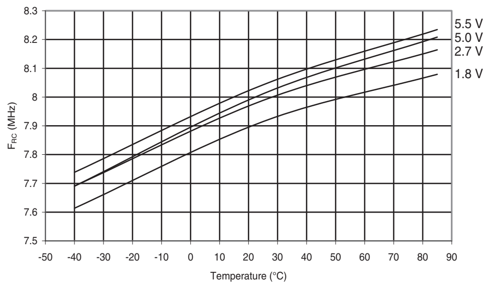
Figure 30-273. ATmega168PA: Calibrated 8MHz RC Oscillator Frequency vs. Temperature
