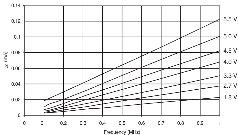
Figure 30-45. ATmega48A: Reset Supply Current vs. Low Frequency (0.1 - 1.0MHz)
