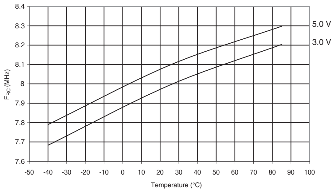
Figure 30-320. ATmega328: Calibrated 8MHz RC Oscillator Frequency vs. Temperature
