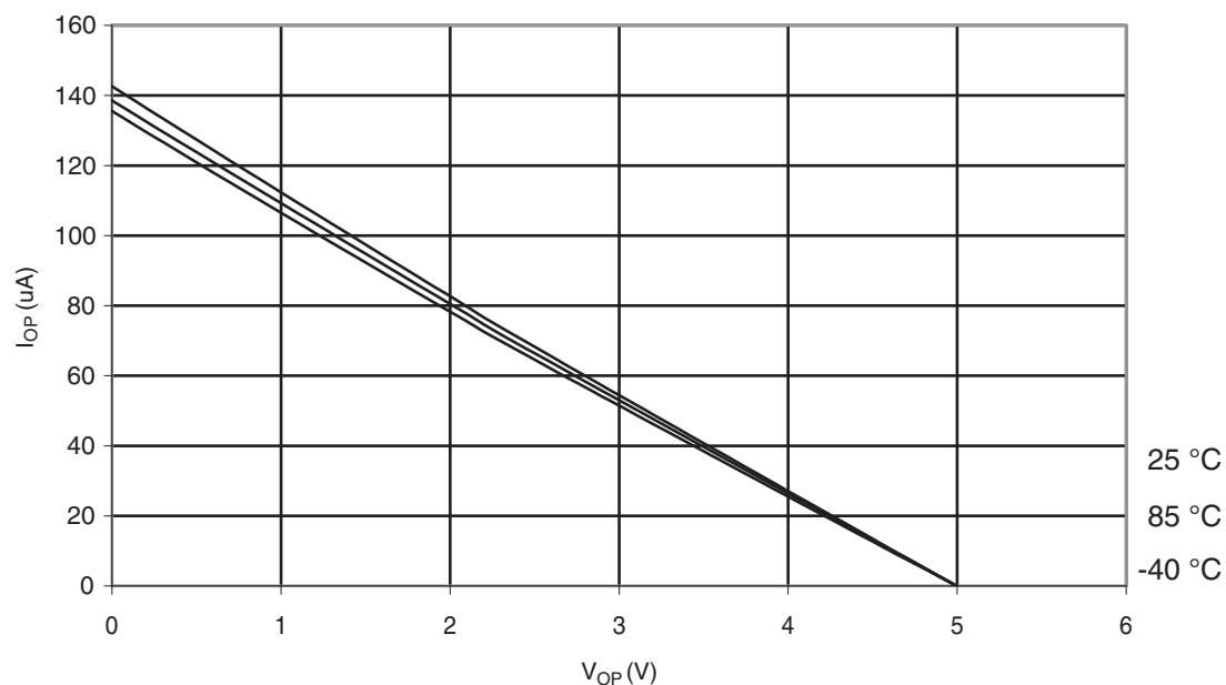
Figure 30-346. ATmega328P: I/O Pin Pull-up Resistor Current vs. Input Voltage ( V_{CC} = 5\text{ V} )
