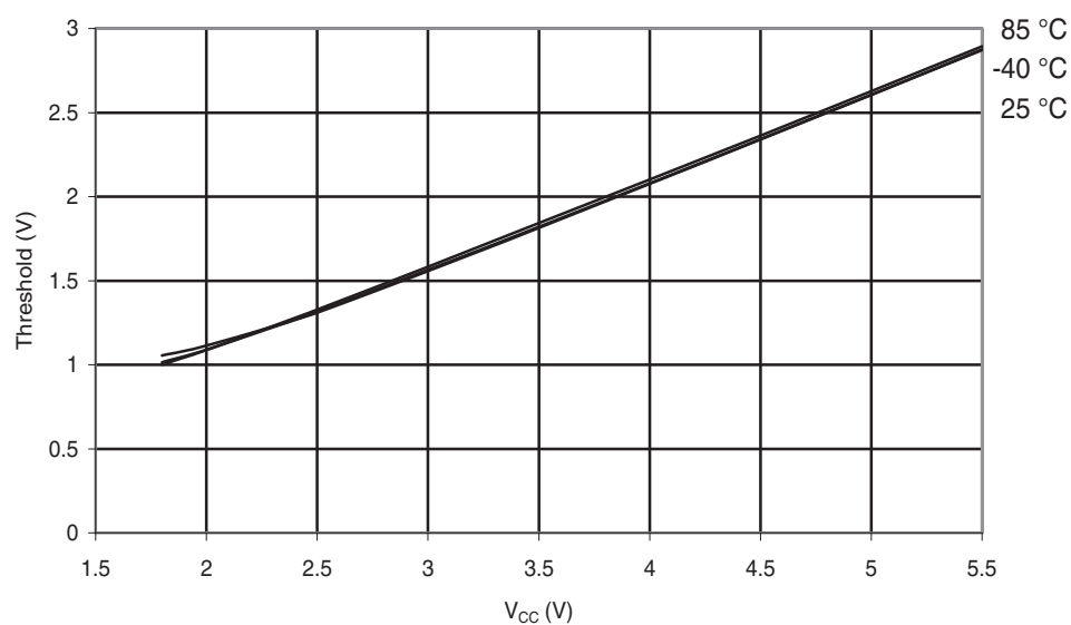
Figure 30-166. ATmega88PA: I/O Pin Input Threshold Voltage vs. V_{CC} ( V_{IH} , I/O Pin read as '1')
