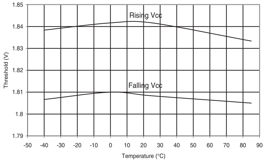
Figure 30-31. ATmega48A: BOD Thresholds vs. Temperature (BODLEVEL is 1.8 V)
