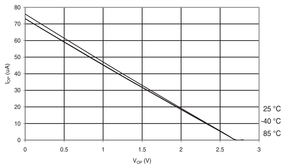
Figure 30-204.ATmega168A: I/O Pin Pull-up Resistor Current vs. Input Voltage ( V_{CC} = 2.7\text{ V} )
