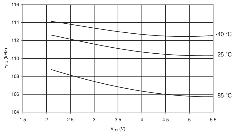
Figure 30-130.ATmega88A: Watchdog Oscillator Frequency vs. V CC
