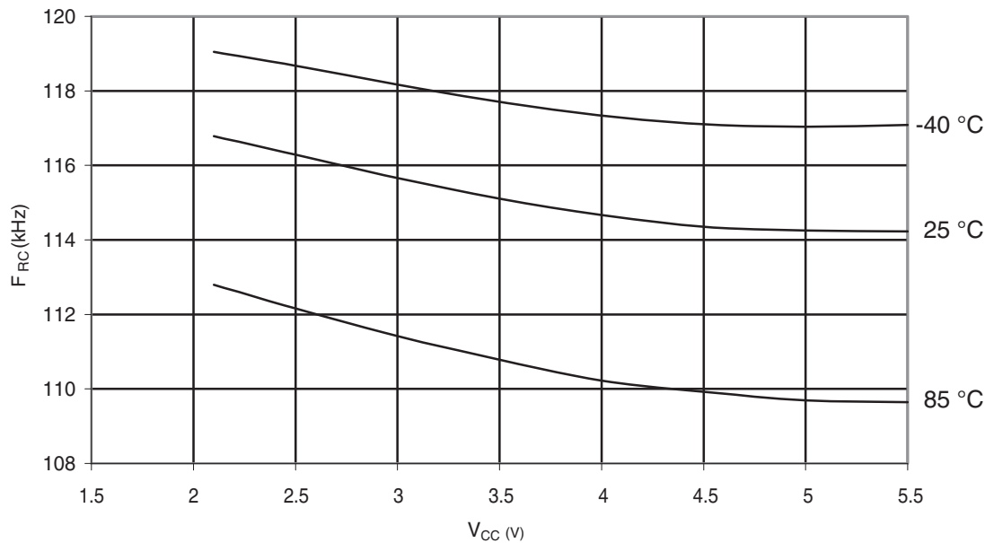
Figure 30-365. ATmega328P: Watchdog Oscillator Frequency vs. V_{CC}
