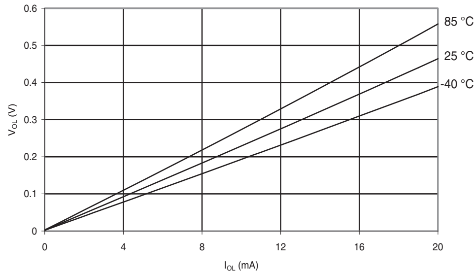
Figure 30-116. ATmega88A: I/O Pin Output Voltage vs. Sink Current ( V_{CC} = 5\text{ V} )
