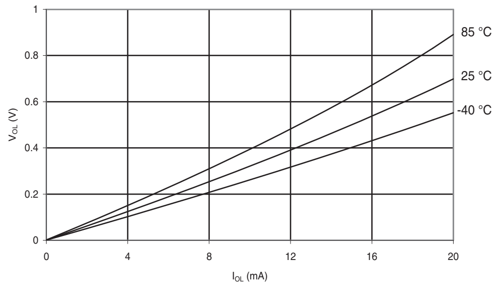
Figure 30-68. ATmega48PA: I/O Pin Output Voltage vs. Sink Current ( V_{CC} = 3\text{ V} )
