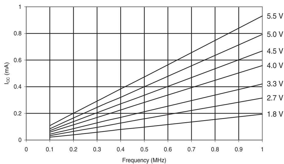
Figure 30-95. ATmega88A: Active Supply Current vs. Low Frequency (0.1-1.0MHz)
