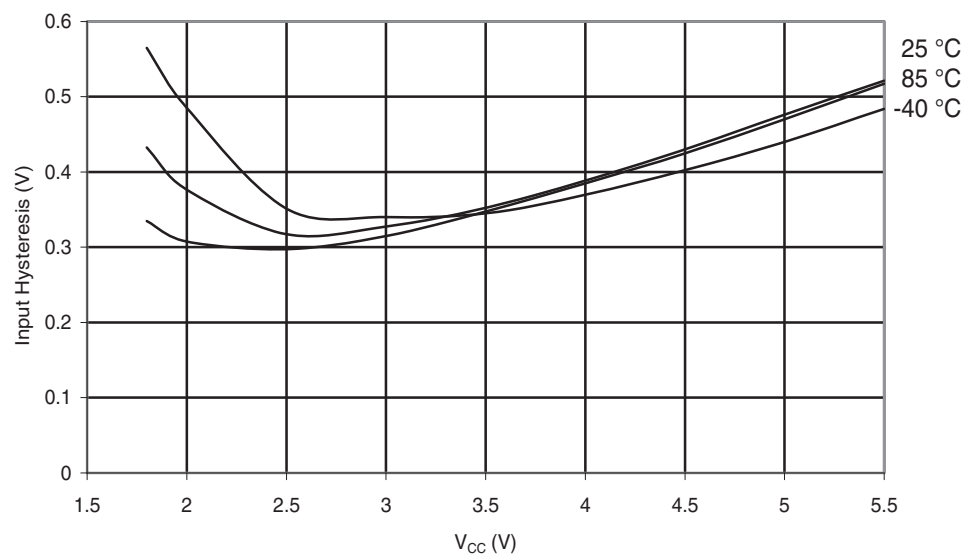
Figure 30-168. ATmega88PA: I/O Pin Input Hysteresis vs. V_{CC}
