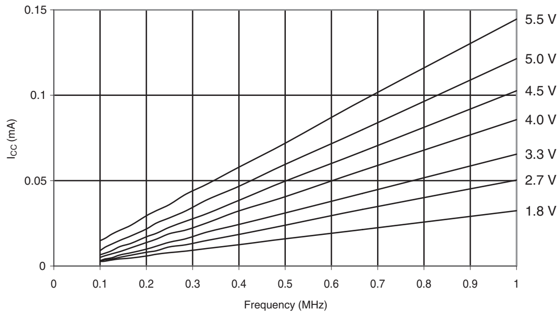
Figure 30-374. ATmega328P: Reset Supply Current vs. Low Frequency (0.1 - 1.0MHz)
