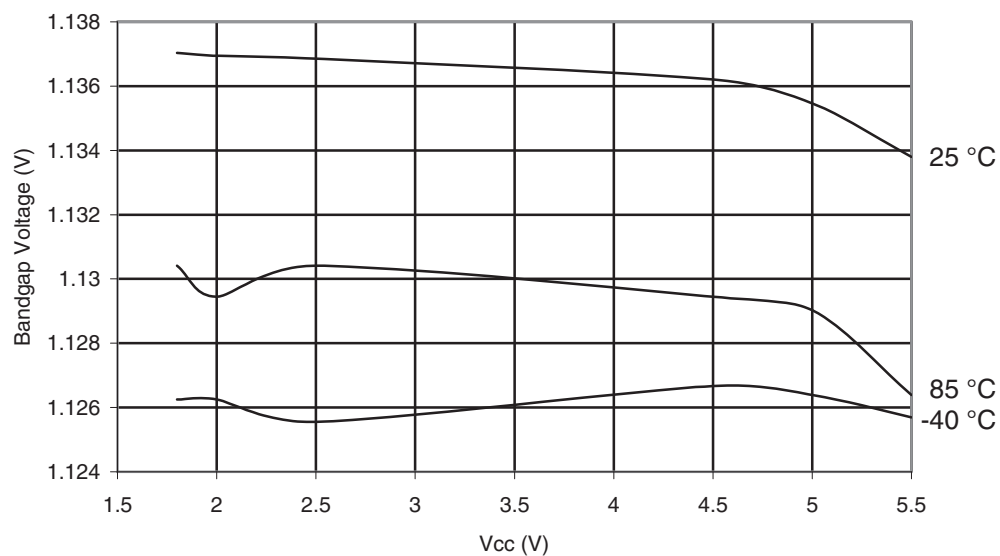
Figure 30-316. ATmega328: Bandgap Voltage vs. V_{CC}
