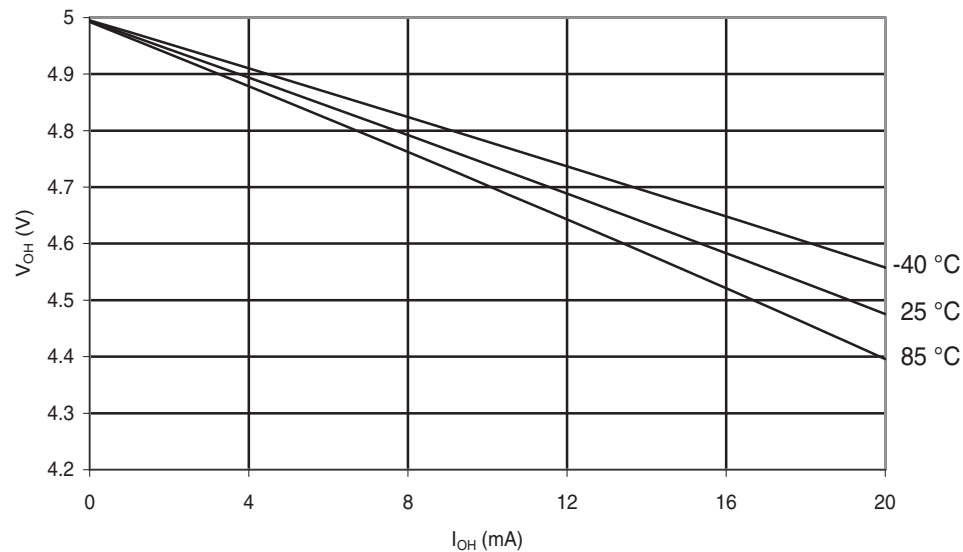
Figure 30-118.) ATmega88A: I/O Pin Output Voltage vs. Source Current ( V_{CC} = 5\text{ V} )
