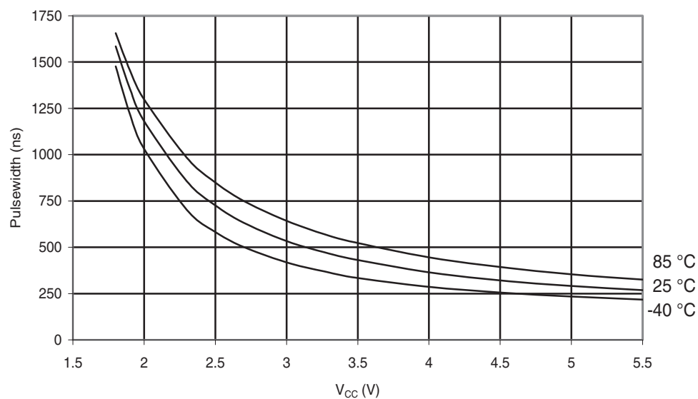
Figure 30-235. ATmega168A: Minimum Reset Pulse width vs. V_{CC}
