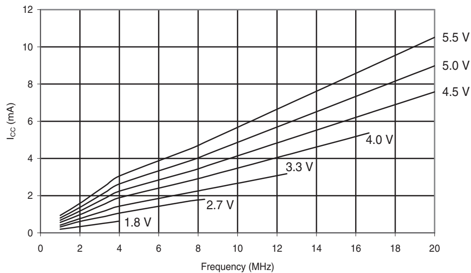
Figure 30-49. ATmega48PA: Active Supply Current vs. Frequency (1-20MHz)
