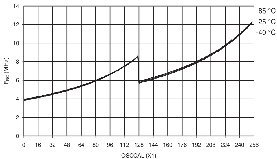
Figure 30-133. ATmega88A: Calibrated 8MHz RC Oscillator Frequency vs. OSCCAL Value
