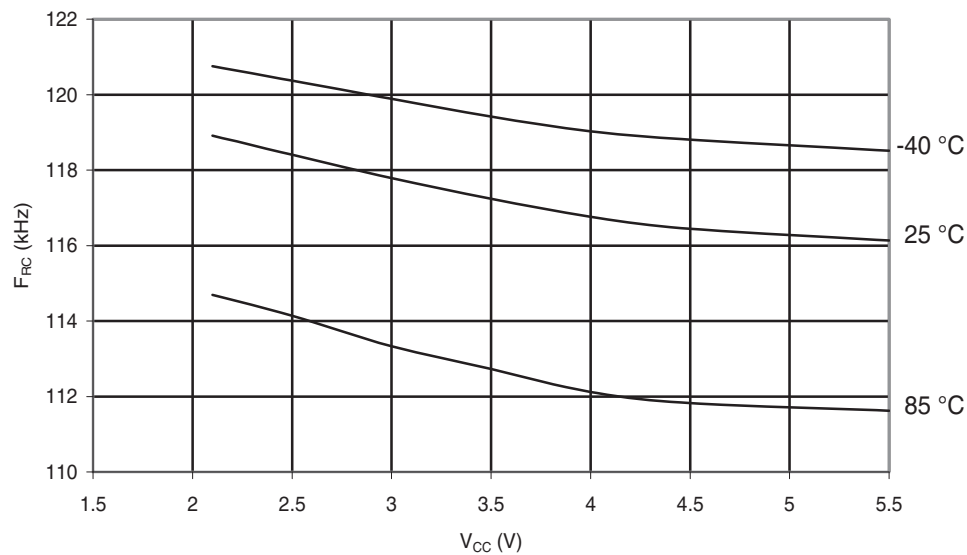
Figure 30-224.ATmega168A: Watchdog Oscillator Frequency vs. V CC
