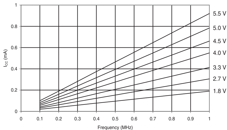
Figure 30-189. ATmega168A: Active Supply Current vs. Low Frequency (0.1-1.0MHz)
