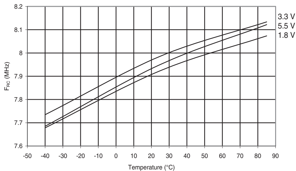
Figure 30-85. ATmega48PA: Calibrated 8MHz RC Oscillator Frequency vs. Temperature
