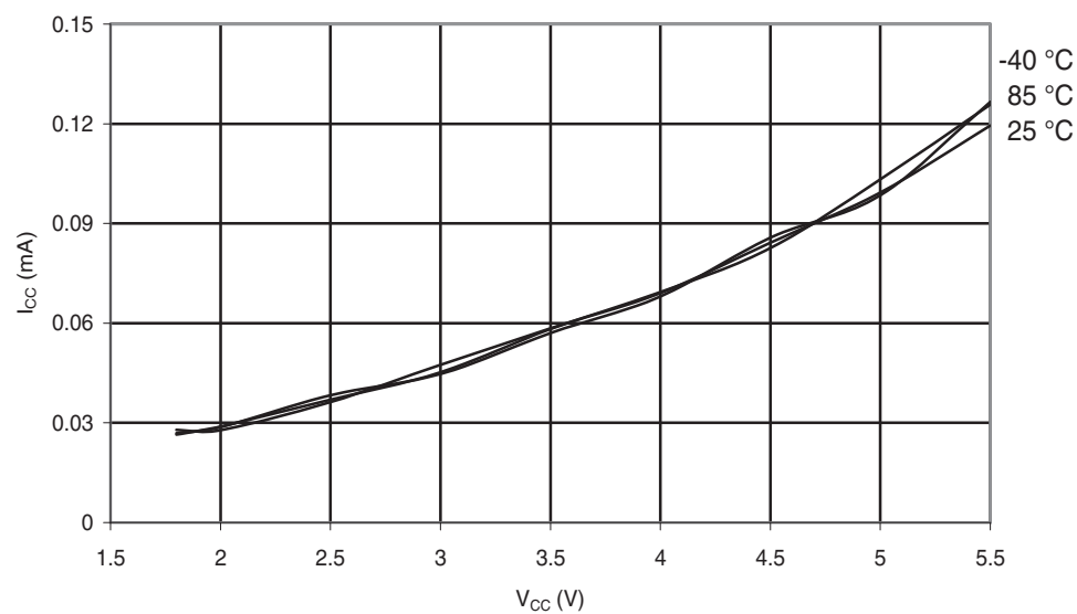
Figure 30-191. ATmega168A: Active Supply Current vs. V_{CC} (Internal RC Oscillator, 128kHz)
