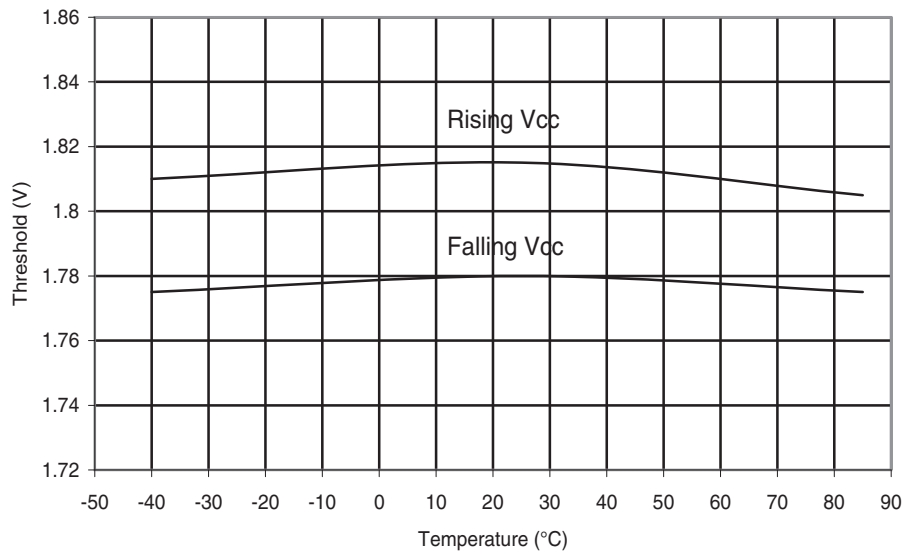
Figure 30-219.ATmega168A: BOD Thresholds vs. Temperature (BODLEVEL is 1.8 V)
