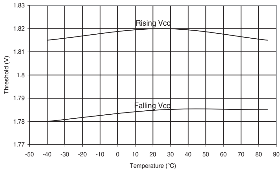
Figure 30-125.ATmega88A: BOD Thresholds vs. Temperature (BODLEVEL is 1.8 V)
