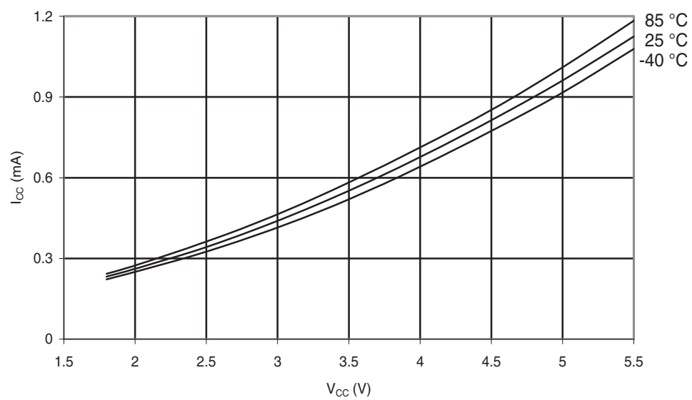
Figure 30-245. ATmega168PA: Idle Supply Current vs. V_{CC} (Internal RC Oscillator, 8MHz)
