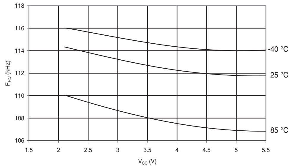
Figure 30-83. ATmega48PA: Watchdog Oscillator Frequency vs. V_{CC}
