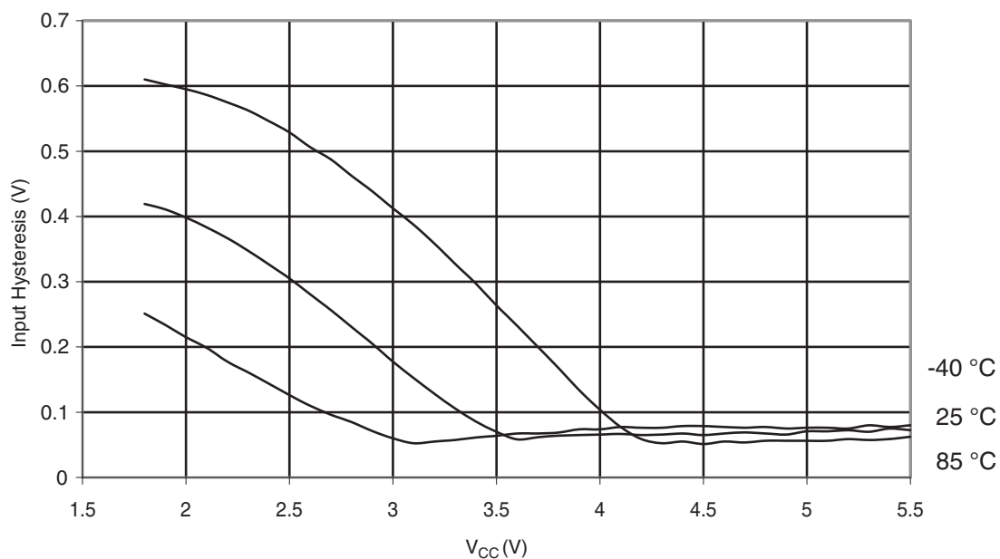
Figure 30-312. ATmega328: Reset Pin Input Hysteresis vs. V_{CC}
