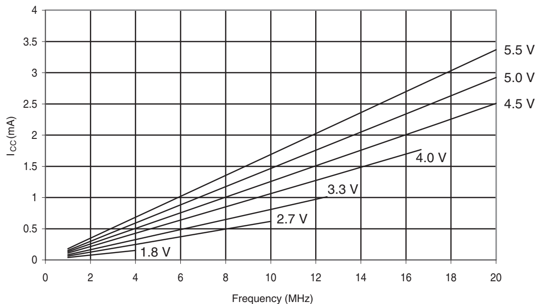
Figure 30-336. ATmega328P: Idle Supply Current vs. Frequency (1-20MHz)
