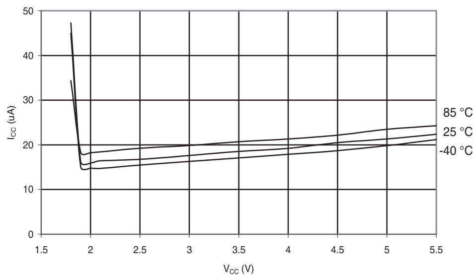
Figure 30-137. ATmega88A: Brownout Detector Current vs. V_{CC}
