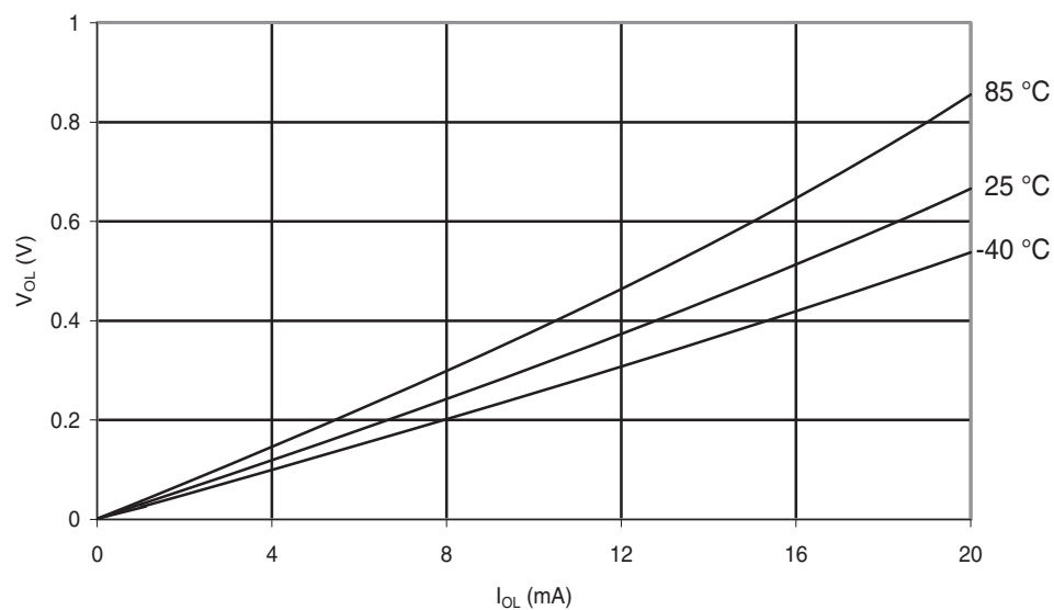
Figure 30-209. ATmega168A: I/O Pin Output Voltage vs. Sink Current ( V_{CC} = 3\text{ V} )
