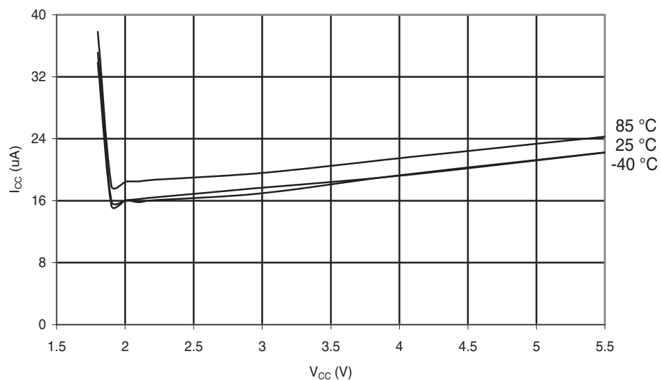
Figure 30-90. ATmega48PA: Brownout Detector Current vs. V_{CC}
