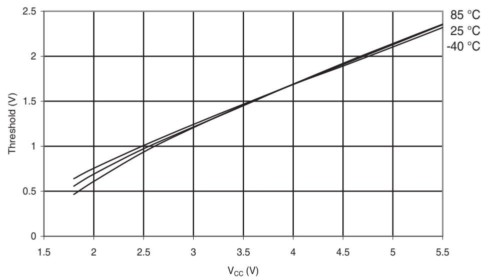
Figure 30-26. ATmega48A: I/O Pin Input Threshold Voltage vs. V_{CC} ( V_{IL} , I/O Pin read as '0')
