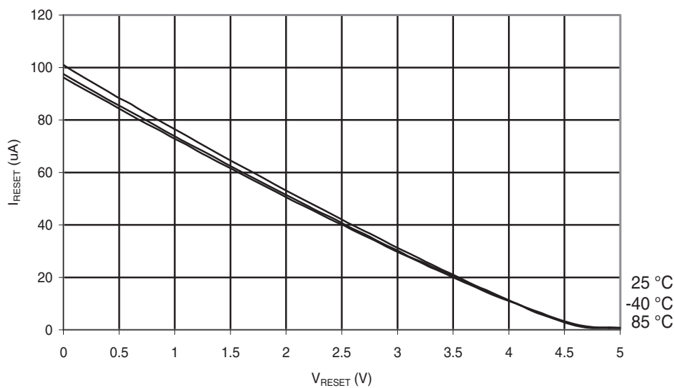
Figure 30-67. ATmega48PA: Reset Pull-up Resistor Current vs. Reset Pin Voltage ( V_{CC} = 5\text{ V} )
