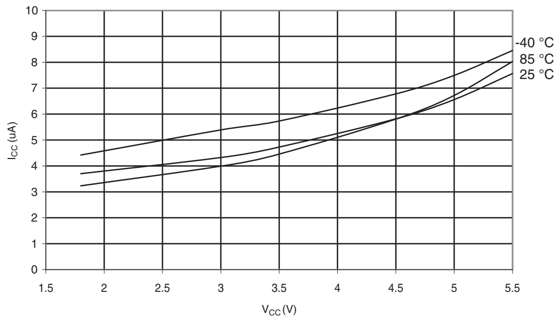
Figure 30-341. ATmega328P: Power-Down Supply Current vs. V_{CC} (Watchdog Timer Enabled)
