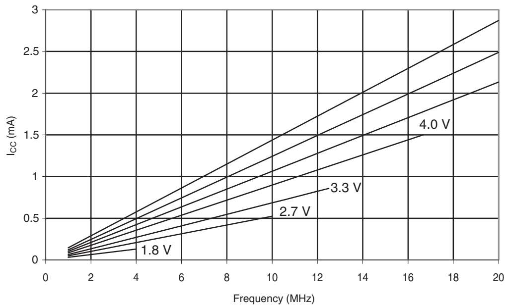
Figure 30-375. ATmega328P: Reset Supply Current vs. Frequency (1 - 20MHz)
