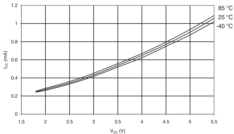
Figure 30-239. ATmega168PA: Active Supply Current vs. V_{CC} (Internal RC Oscillator, 1MHz)
