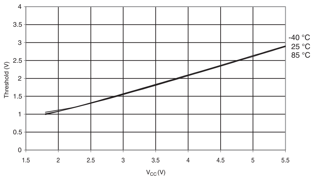
Figure 30-354. ATmega328P: I/O Pin Input Threshold Voltage vs. V_{CC} ( V_{IH} , I/O Pin read as '1')
