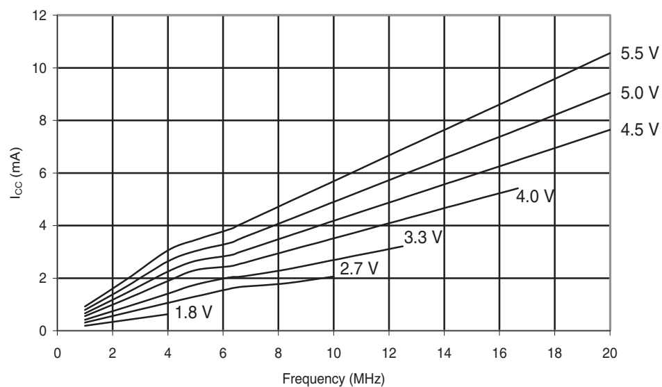
Figure 30-237. ATmega168PA: Active Supply Current vs. Frequency (1-20MHz)
