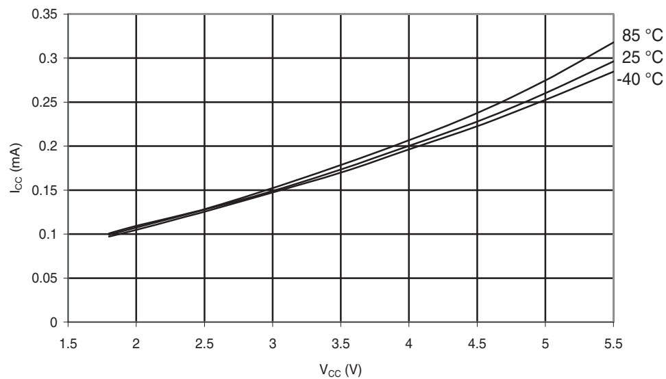
Figure 30-150. ATmega88PA: Idle Supply Current vs. V_{CC} (Internal RC Oscillator, 1MHz)
