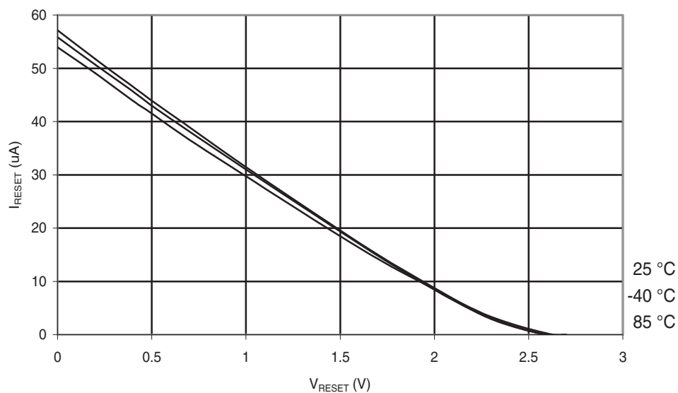
Figure 30-160. ATmega88PA: Reset Pull-up Resistor Current vs. Reset Pin Voltage ( V_{CC} = 2.7\text{ V} )
