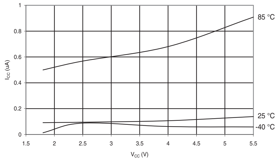
Figure 30-199.ATmega168A: Power-Down Supply Current vs. V CC (Watchdog Timer Disabled)
