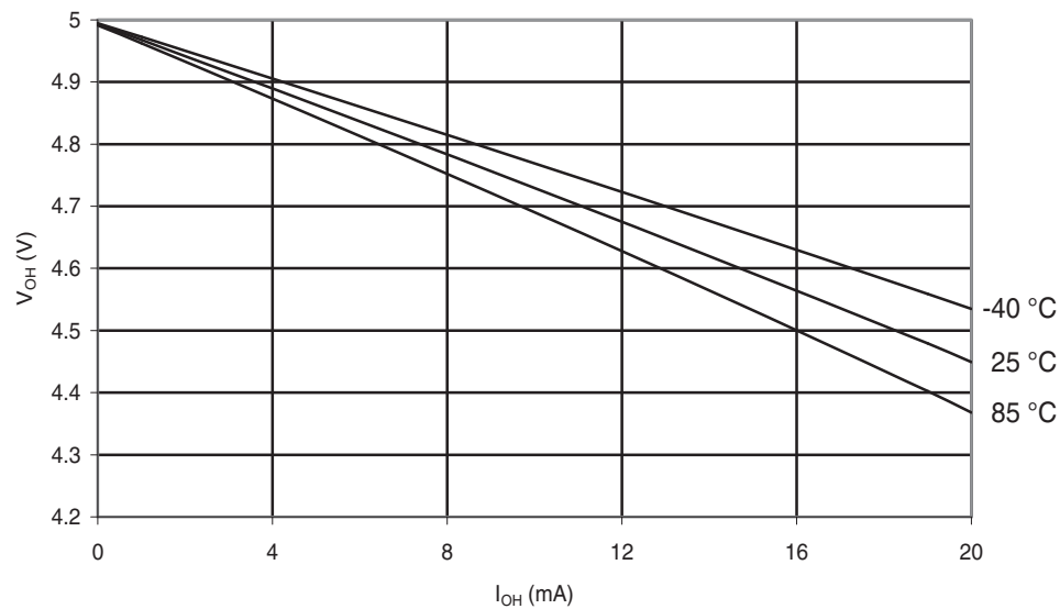
Figure 30-24. ATmega48A: I/O Pin Output Voltage vs. Source Current ( V_{CC} = 5\text{ V} )
