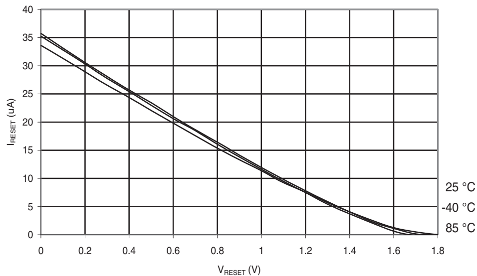
Figure 30-206. ATmega168A: Reset Pull-up Resistor Current vs. Reset Pin Voltage ( V_{CC} = 1.8\text{ V} )
