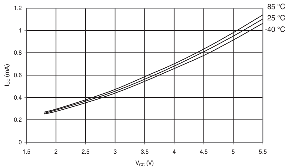
Figure 30-145. ATmega88PA: Active Supply Current vs. V_{CC} (Internal RC Oscillator, 1MHz)
