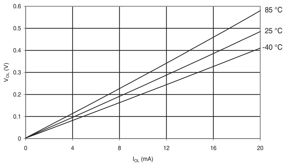
Figure 30-22. ATmega48A: I/O Pin Output Voltage vs. Sink Current ( V_{CC} = 5\text{ V} )
