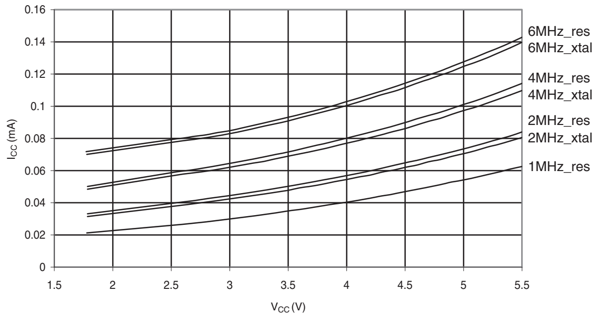
Figure 30-296. ATmega328: Standby Supply Current vs. V CC (Watchdog Timer Disabled)
