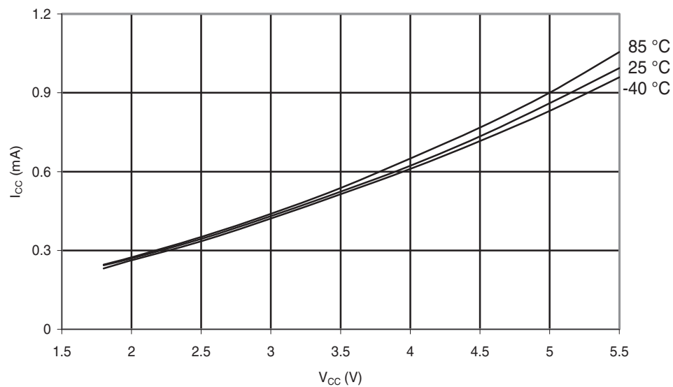
Figure 30-104. ATmega88A: Idle Supply Current vs. V CC (Internal RC Oscillator, 8MHz)
