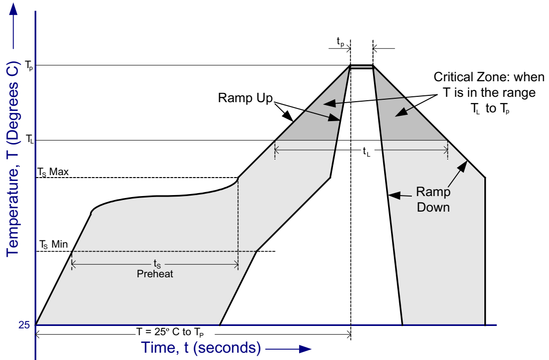
Figure 8 - FT232R Solder Reflow Profile
