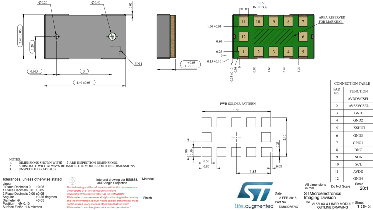
Figure 22. Outline drawing (1/3)
