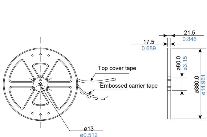
Dimensions of tape reel (Typ.)
