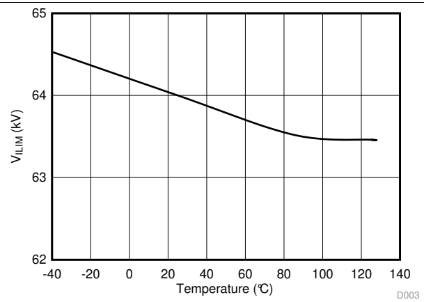
Figure 2. V_{ILIM} vs Temperature
