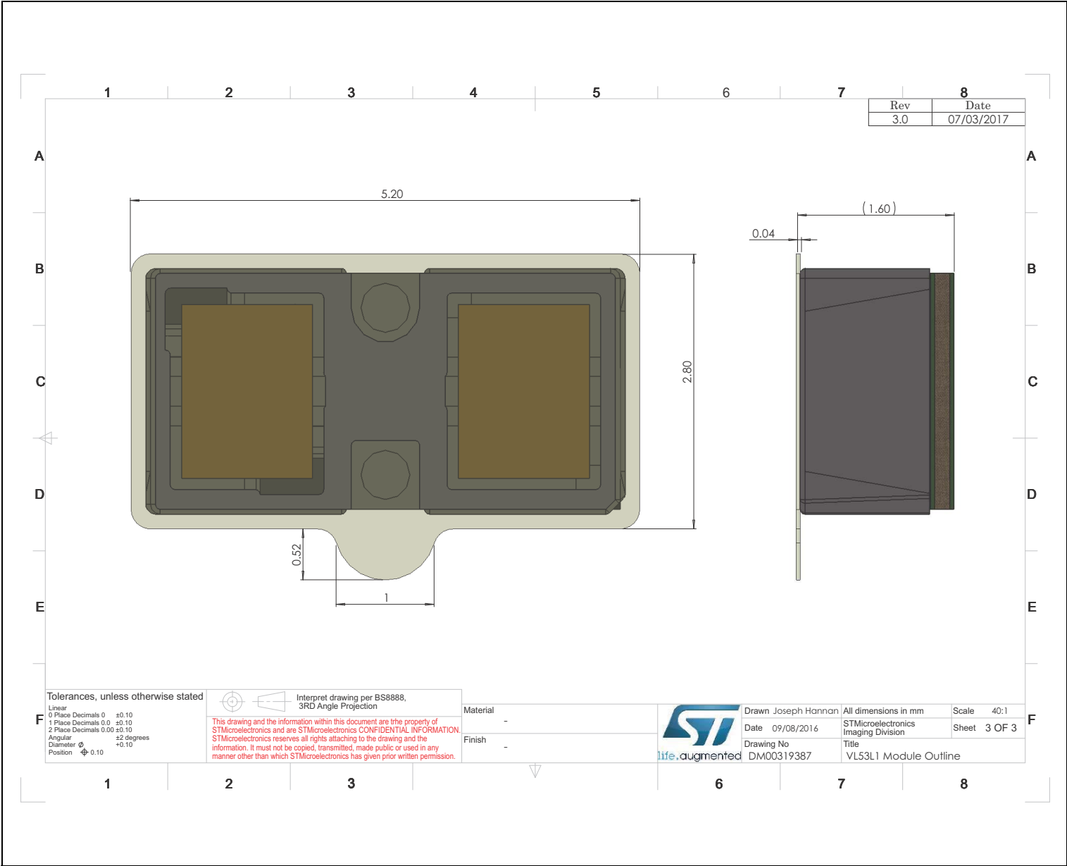
Figure 20. Outline drawing (page 3/3)
