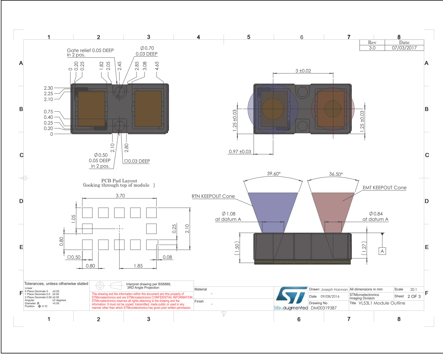
Figure 19. Outline drawing (page 2/3)
