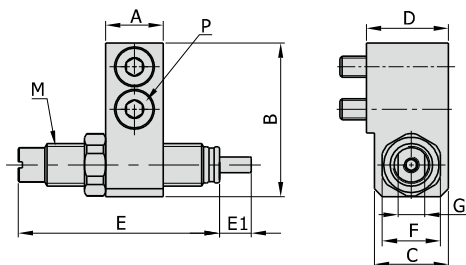
Body Mounting
