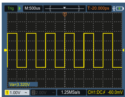
0-1. figure: Automatic setting
