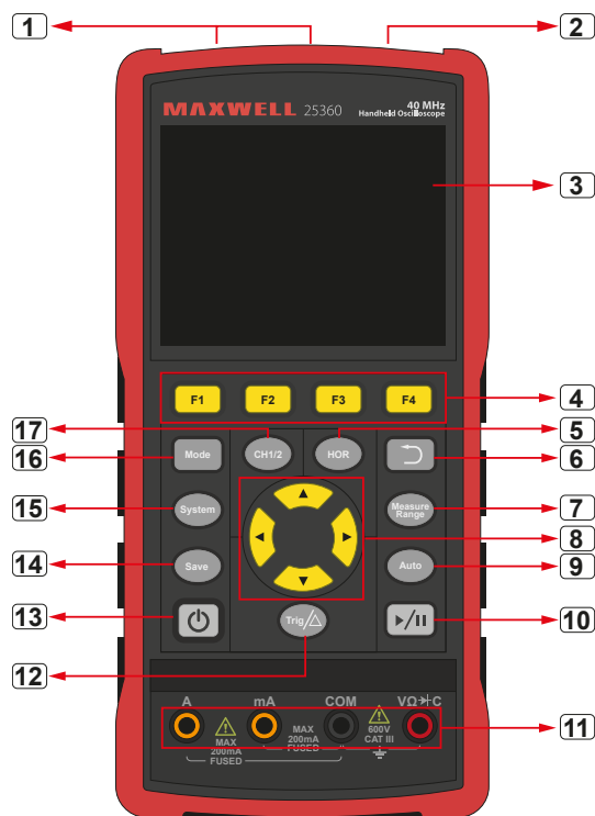
Oscilloscope front panel
