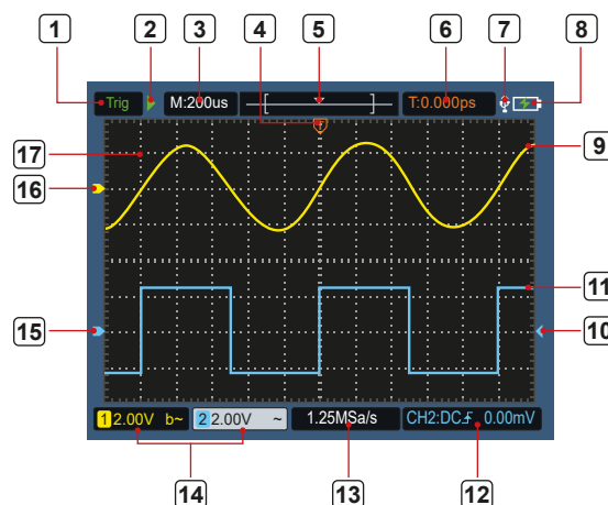
5. figure: Oscilloscope user interface
