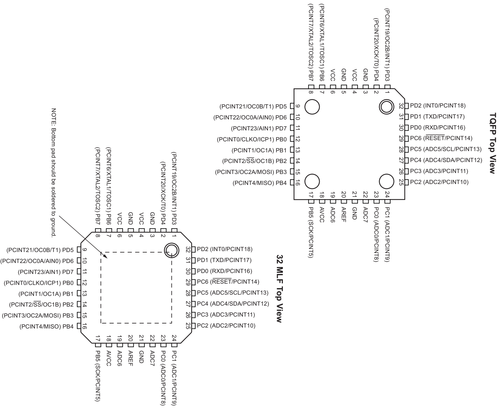
Figure 1-1. Pinout
