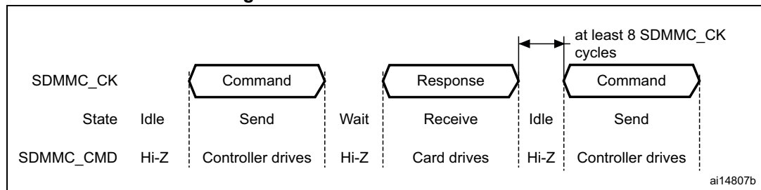
Figure 239. SDIO command transfer
