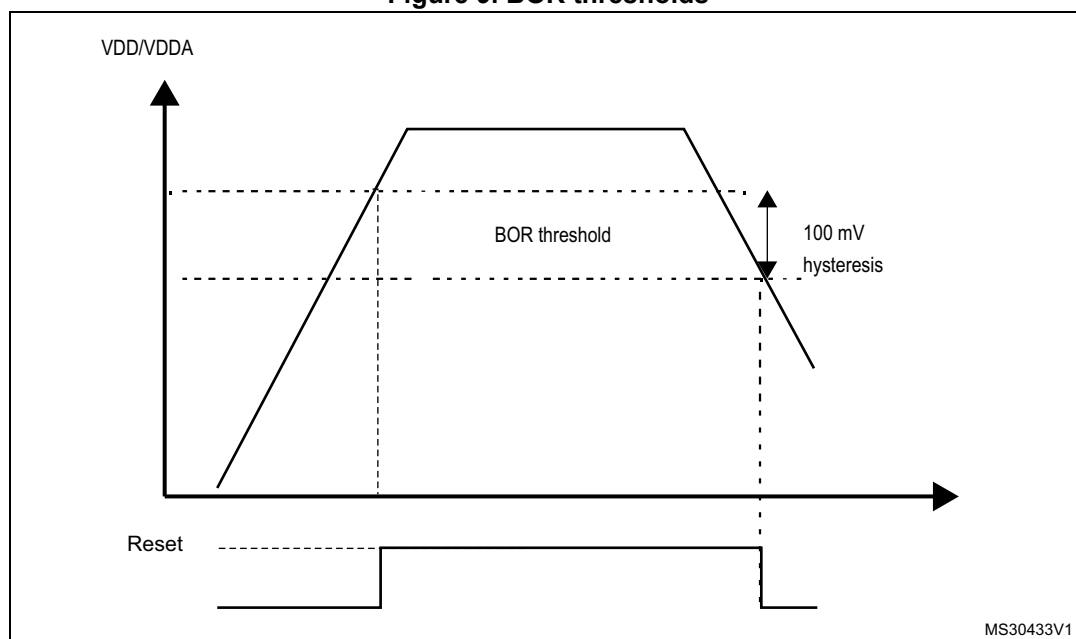
Figure 9. BOR thresholds
