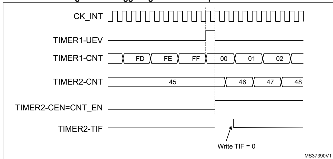
Figure 130. Triggering timer 2 with update of timer 1
