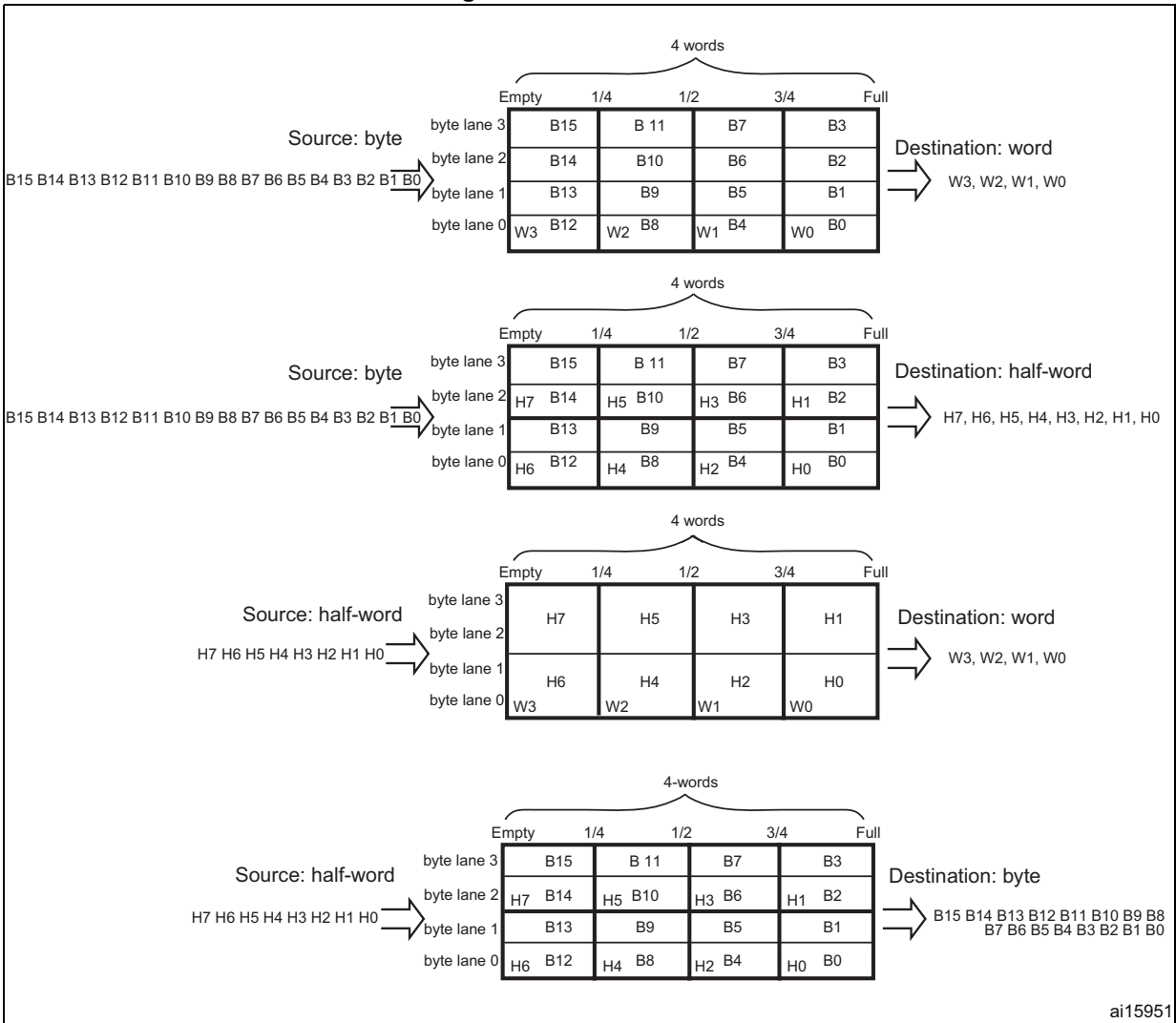
Figure 28. FIFO structure
