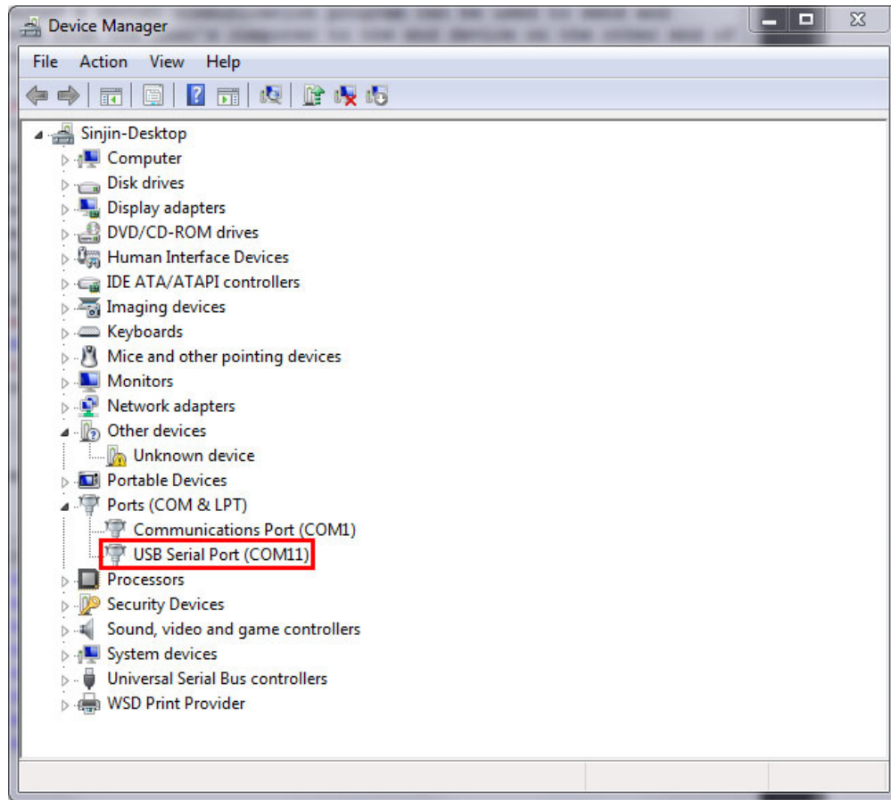
Figure 6: Device Manager
