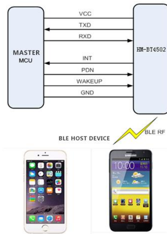
Figure 1. Application Schematic of the Pass-through Module
