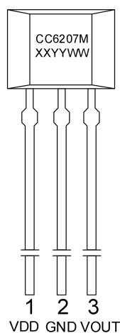
TO-92S package
