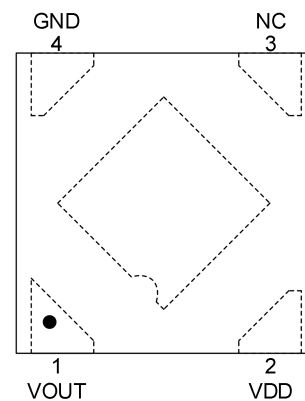
DFN4L package
