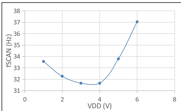
f_SCAN vs. VDD
