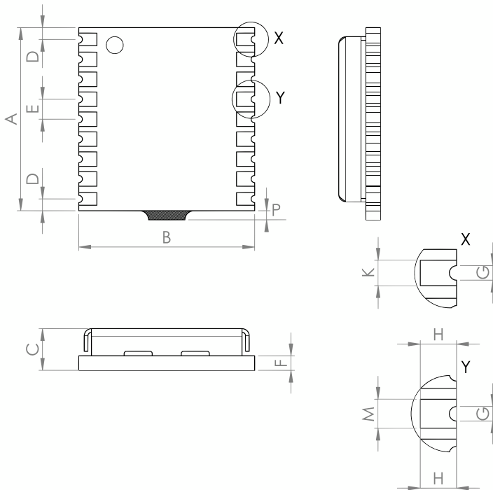
Figure 3: Mechanical drawing
