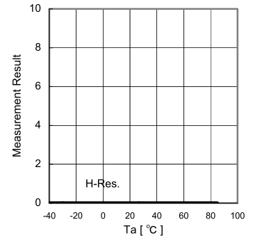
Fig.6 Dark Response
