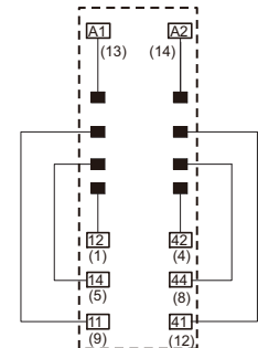
Terminal Arrangement/Internal Connection Diagram (Top View)
