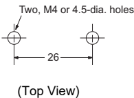
Mounting Hole Dimensions
