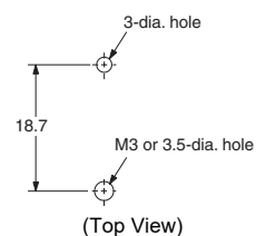
Mounting Hole Dimensions
