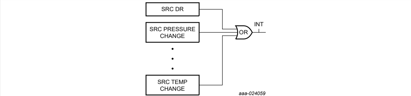
Figure 8. INT1/INT2 pin control logic
