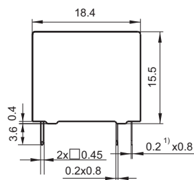
Outline Dimensions
