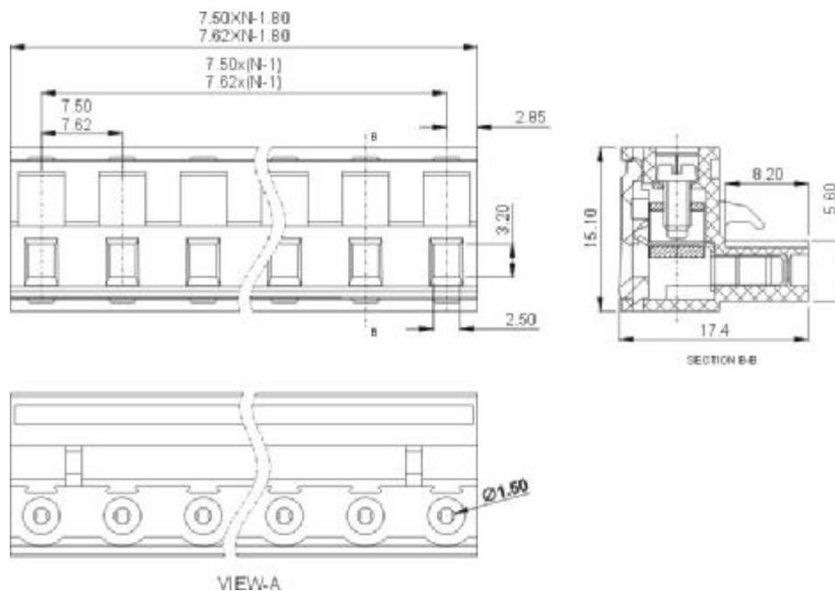
2EDGK-7.5 2EDGK-7.62
