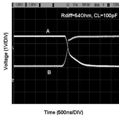
FIGURE 20. DRIVER WAVEFORMS
