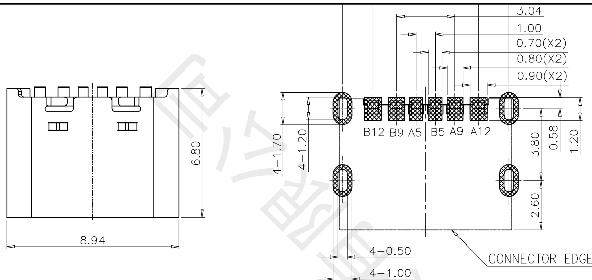
RECOMMENDED PCB LAYOUT(TOP VIEW) THICKNESS 1.6±0.1MM;DEFAULT TOLERANCE:±0.05
