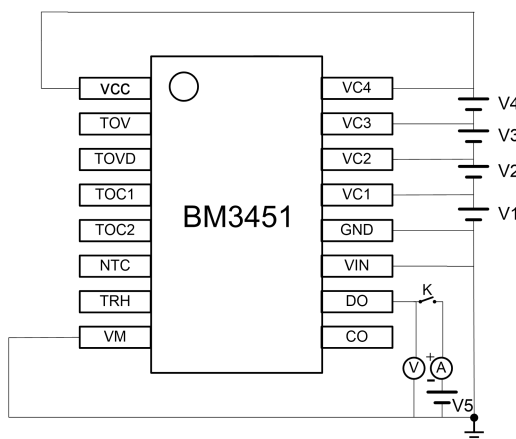
Test Circuit 6
