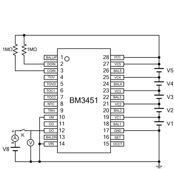
Test Circuit 7
