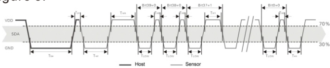
Figure 8 AM2120 Single bus communication timing
