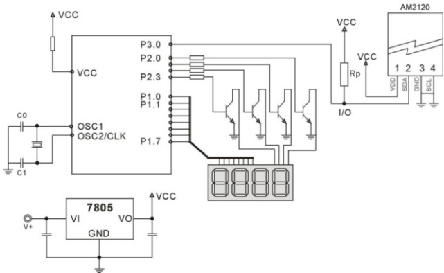
Figure 6 AM2120 One-wire bus application circuitry
