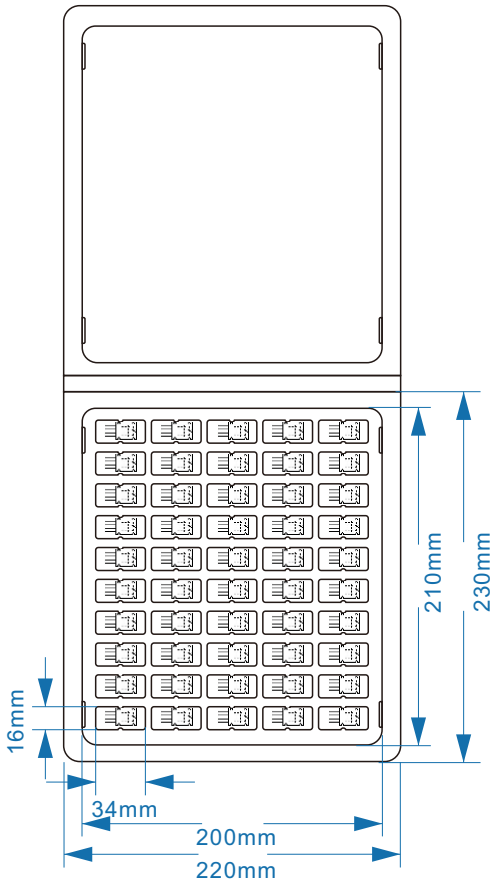
Figure14 Blister box and sensor location diagram
