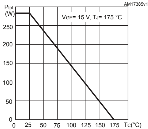
Figure 1. Power dissipation vs case temperature for TO-247
