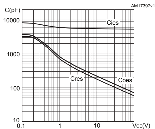
Figure 17. Capacitance variations
