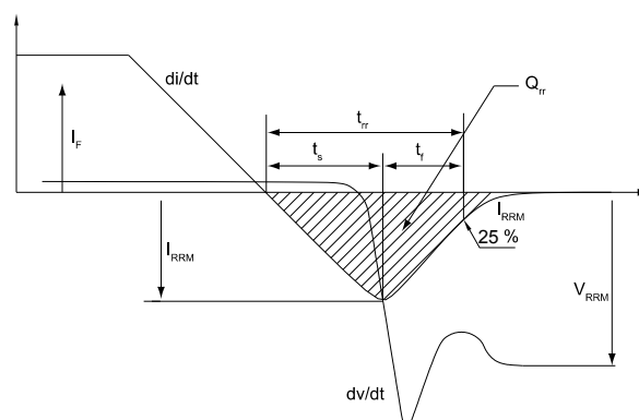
Figure 36. Diode reverse recovery waveform
