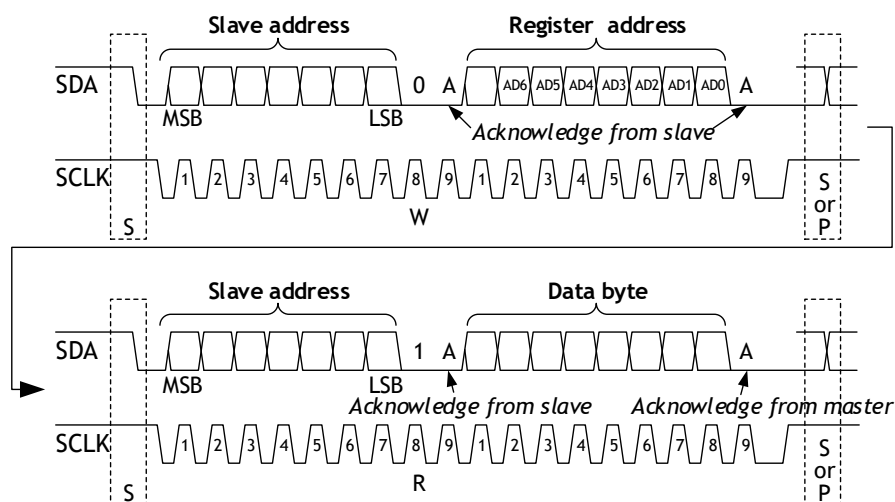
Figure 12: I 2 C Read Operation
