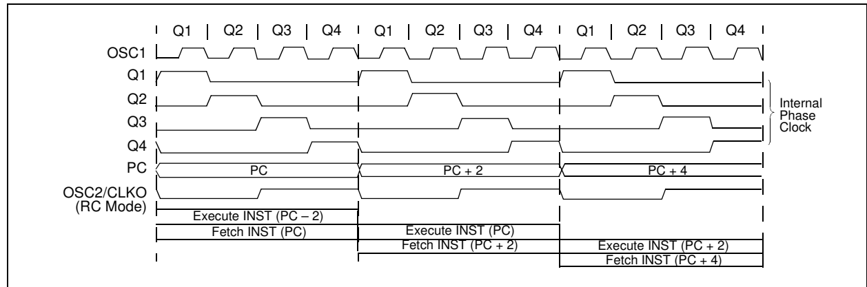
FIGURE 5-4: CLOCK/INSTRUCTION CYCLE
