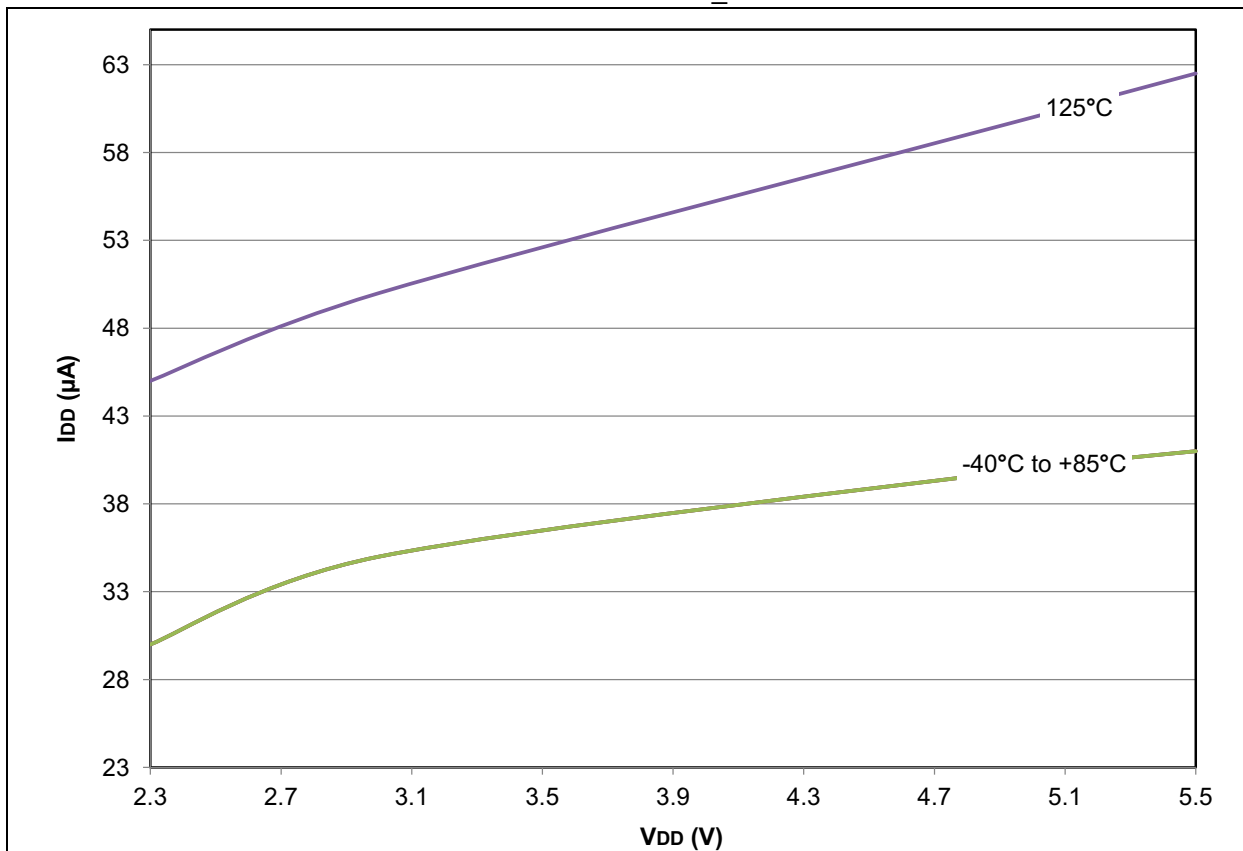
FIGURE 28-79: PIC18F2X/4XK22 MAXIMUM I_{DD} : SEC_IDLE 32.768 kHz
