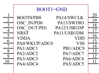
CH32V203F6P6
