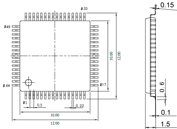
Figure 5-7 LQFP64M package
