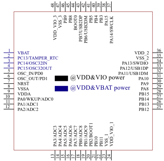
CH32V203CxT6
