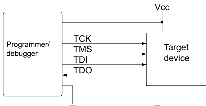
Figure 3-14. JTAG Interface Basics
