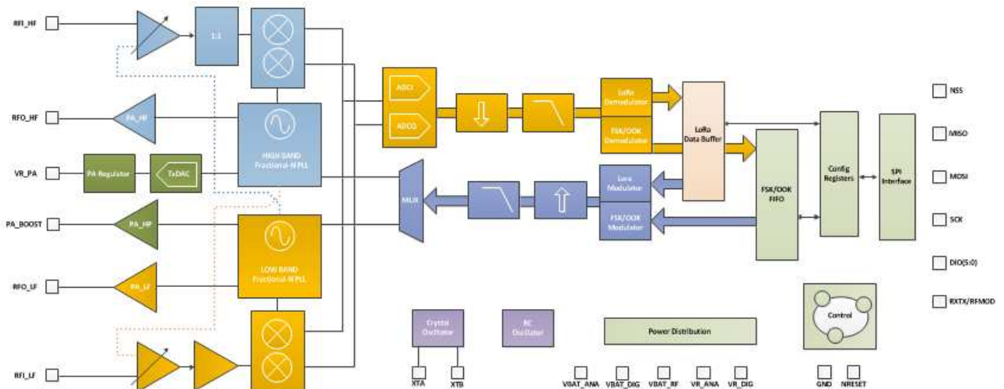
Figure 3. RF96/97/98 Block Schematic Diagram
