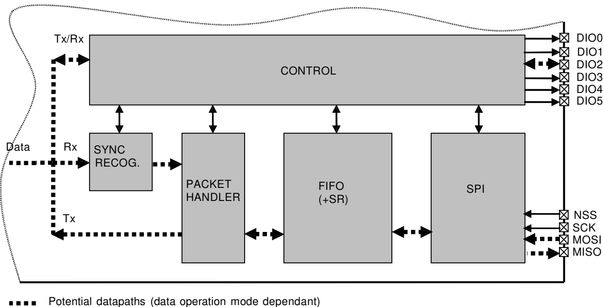
Figure 25. RF96/97/98 Data Processing Conceptual View
